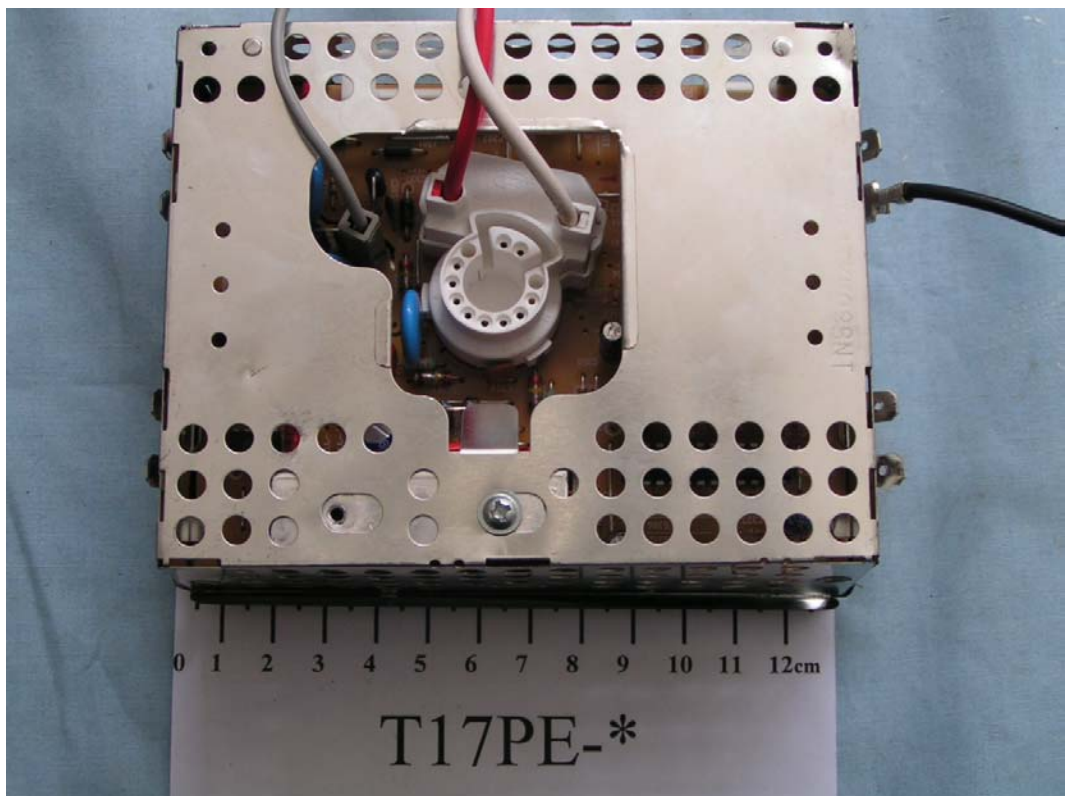
FIGURE 9 COLOR MONITOR (M/N: T17PE-*) CRT BOARD
