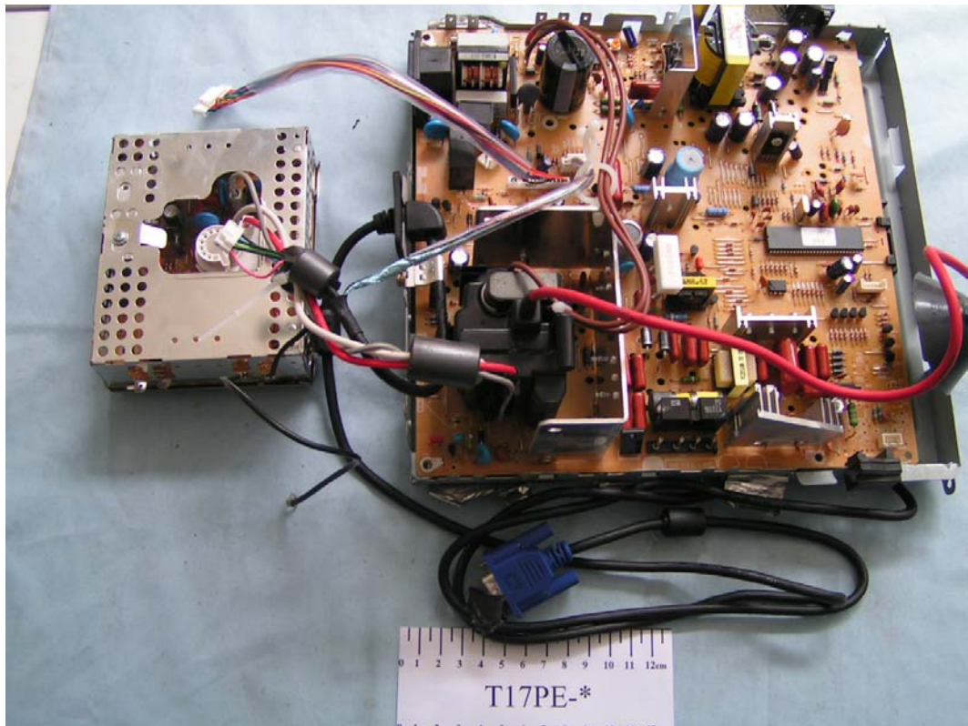
FIGURE 3 COLOR MONITOR (M/N: T17PE-*) MAIN BOARD & CRT BOARD
