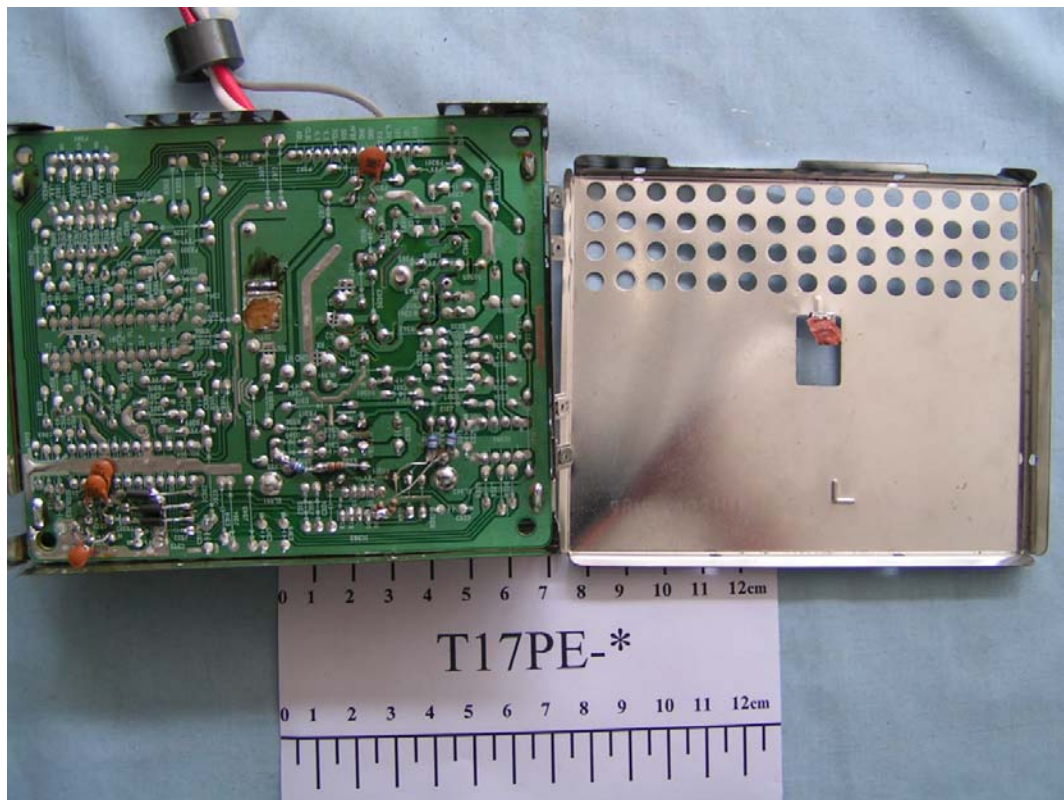
FIGURE 10 COLOR MONITOR (M/N: T17PE-*) CRT BOARD – SHELL REMOVED 1
