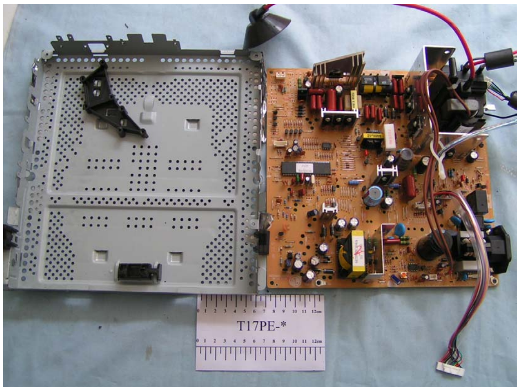
FIGURE 4 COLOR MONITOR (M/N: T17PE-*) MAIN BOARD-HOLDER REMOVED
