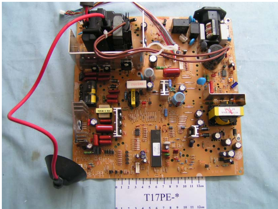
FIGURE 6 COLOR MONITOR (M/N: T17PE-*) MAIN BOARD (COMPONENT SIDE)
