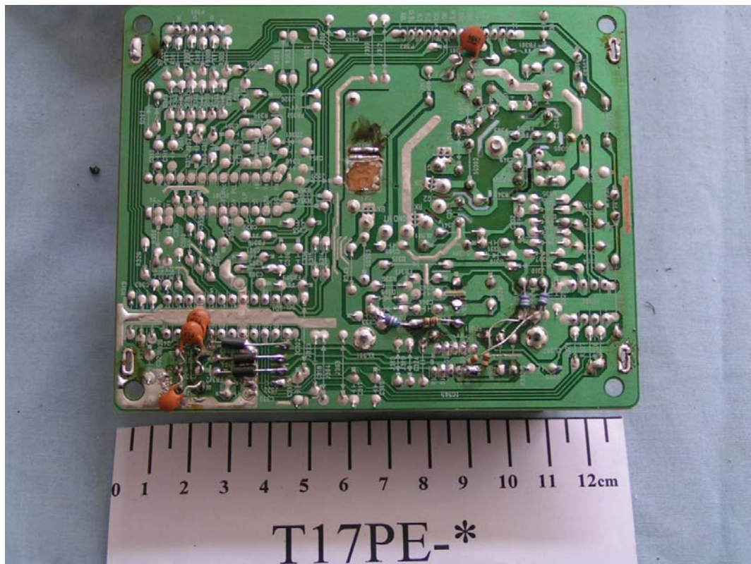
FIGURE 12 COLOR MONITOR (M/N: T17PE-*) CRT BOARD (SOLDERED SIDE)
