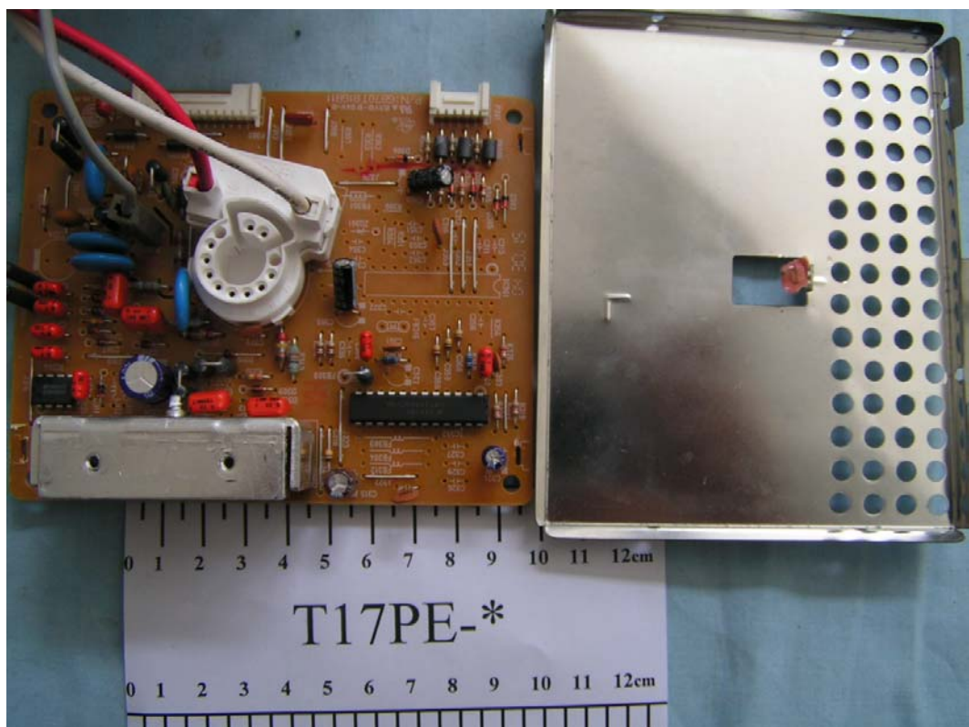
FIGURE 11 COLOR MONITOR (M/N: T17PE-*) CRT BOARD – SHELL REMOVED 2
