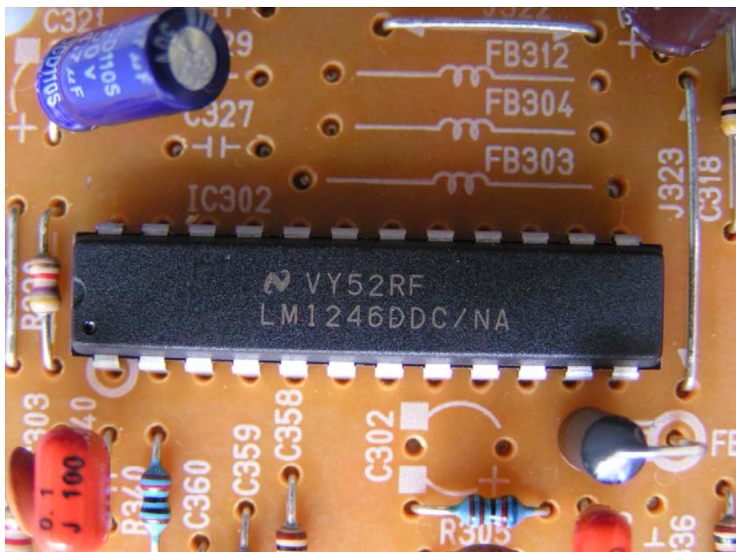
FIGURE 13 COLOR MONITOR (M/N: T17PE-*) CHIP ON THE CRT BOARD
