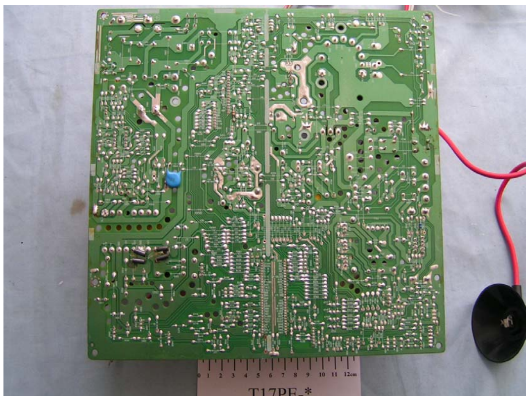
FIGURE 7 COLOR MONITOR (M/N: T17PE-*) MAIN BOARD (SOLDERED SIDE)
