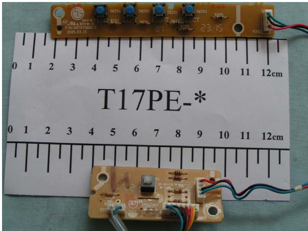
FIGURE 14 COLOR MONITOR (M/N: T17PE-*) BUTTON BOARD (FRONT VIEW)
