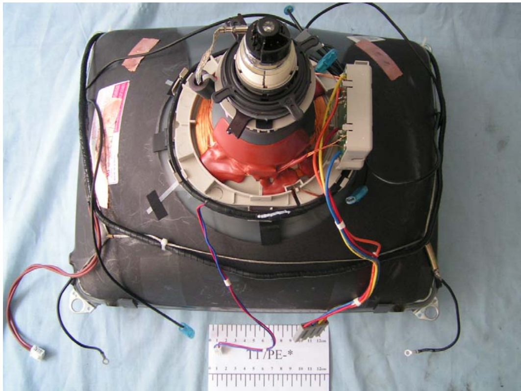
FIGURE 18 COLOR MONITOR (M/N: T17PE-*) CRT (REAR VIEW)
