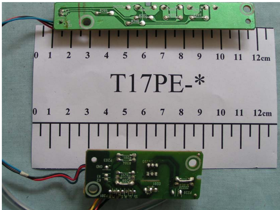
FIGURE 15 COLOR MONITOR (M/N: T17PE-*) BUTTON BOARD (REAR VIEW)
