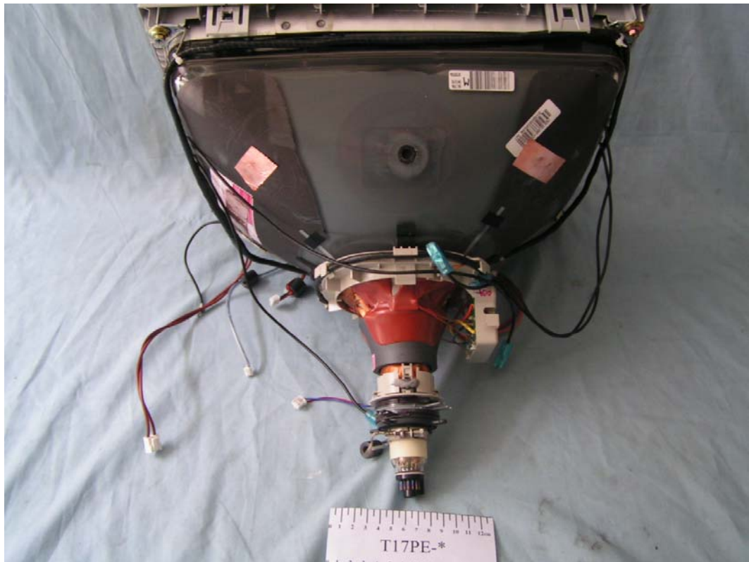
FIGURE 16 COLOR MONITOR (M/N: T17PE-*) CRT – ALL BOARD REMOVED
