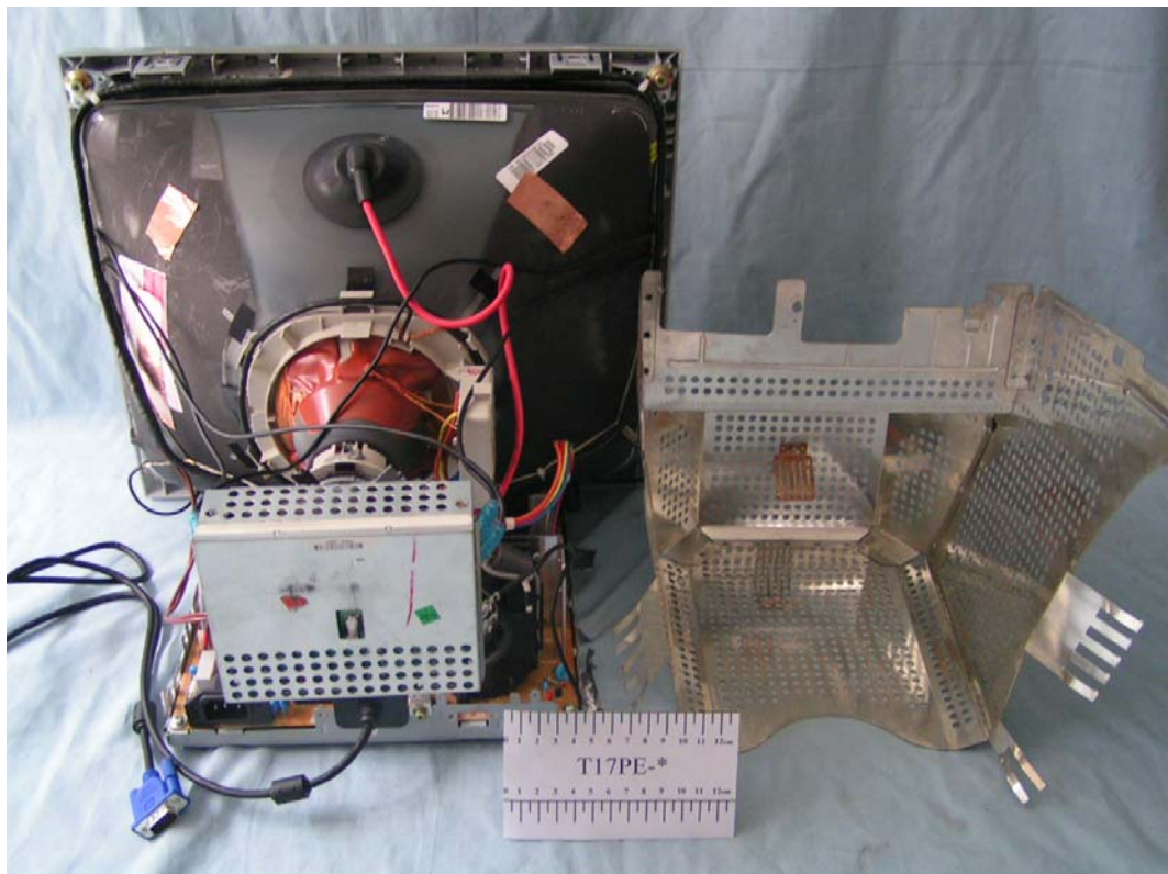
FIGURE 2 COLOR MONITOR (M/N: T17PE-*) SHIELDED SHELL REMOVED
