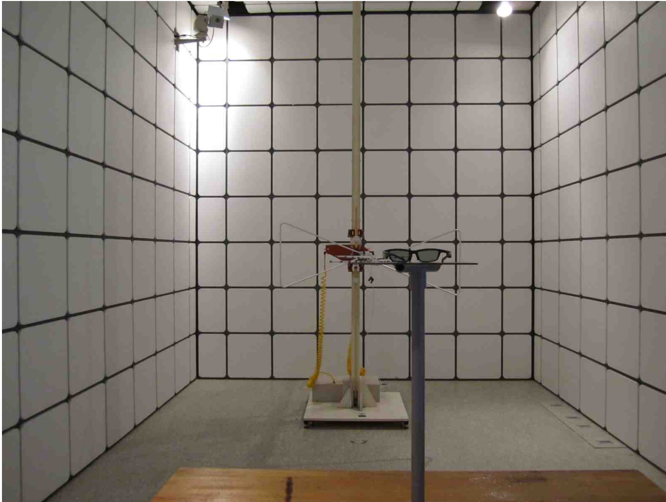
Radiated Test Setup below 1 GHz
