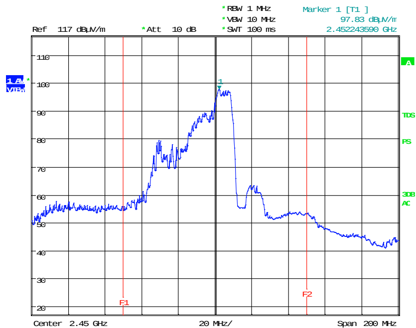
< Fig 10. Frequency Measurements (Minimum Frequency Observed: 2.452 GHz) >
