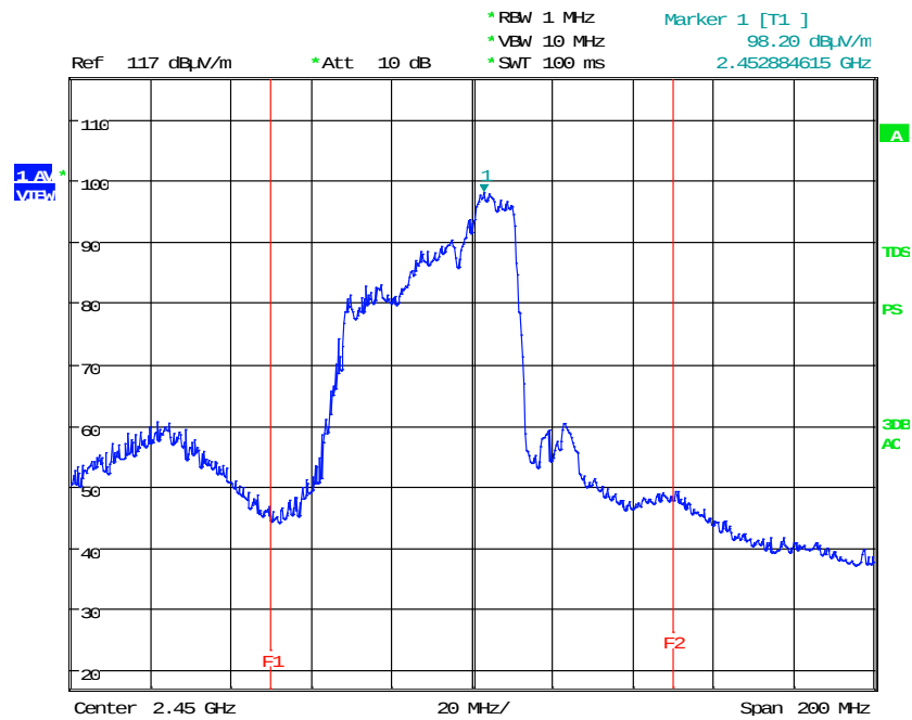
< Fig 9. Frequency Measurements (Maximum Frequency Observed: 2.452 GHz) >
