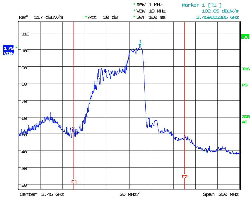
< Fig 8. Frequency Measurements (Minimum Frequency Observed: 2.459 GHz) >
