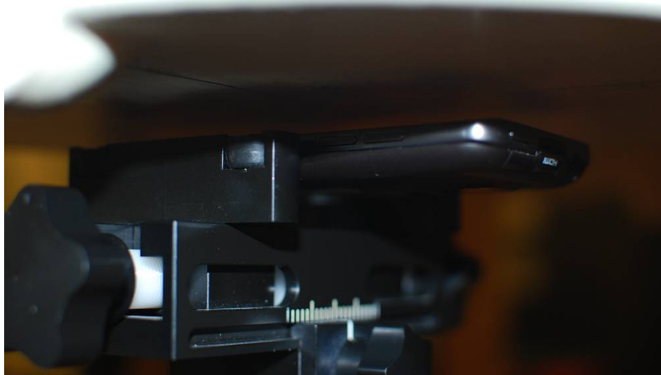
Figure 21-6 SAR Test Setup Photo 6: Front 1.0 cm
