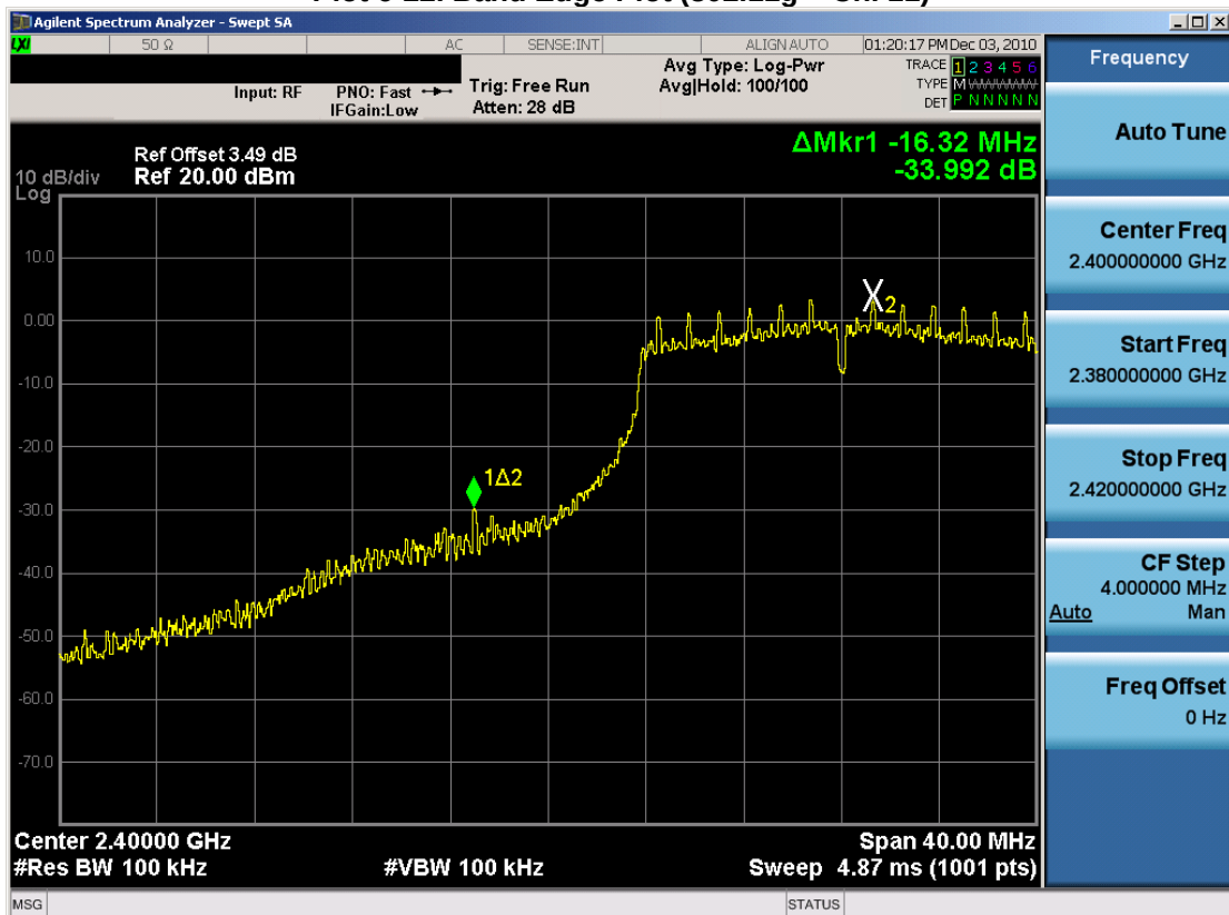
Plot 6-23. Band Edge Plot (802.11n – Ch. 1)
