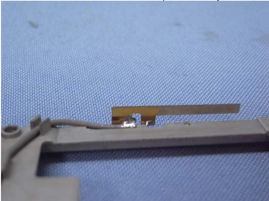
Figure 32 Internal View (Cable Assembly Antenna, Front View)
