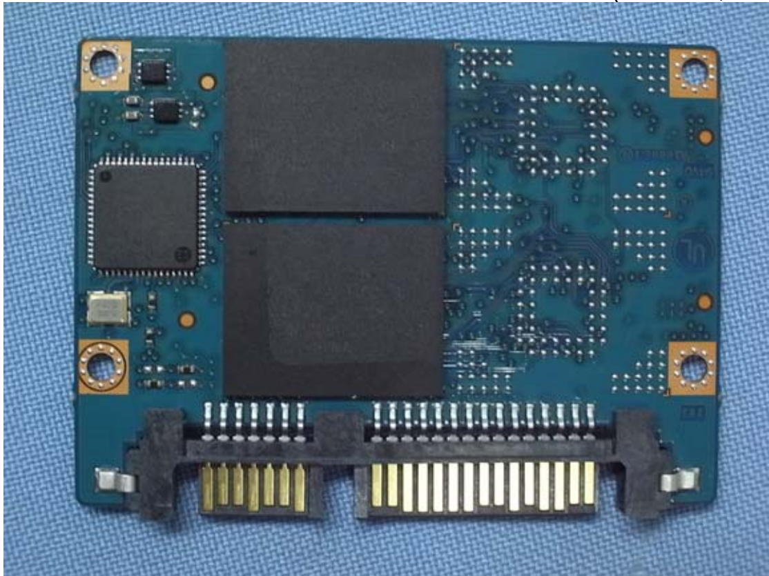
Figure 16 Internal View (SSD Card, Front View)
