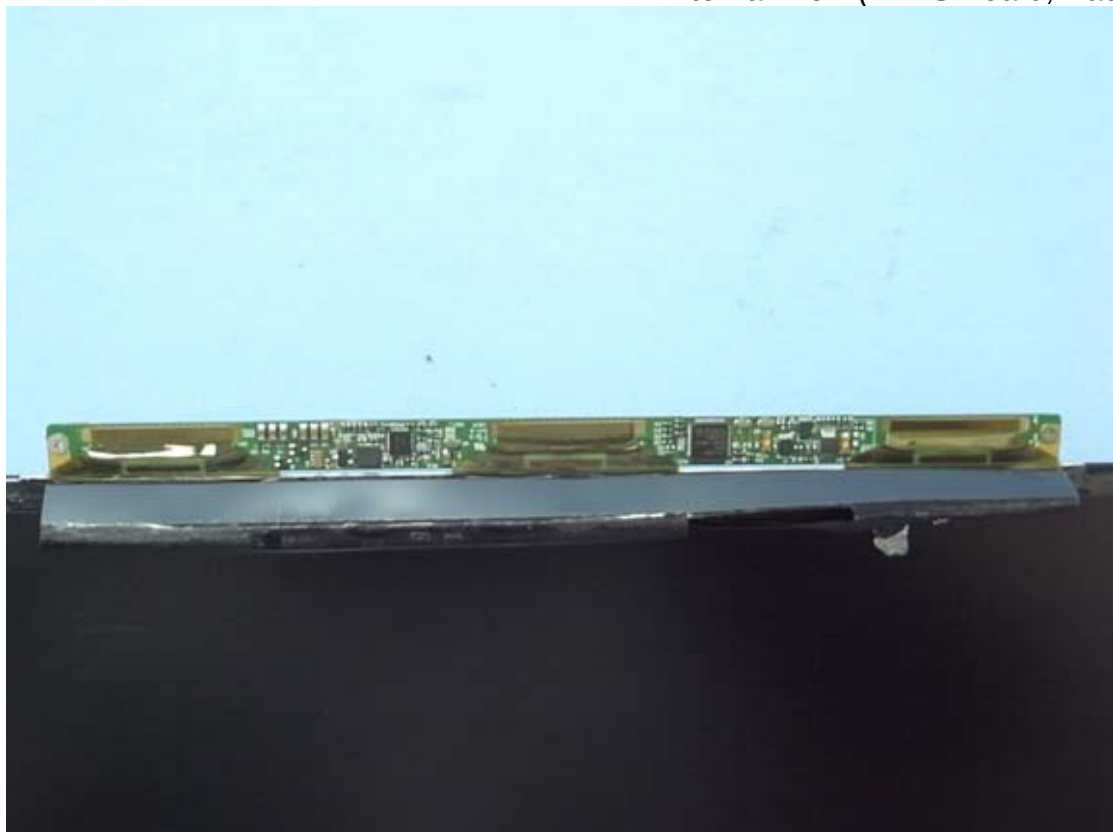
Figure 31 Internal View (LVDS Board, Back View)
