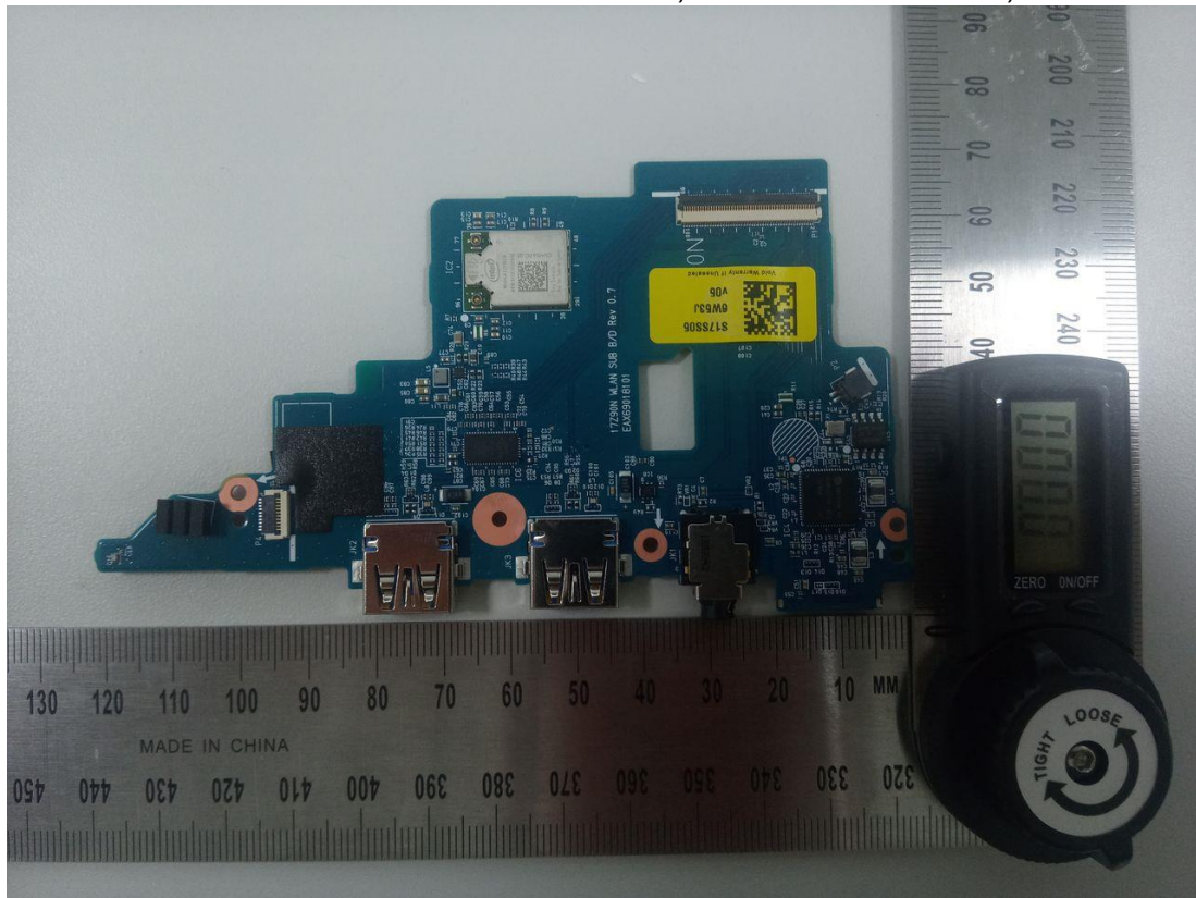
Figure 50 Elec & Eltek, WLAN SUB Board, Front View
