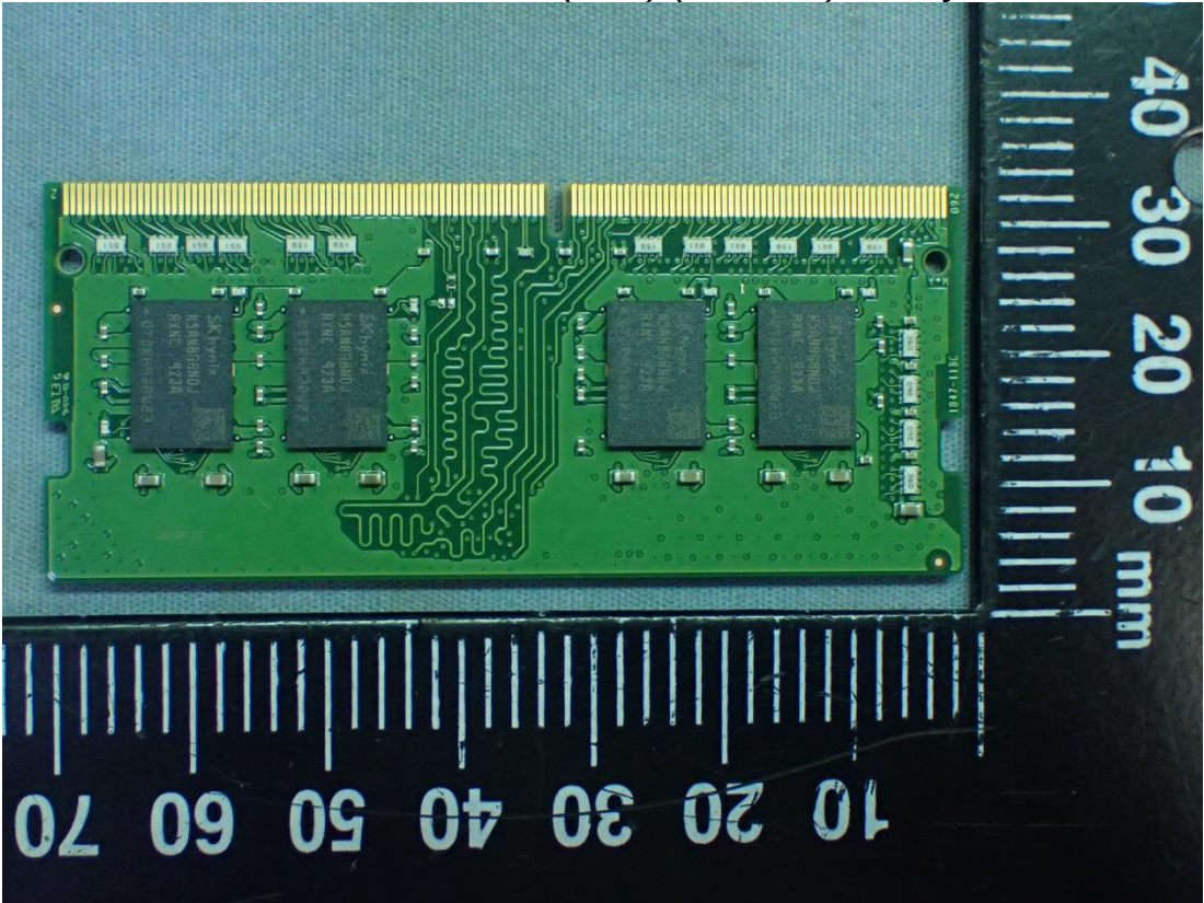
Figure 71 RAM (8GB) (On Card), SK hynix, Back View
