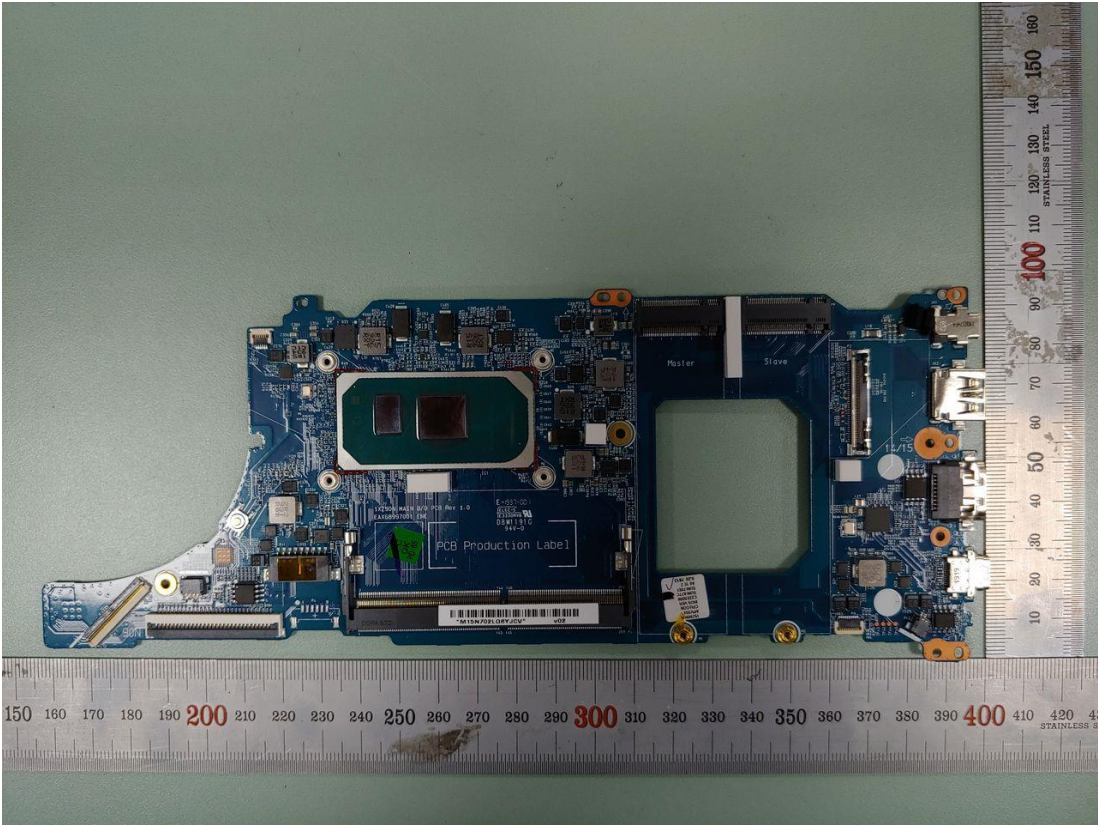
Figure 41 Elec & Eltek, Main Board, Front View
