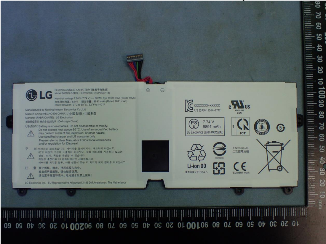
Figure 63 Battery Pack, Back View
