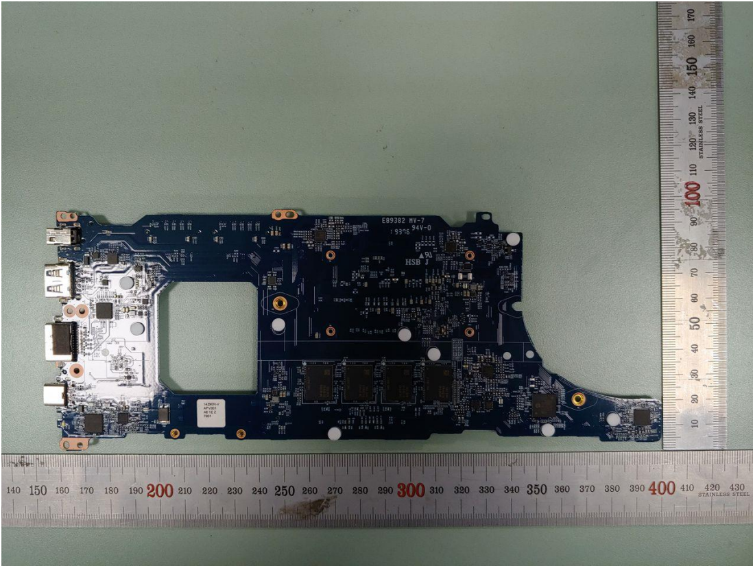
Figure 40 Hannstar, Main Board, Back View
