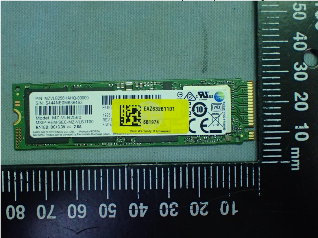
Figure 66 SSD (256GB), Samsung, Front View
