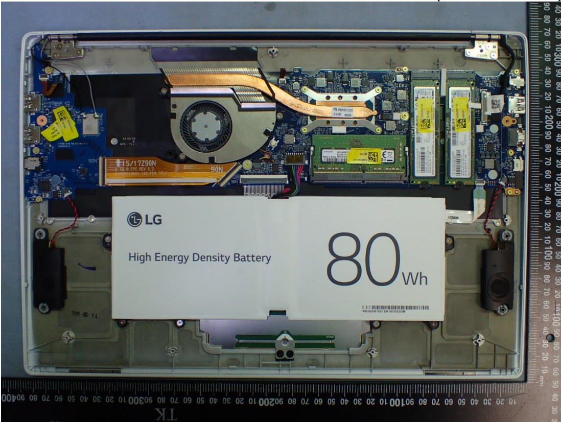
Figure 34 Internal View (Removed Cover)
