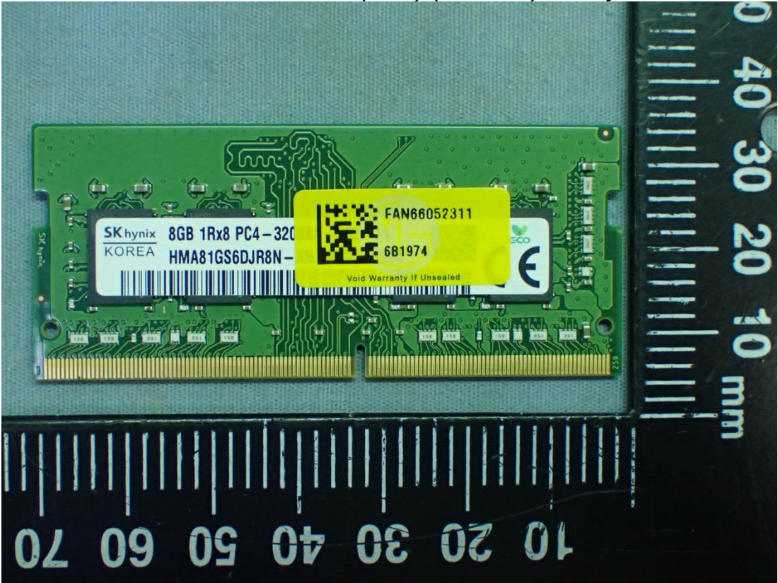
Figure 70 RAM (8GB) (On Card), SK hynix, Front View
