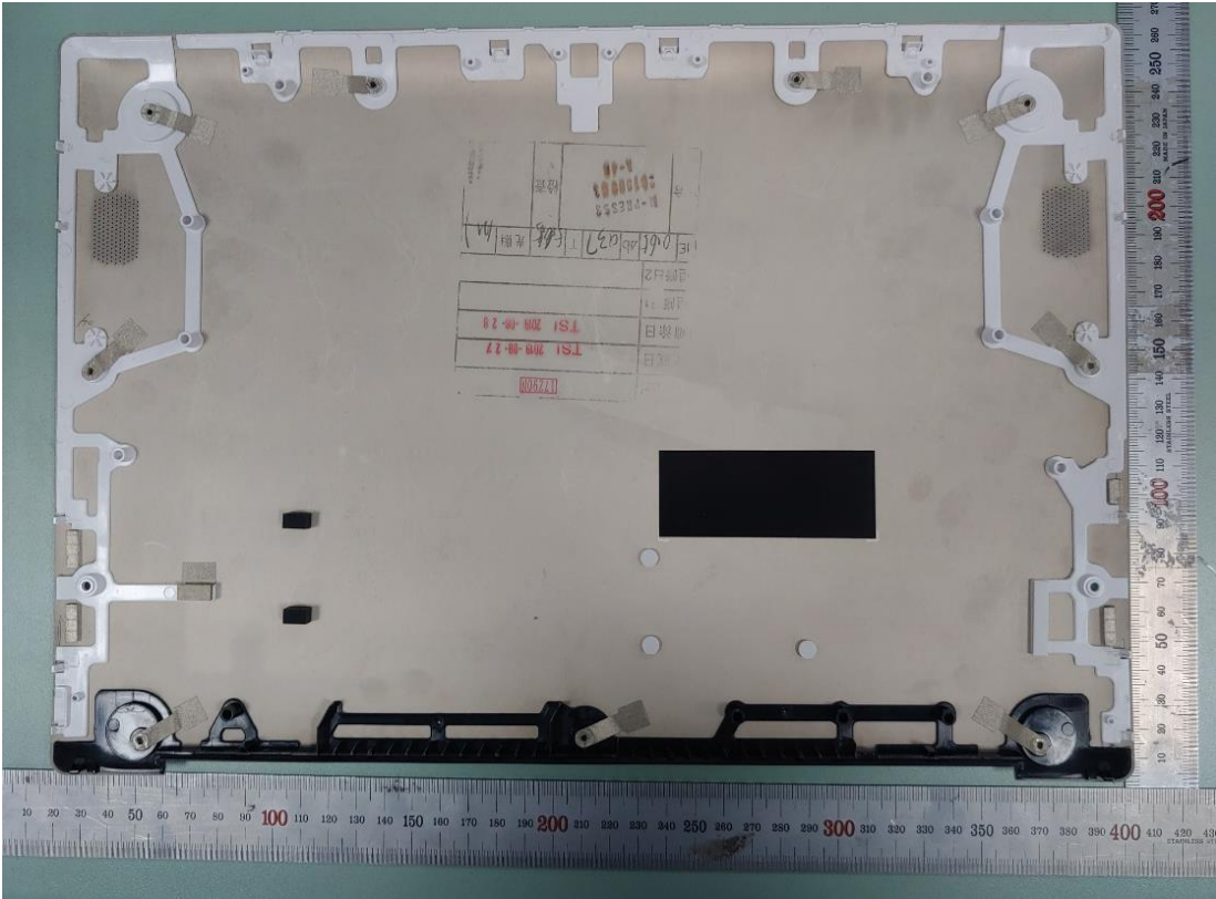
Figure 35 Internal View
