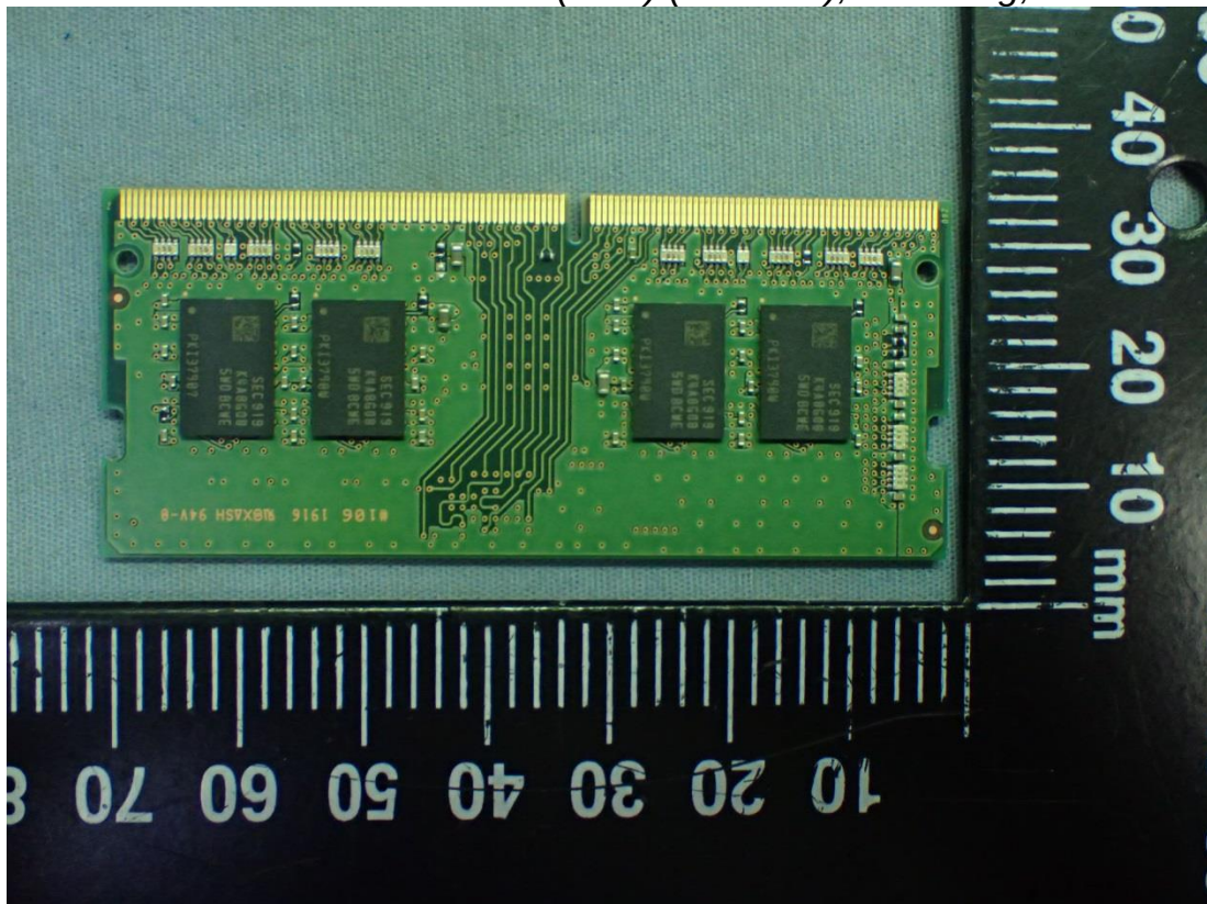
Figure 69 RAM (8GB) (On Card), Samsung, Back View
