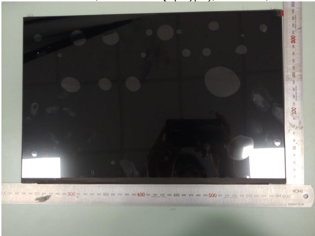
Figure 55 LGD, M/N LP170WQ1(SP)(A1), LCD Panel, Front View
