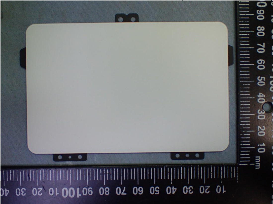
Figure 38 Internal View (Touch Pad, Front View)
