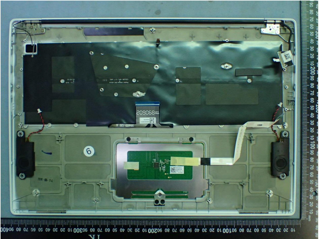
Figure 36 Internal View
