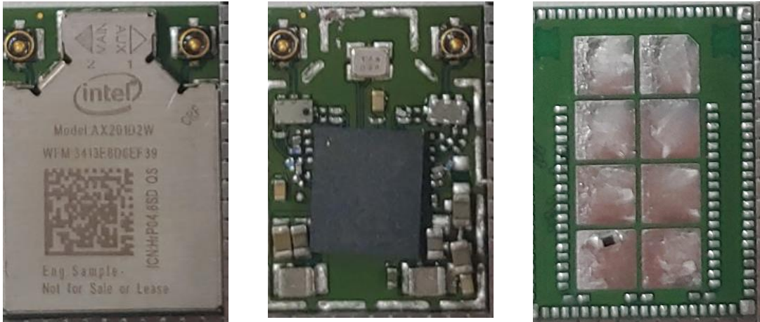
Figure 53 WLAN Combo Card, Remove Cover
