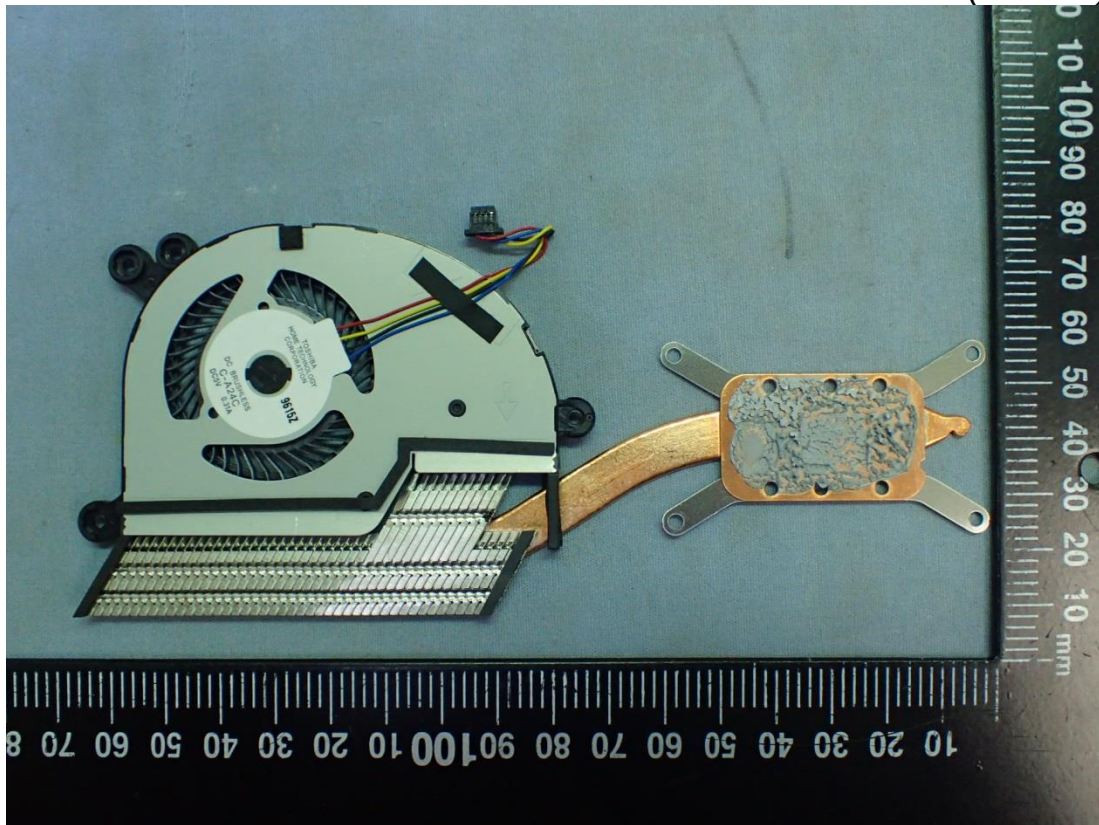
Figure 54 Internal View (DC Fan)
