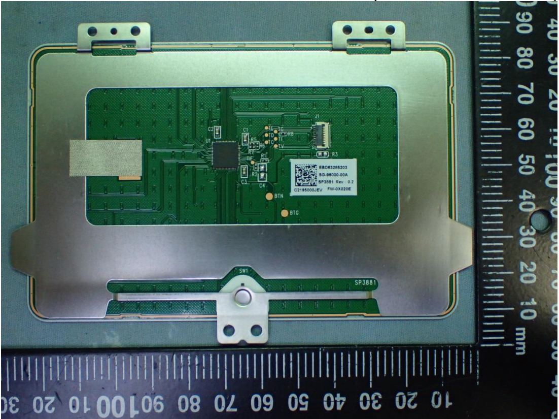
Figure 37 Internal View (Touch Pad, Back View)
