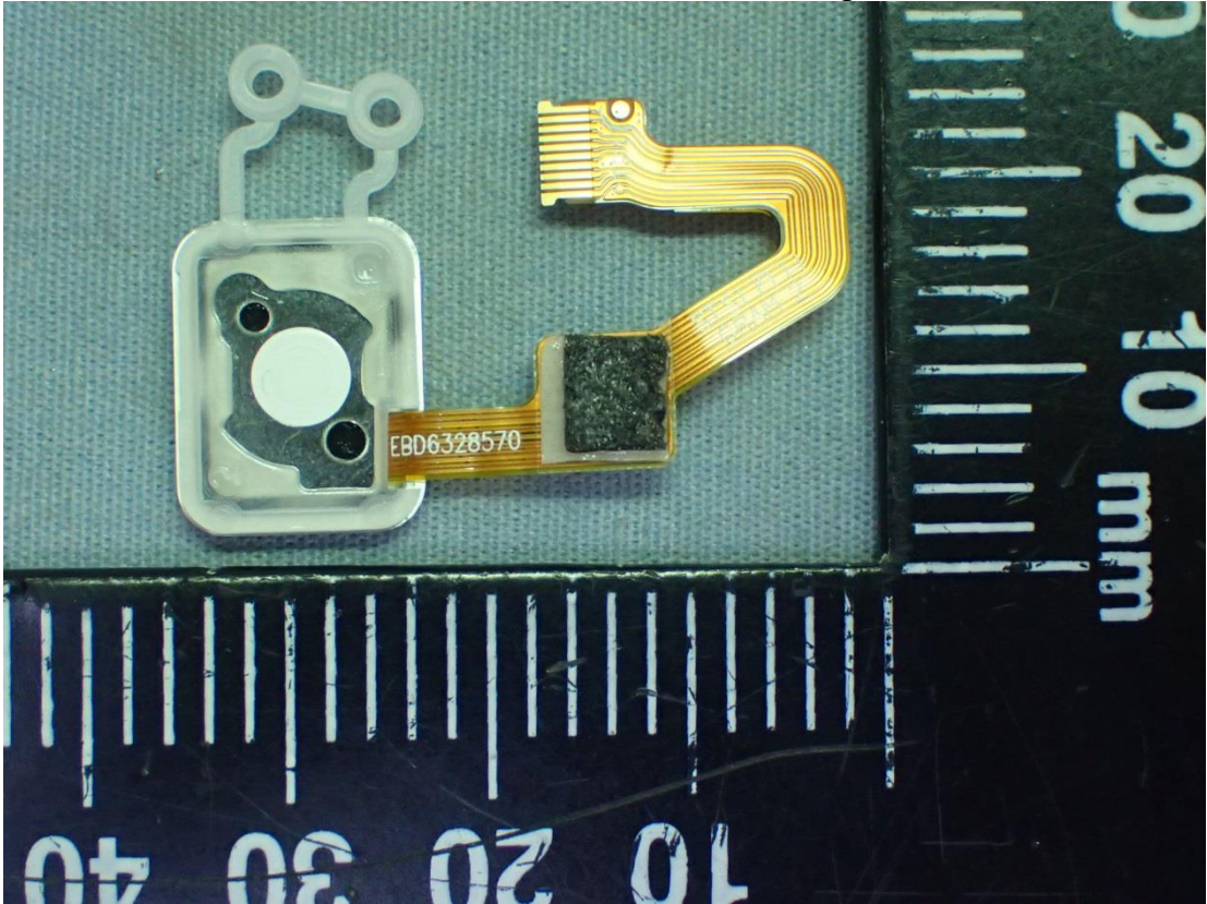
Figure 47 Finger Printer, Back View
