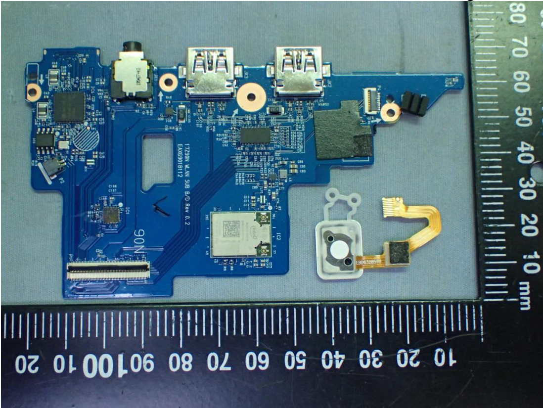
Figure 43 WLAN SUB Board, Removed Finger Printer
