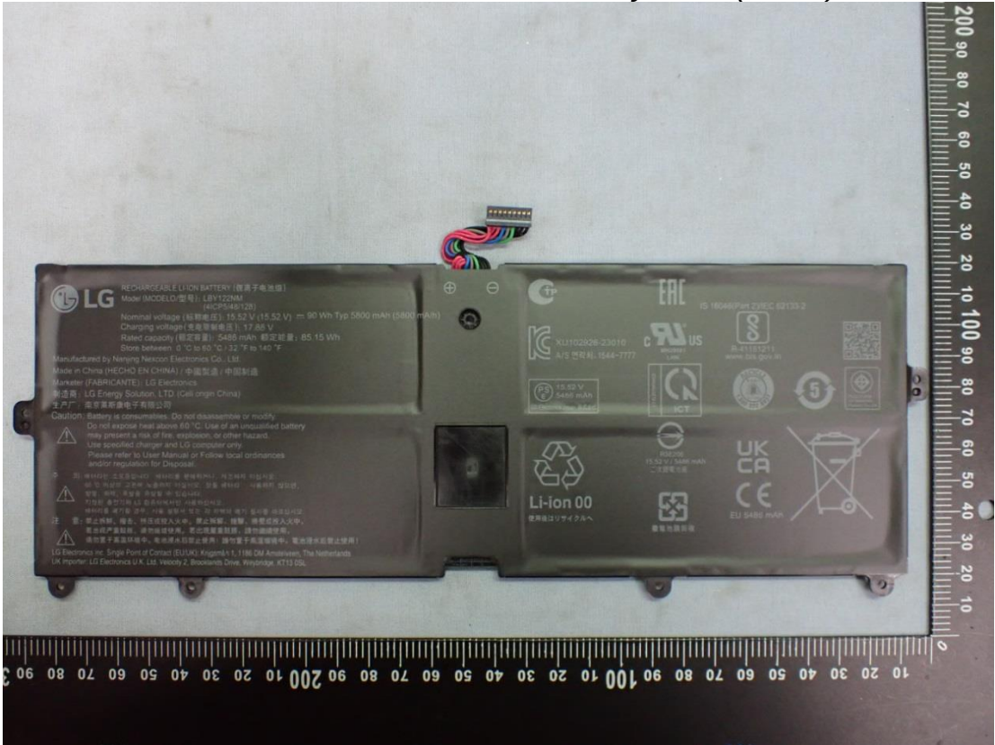
Figure 30 Battery Pack (90Wh), Back View
