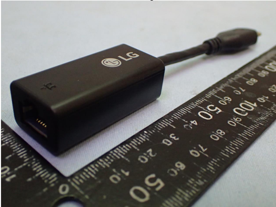
Figure 61 HUIZHOU DEHONG 100 Megabit Ethernet, LAN Gender View
