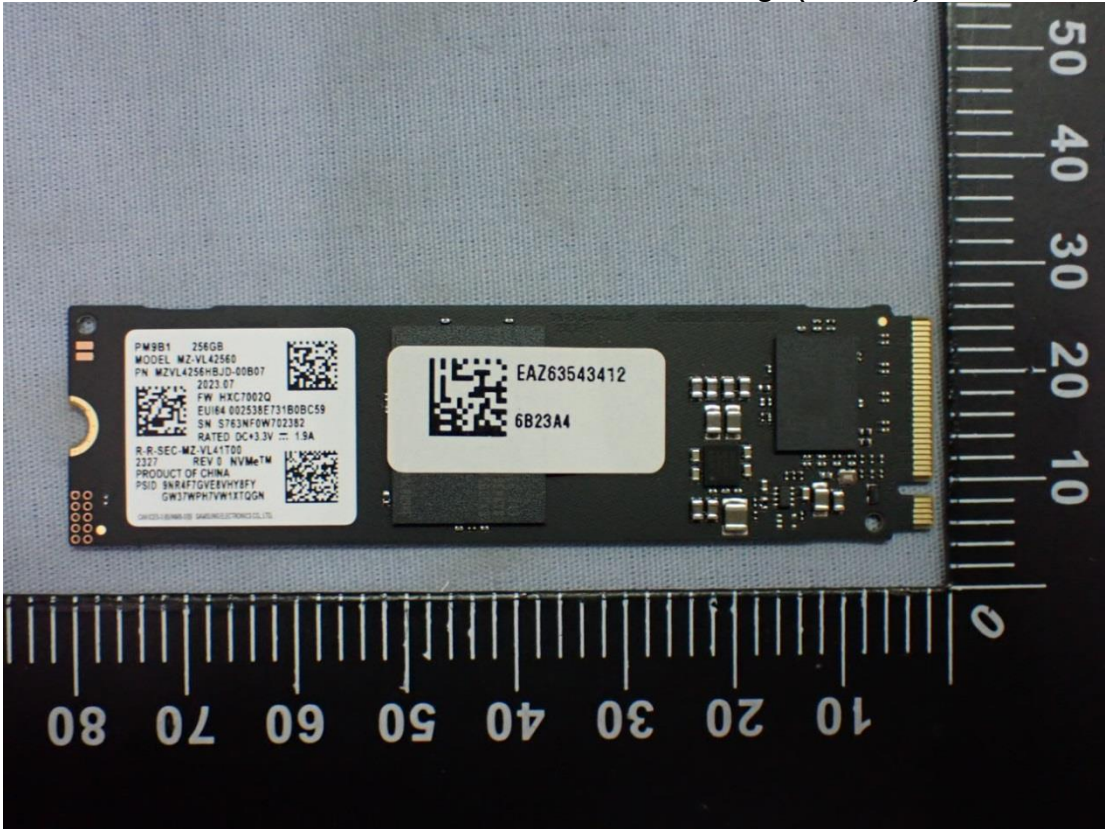
Figure 37 SSD, Samsung, (256GB), Front View
