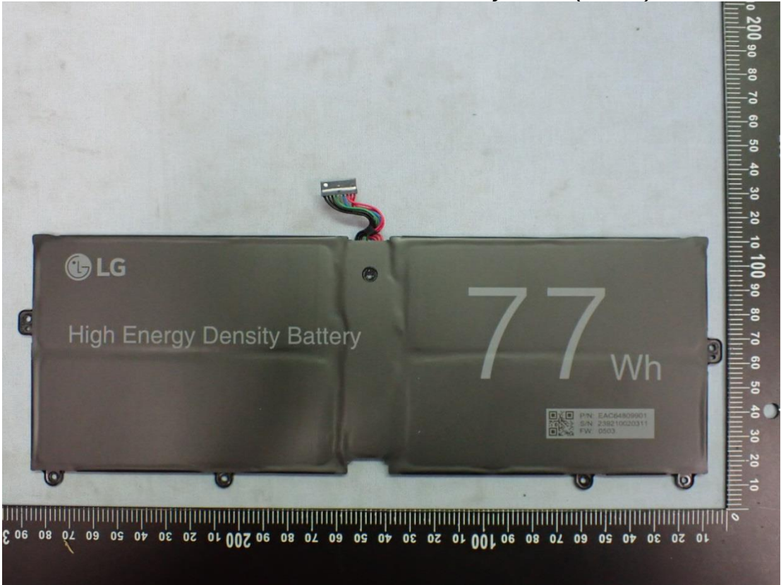
Figure 27 Battery Pack (77Wh), Front View
