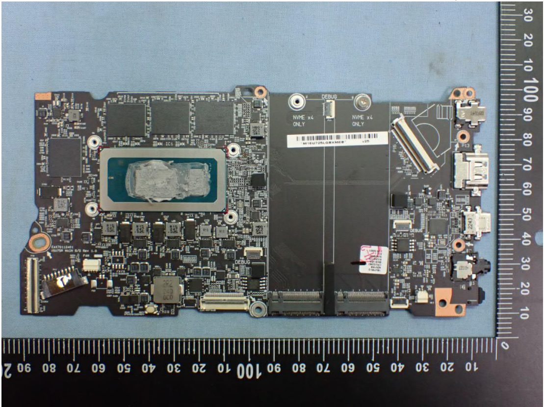
Figure 12 Main Board, Front View
