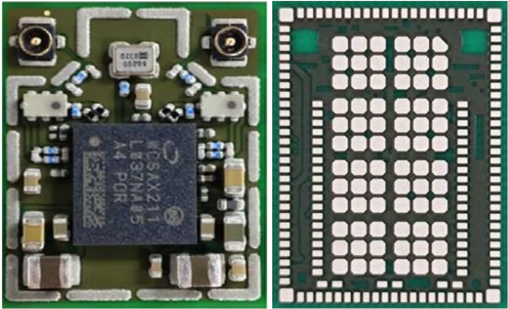
Figure 17 WLAN Combo Card, Without Shield and Back View
