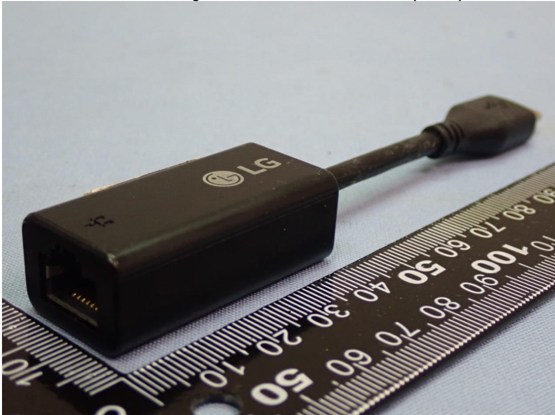
Figure 33 100 Megabit Ethernet, LAN Gender (Black), Front View
