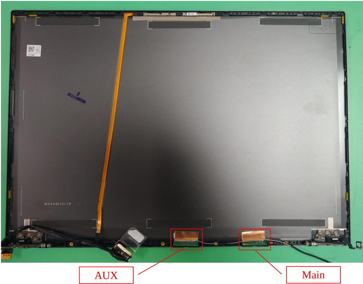
Figure 30 Antenna Location
