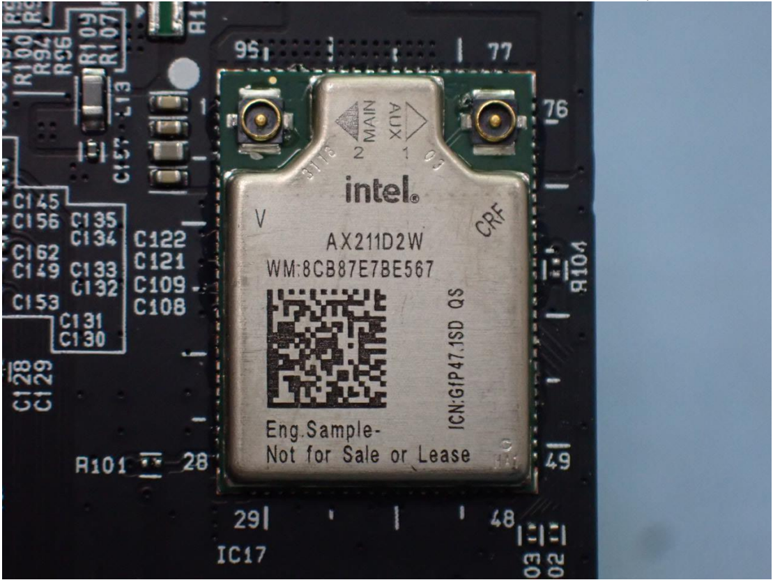
Figure 16 WLAN Combo Card, Front View
