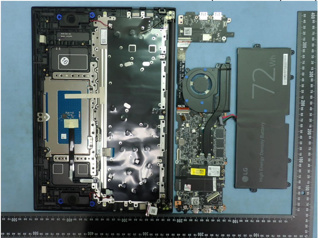
Figure 10 Internal View (Removed Components)
