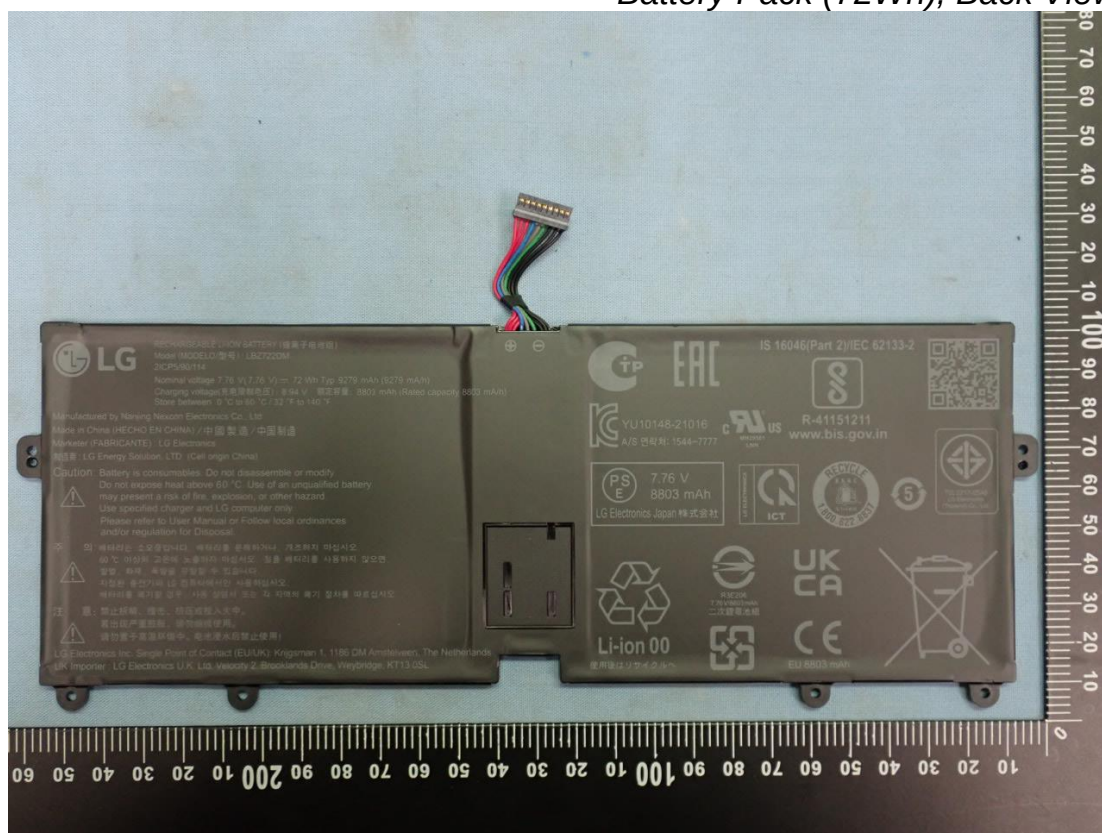
Figure 19 Battery Pack (72Wh), Back View
