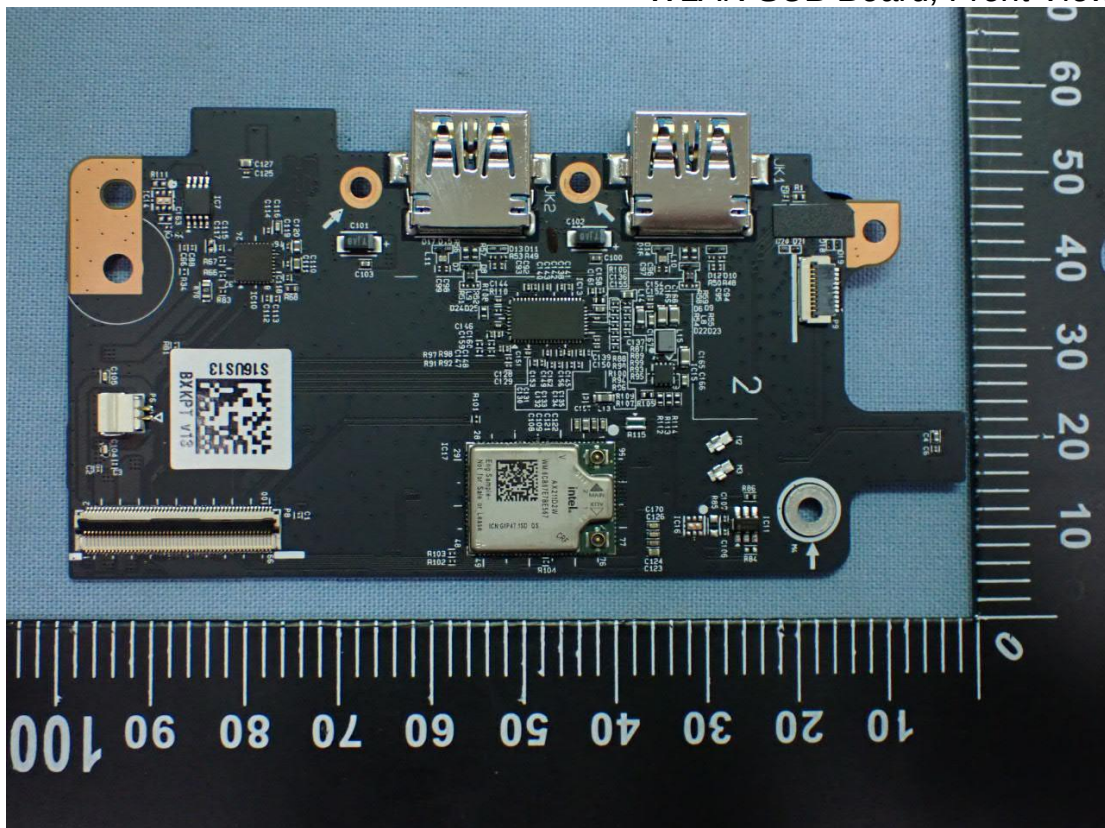
Figure 14 WLAN SUB Board, Front View
