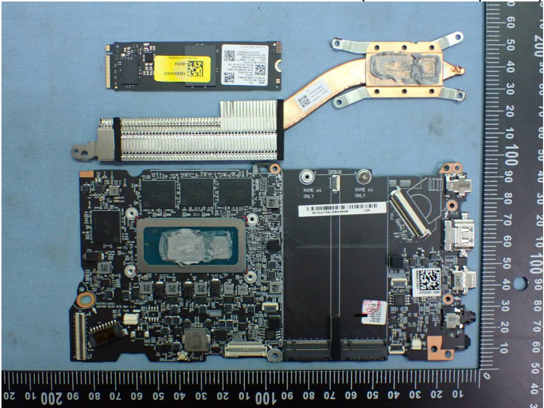
Figure 11 Main Board, Front View (Removed Components)
