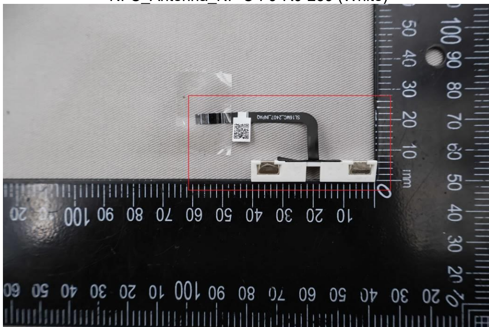
NFC_Antenna_NF-C-F9-R0-239 (White)
