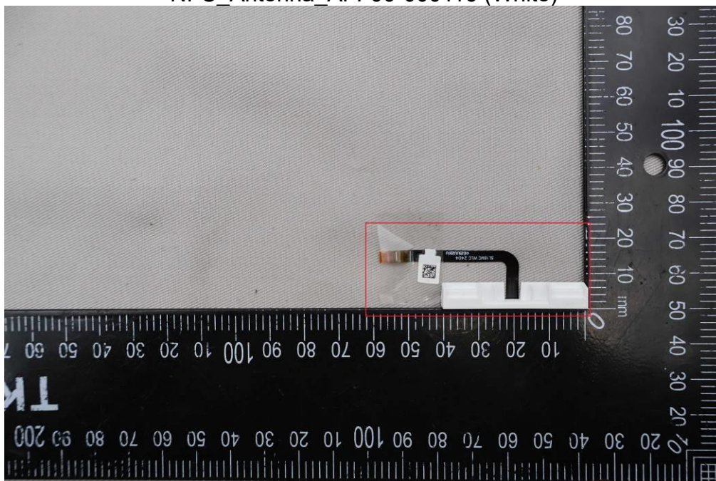
NFC_Antenna_AFF00-000116 (White)
