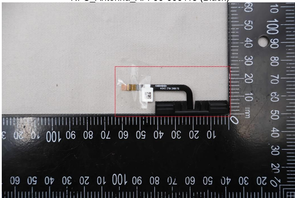
NFC_Antenna_AFF00-000115 (Black)
