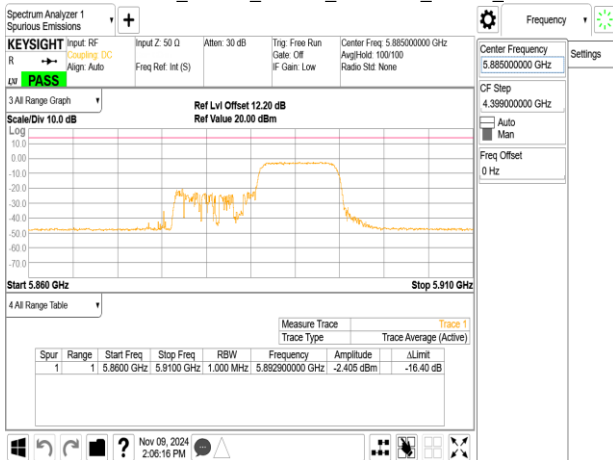
802.11ax_20MHz_ChainA_5885MHz_RU26_8
