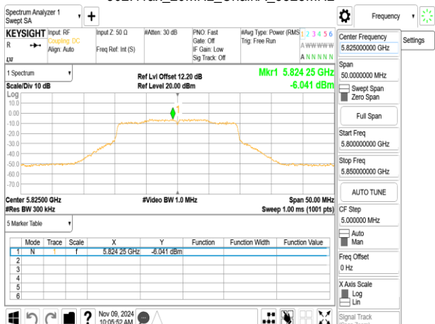
802.11ax_20MHz_ChainA_5825MHz
