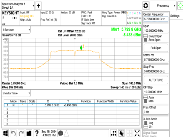
802.11n_40MHz_ChainA_5795MHz
