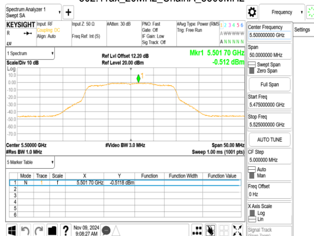
802.11ax_20MHz_ChainA_5500MHz_RU106_53
