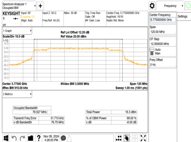
802.11ax_80MHz_ChainA_5775MHz_RU484_65
