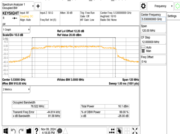
802.11ax_80MHz_ChainA_5530MHz
