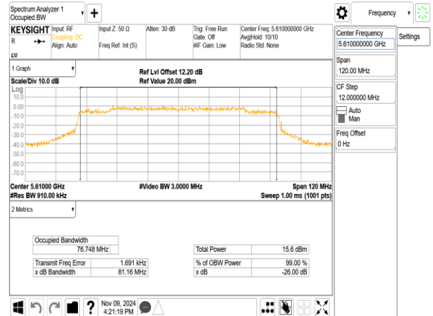
802.11ax_80MHz_ChainA_5610MHz_RU484_66
