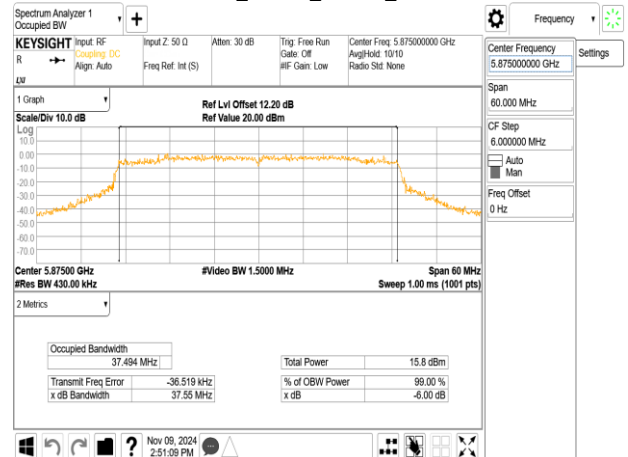
802.11ax_40MHz_ChainA_5875MHz
