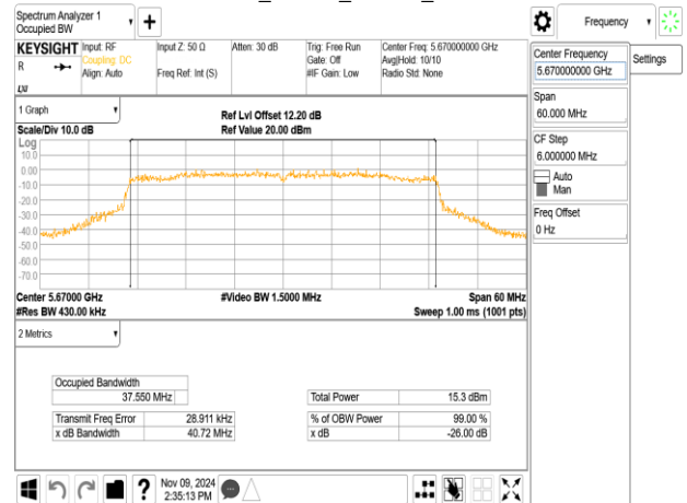
802.11ax_40MHz_ChainA_5670MHz_RU242_62
