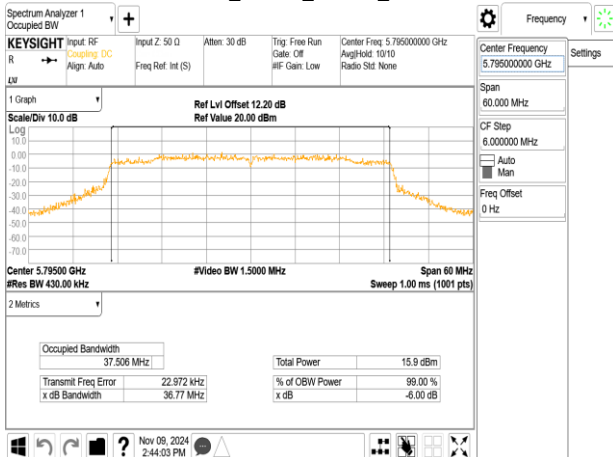
802.11ax_40MHz_ChainA_5795MHz
