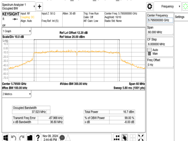
802.11ax_40MHz_ChainA_5795MHz
