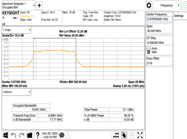
802.11ax_40MHz_ChainA_5875MHz_RU242_62
