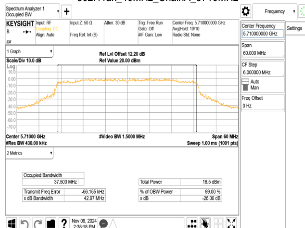
802.11ax_40MHz_ChainA_5710MHz
