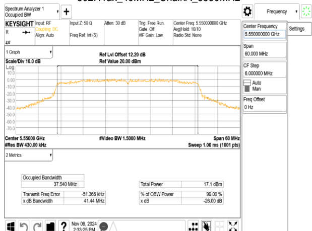
802.11ax_40MHz_ChainA_5550MHz
