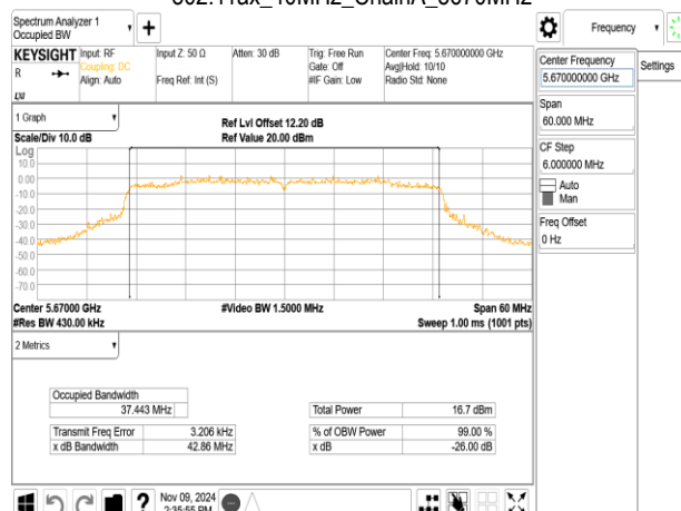
802.11ax_40MHz_ChainA_5670MHz_RU242_62
