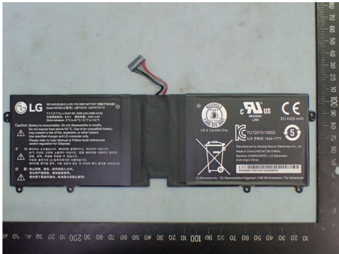
Figure 12 Internal View (LG, M/N: LBP7221E Battery Pack, Label View)
