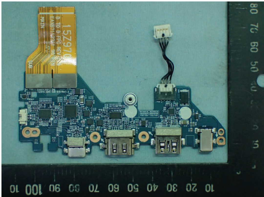
Figure 24 Internal View (E&E/ HANNSTAR, M/N 15Z970 HDMI SUB HDMI (Non TBT3 Model) Board, Front View)
