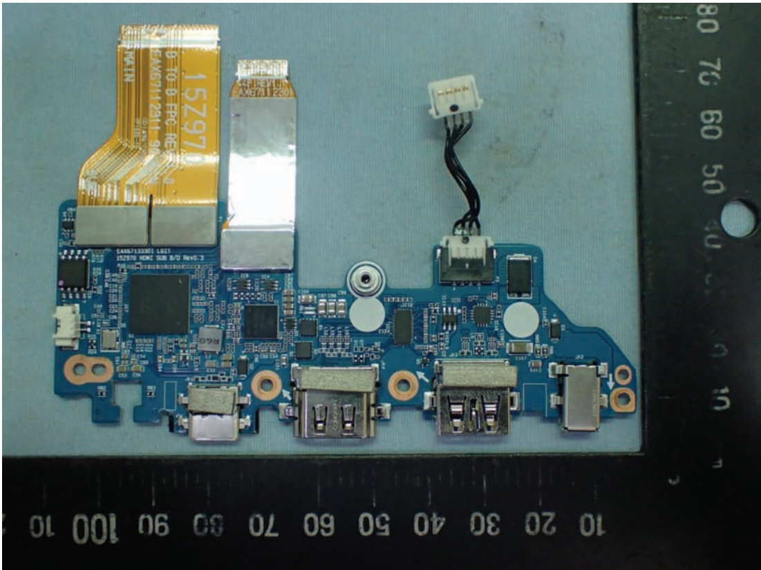
Figure 22 Internal View (LGIT/E&E, M/N 15Z970 HDMI SUB HDMI (TBT3 Model) Board, Front View)
