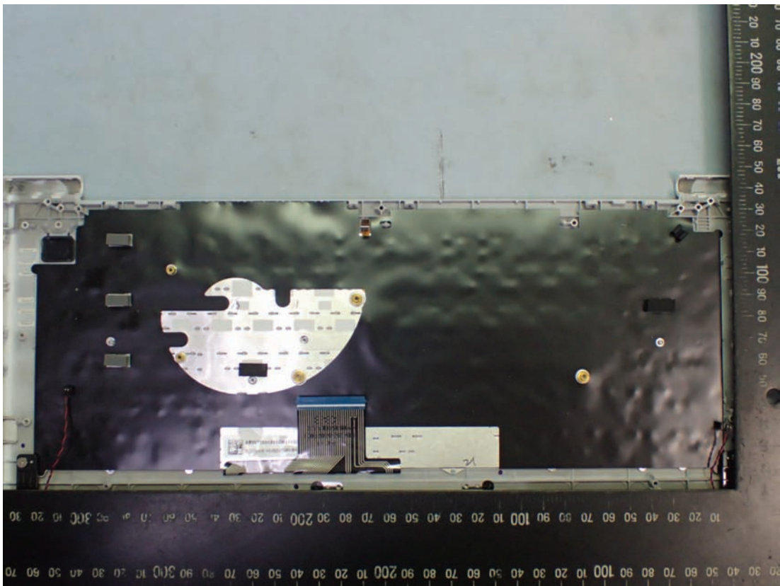
Figure 14 Internal View (LG, M/N 15Z970 KR HMB8154ELB13 Keyboard)
