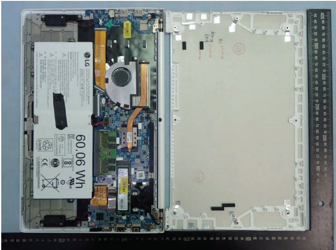
Figure 6 Internal View (Remove Cover, With 60W Battery)
