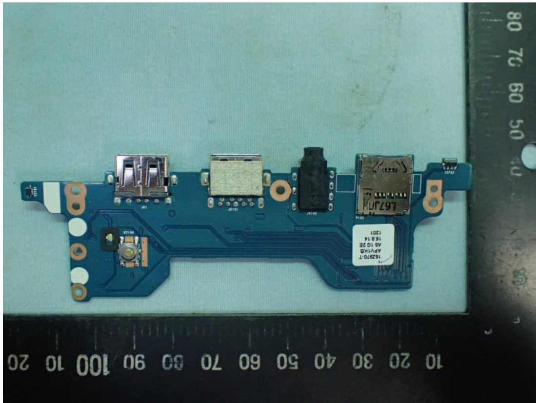
Figure 28 Internal View (HANNSTAR, M/N15Z970 WLAN SUB Board, Front View)
