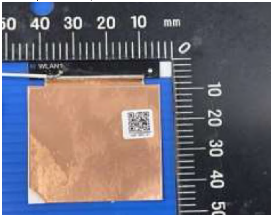
(32) EUT Photo (Antenna: Pulse)
