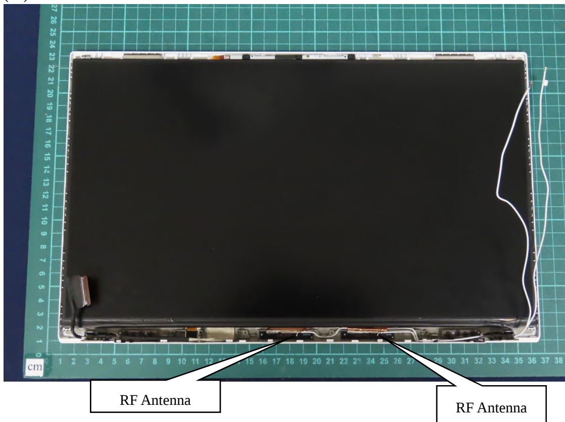
(28) EUT Photo
