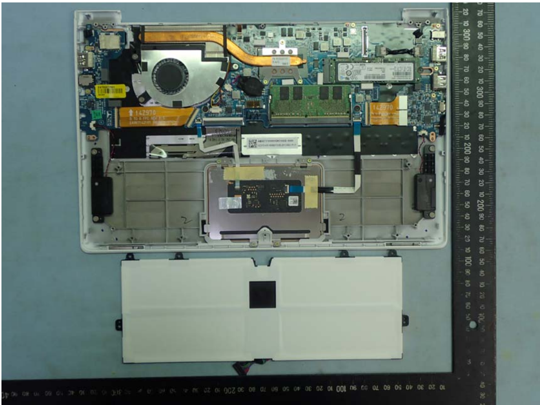
Figure 8 Internal View
