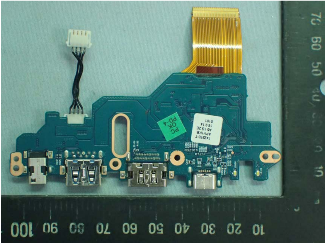
Figure 24 Internal View (ENE, M/N 13Z970 HDMI SUB Board, Front View)
