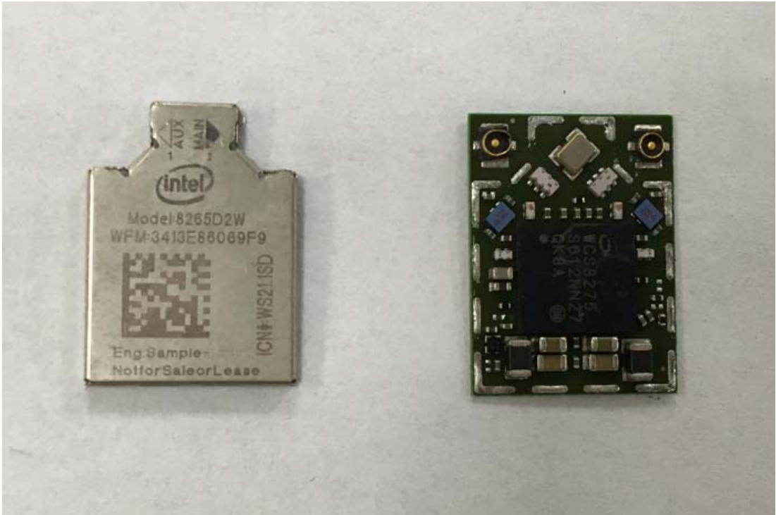
Figure 32 Internal View (WLAN Combo Card, Back View)
