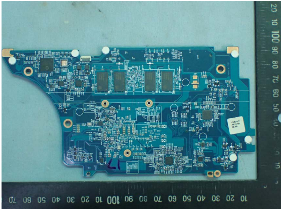
Figure 34 Internal View (LGIT, M/N 13/14/15Z970 Main Board, Back View)
