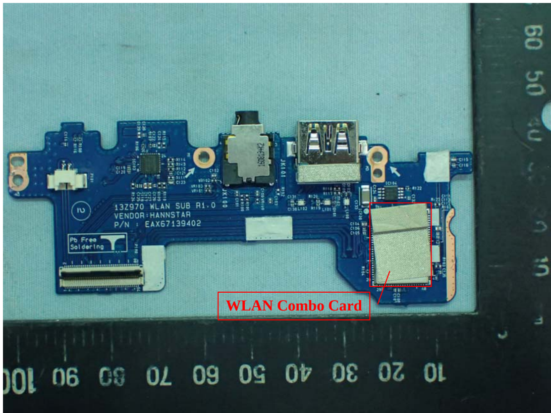
Figure 28 Internal View (HANNSTAR, M/N13Z970 WLAN SUB Board, Front View)
