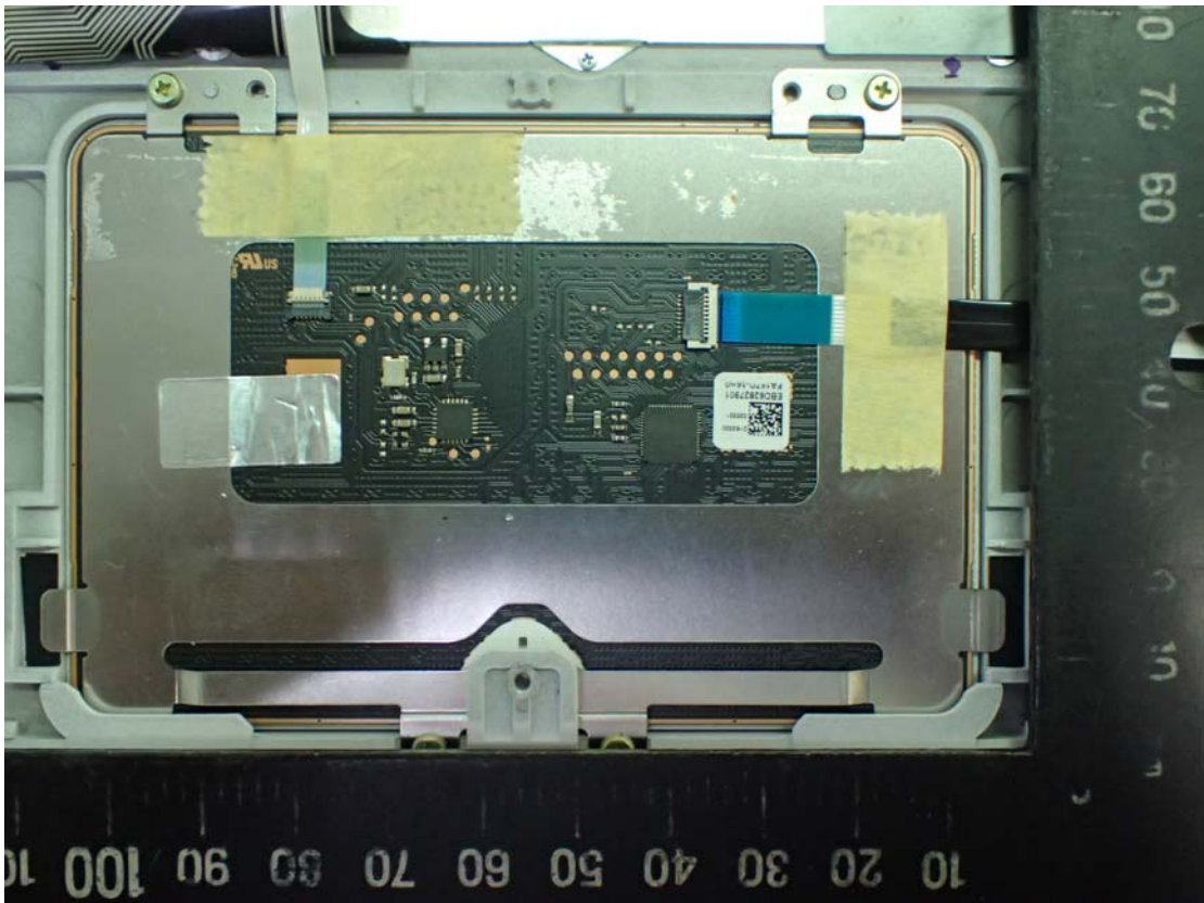
Figure 16 Internal View (LG, M/N EBD62827901 FA167D-16H0 Touch Pad)
