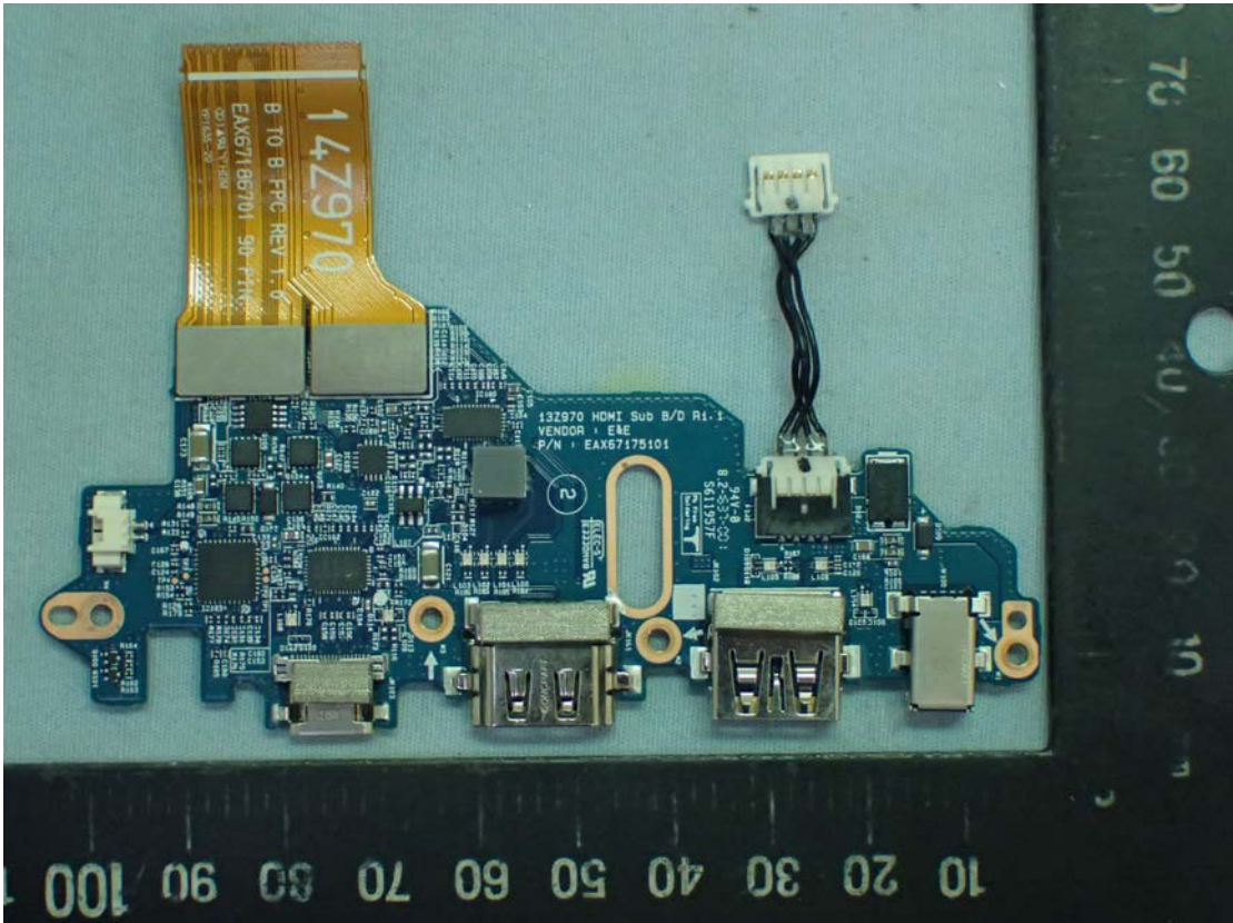
Figure 22 Internal View (E&E, M/N 13Z970 HDMI SUB Board, Front View)
