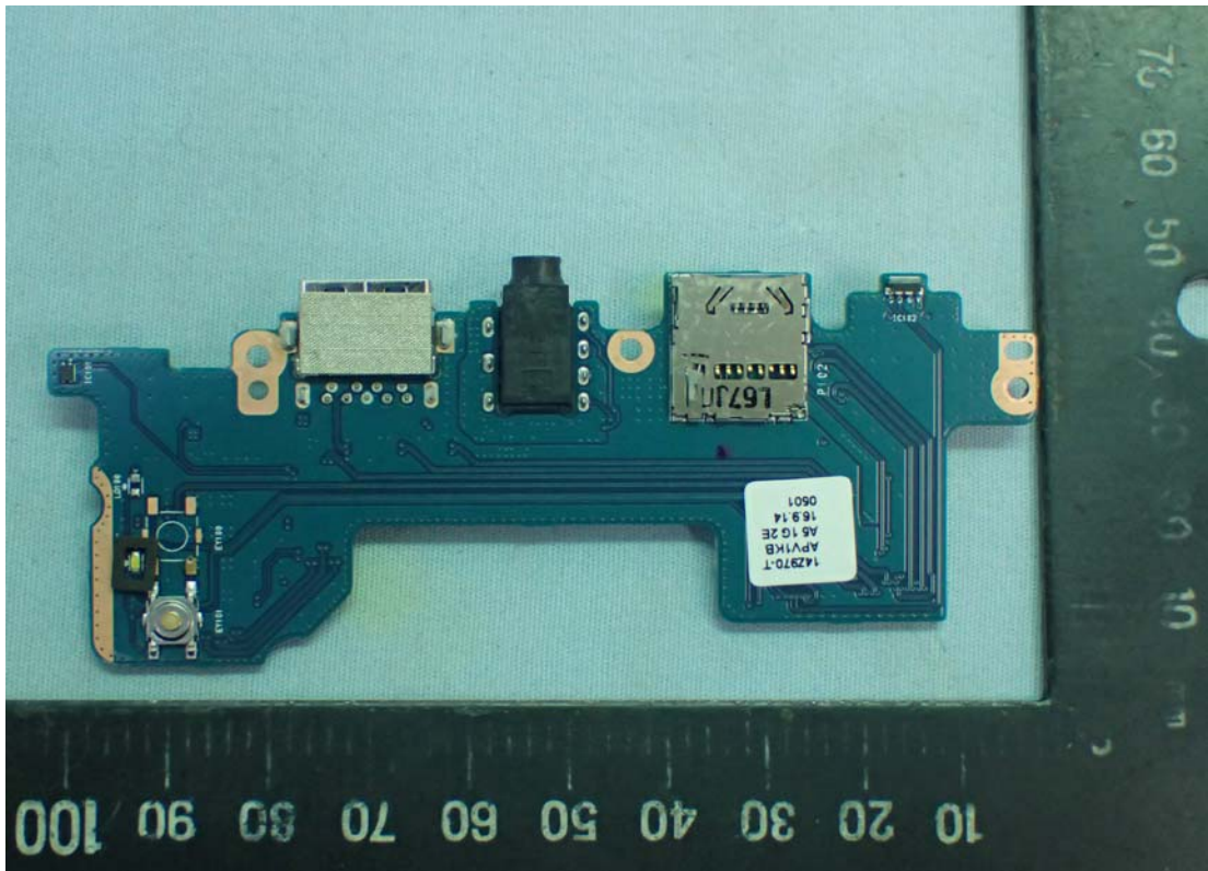
Figure 28 Internal View (HANNSTAR, M/N13Z970 WLAN SUB Board, Front View)
