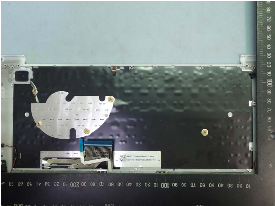
Figure 14 Internal View (LG, M/N 13Z970 KR HMB8150ELB13 Keyboard)
