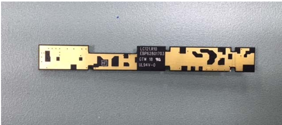
Figure 38 Internal View (Web Camera, Back View)
