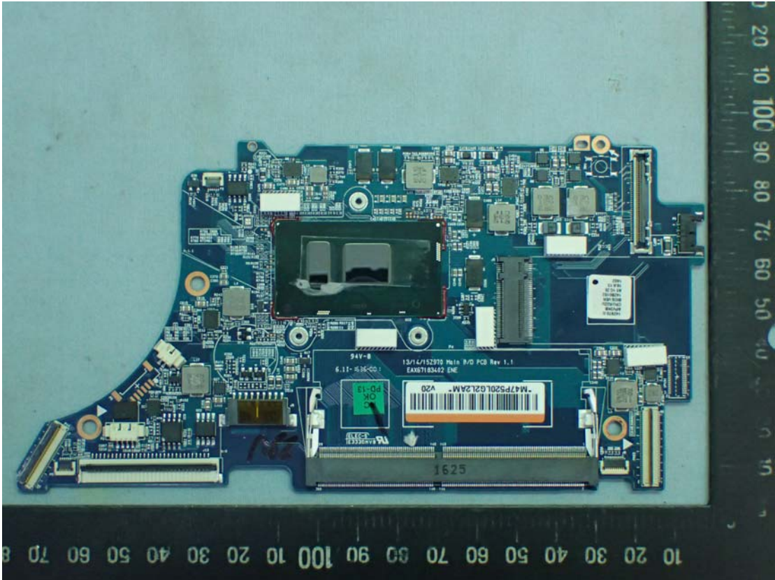
Figure 36 Internal View (ENE, M/N 13/14/15Z970 Main Board, Back View)
