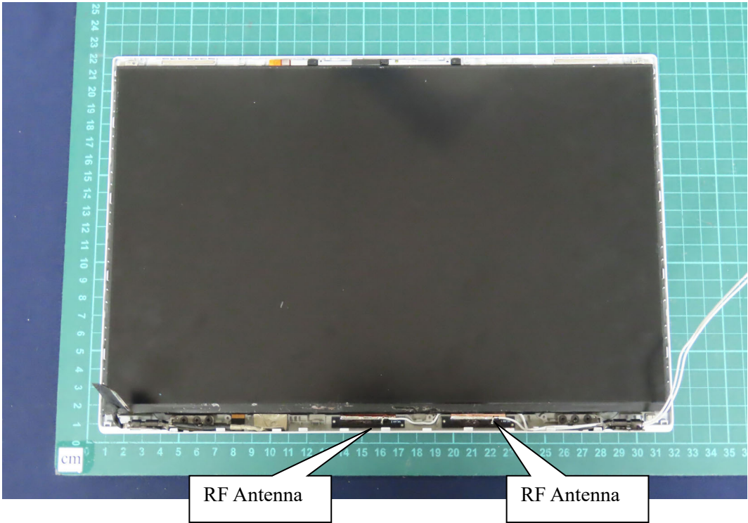
(29) EUT Photo
