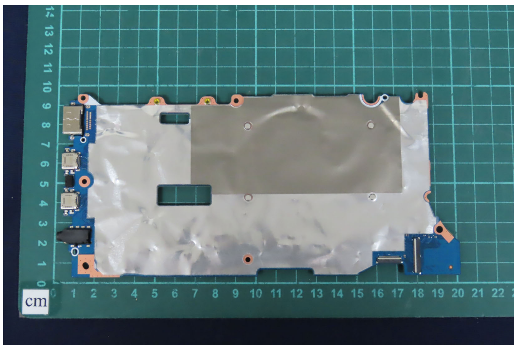
(22) EUT Photo
