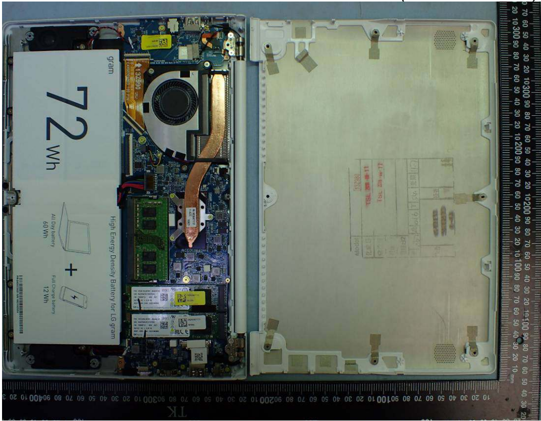
Figure 17 Internal View (Removed Cover)
