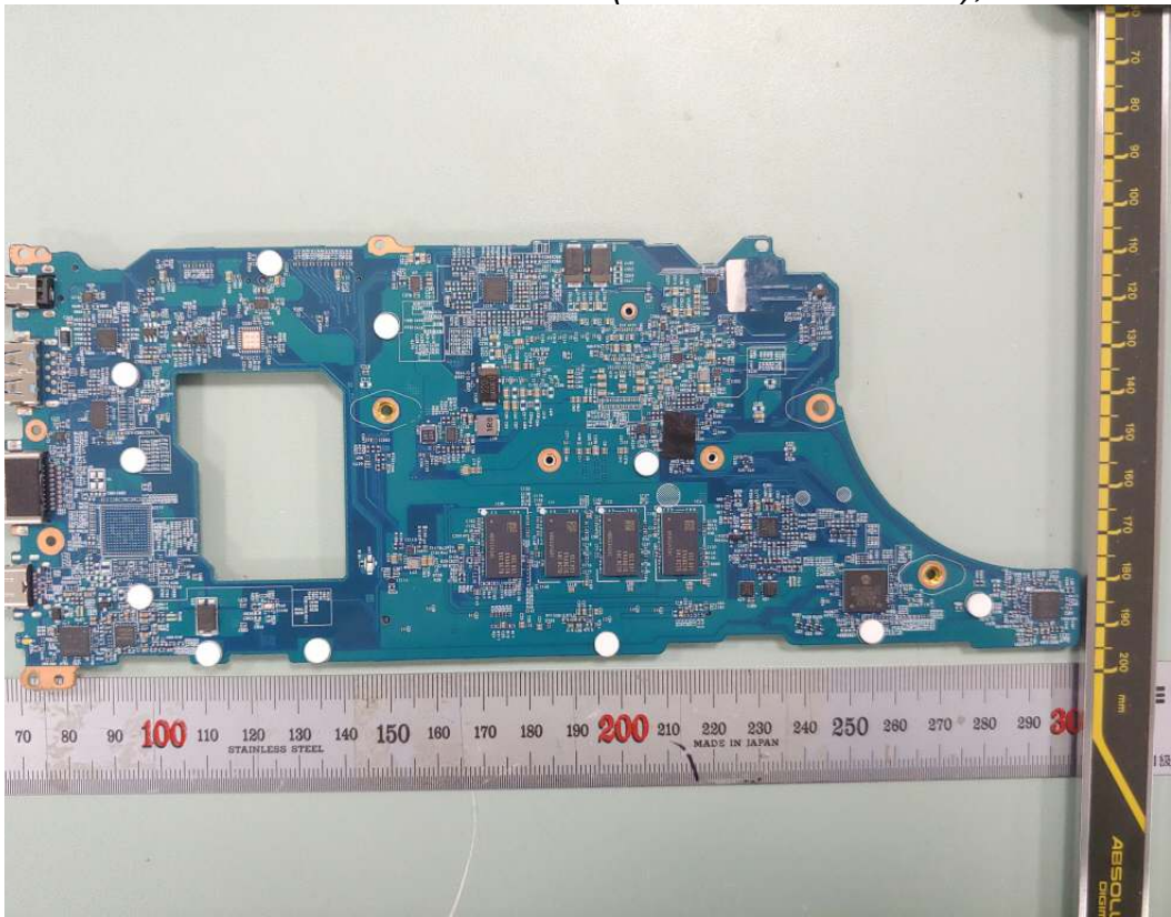
Figure 28 Main Board (without Thunderbolt), Back View
