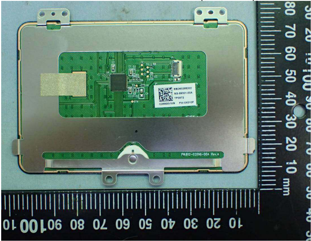
Figure 52 Touch Pad (Dark Silver), Back View
