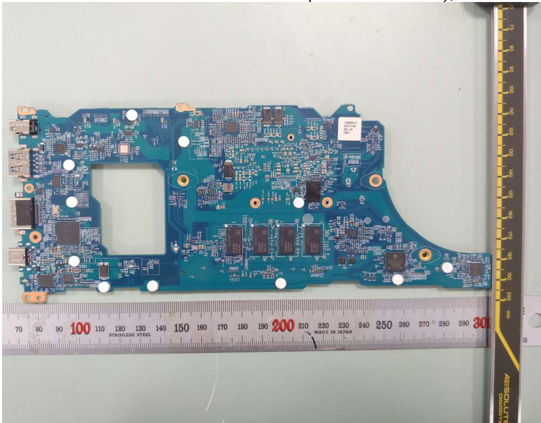
Figure 26 Main Board (with Thunderbolt), Back View
