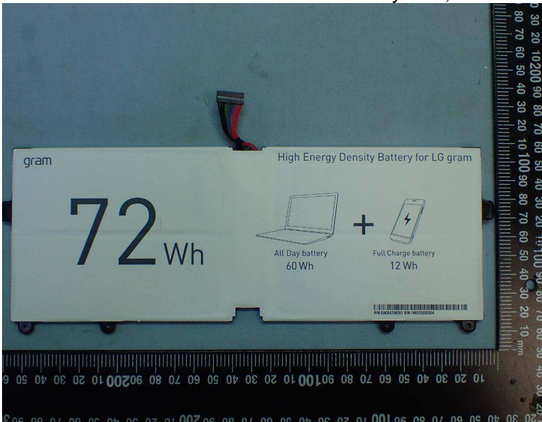
Figure 43 Battery Pack, Front View
