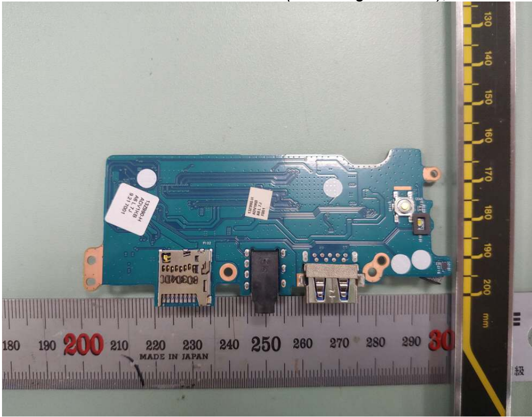
Figure 31 SUB Board (With Finger Printer), Back View
