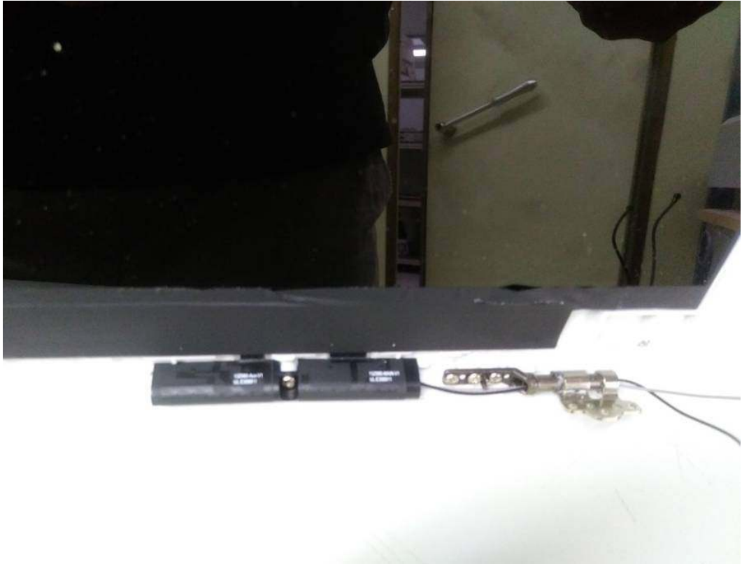
Figure 37 WLAN Combo Antenna Location
