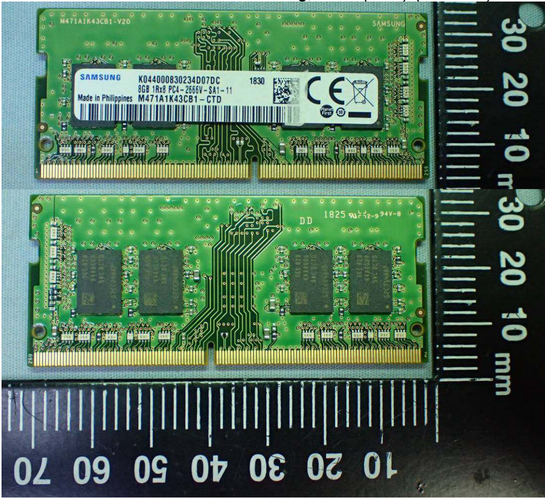
Figure 48 Samsung, RAM (8GB) (On Card) View
