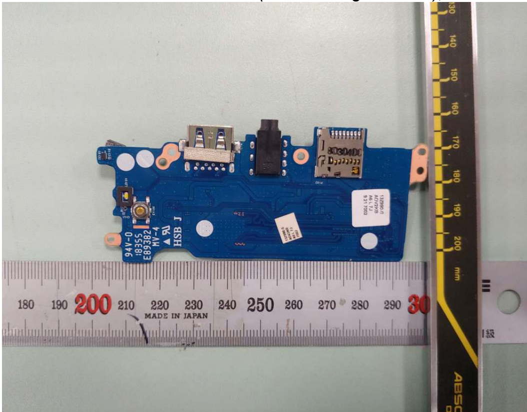
Figure 33 SUB Board (Without Finger Printer), Back View
