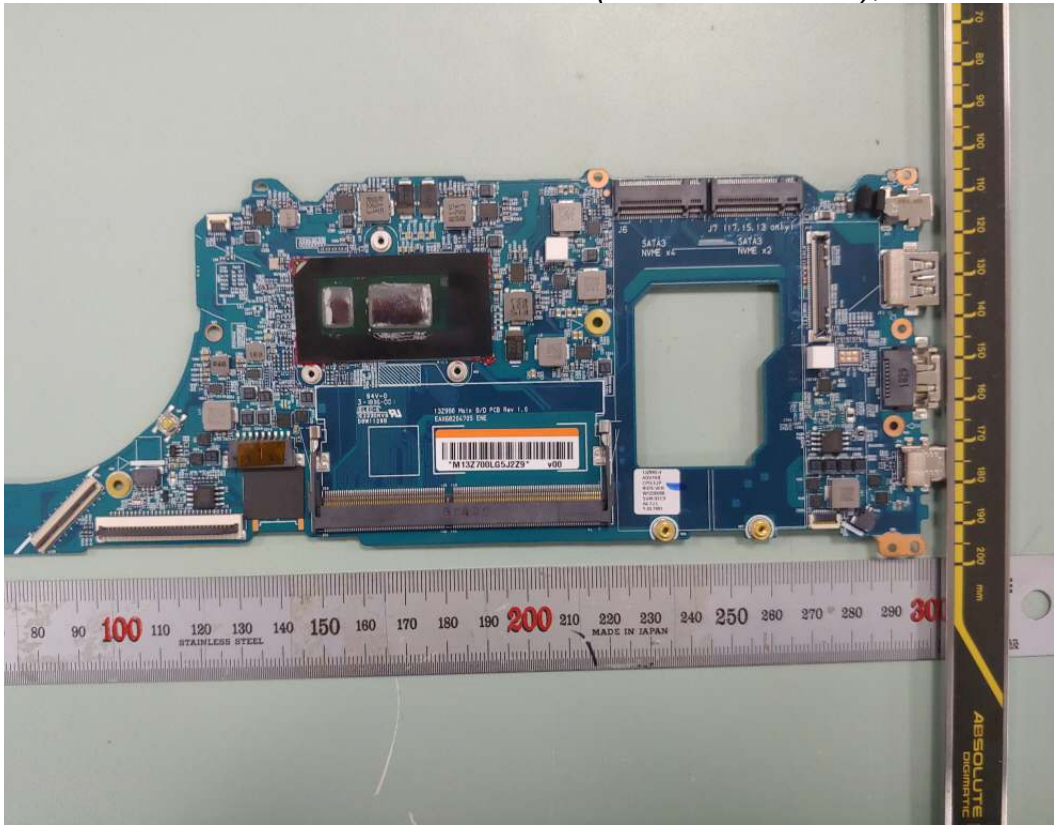
Figure 25 Main Board (with Thunderbolt), Front View
