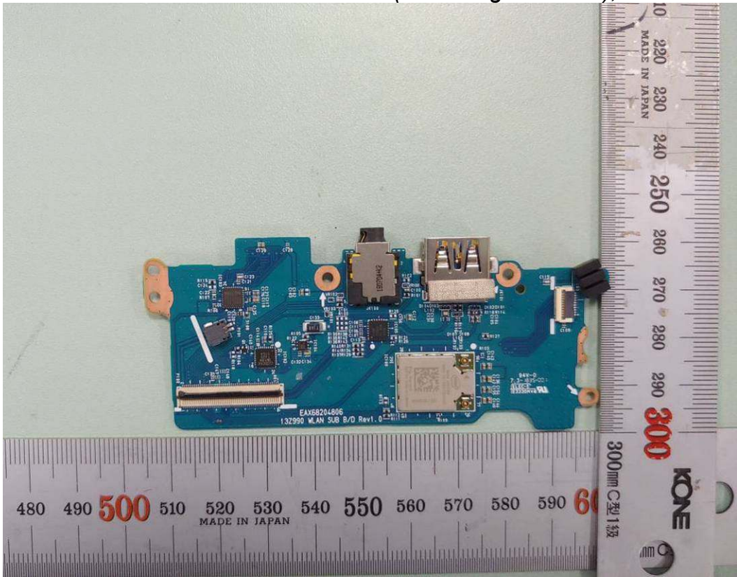
Figure 30 SUB Board (With Finger Printer), Front View
