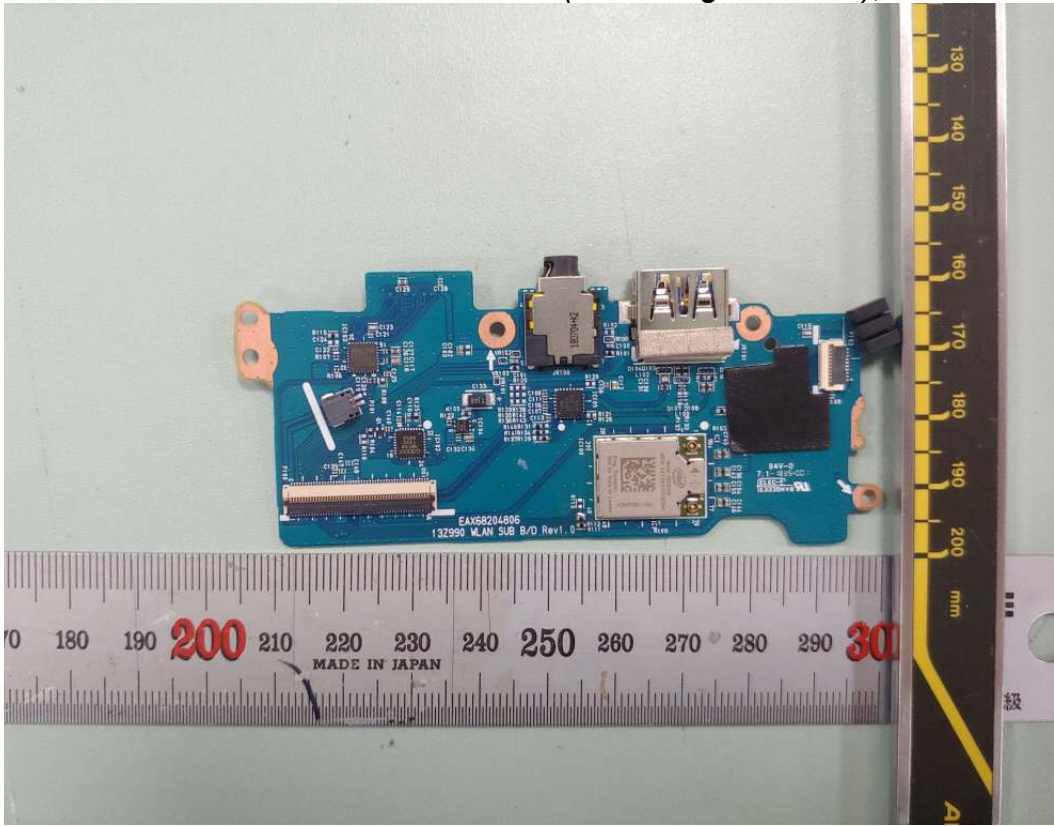
Figure 29 SUB Board (With Finger Printer), Front View
