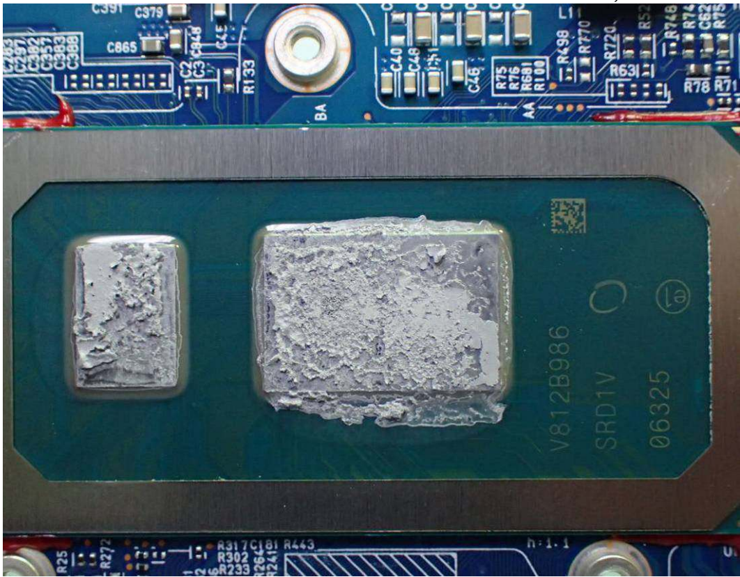
Figure 42 i3-8145U, CPU View
