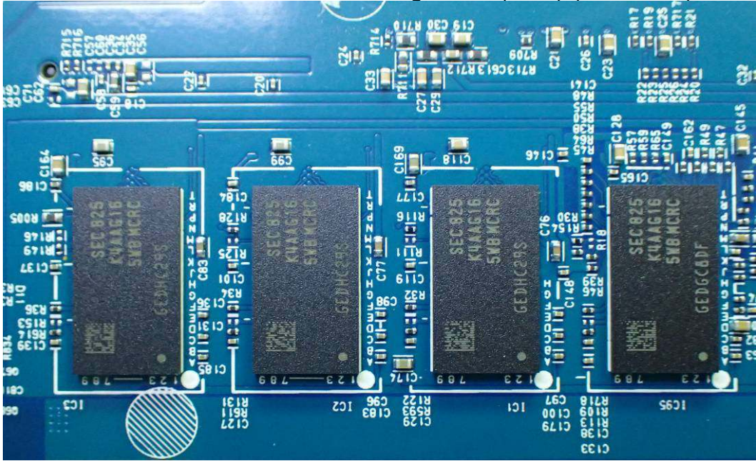
Figure 47 Samsung, RAM (8GB) (On Board) View
