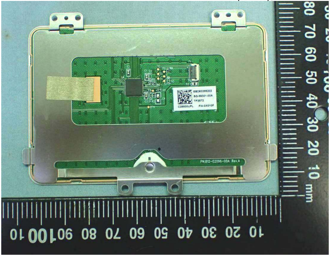
Figure 50 Touch Pad (White), Back View
