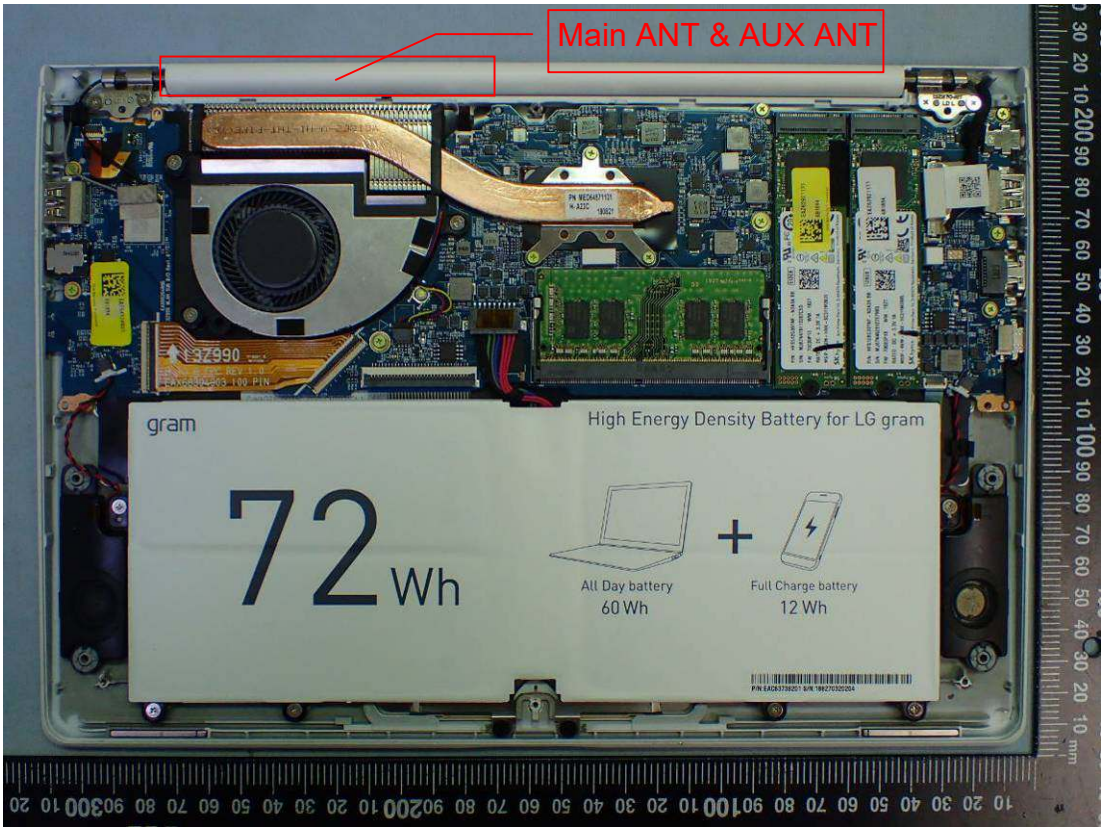
Figure 39 WLAN Combo Antenna
