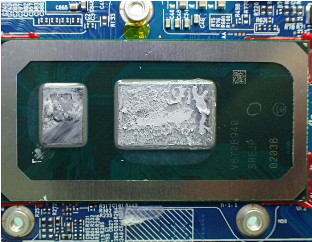
Figure 40 i7-8565U, CPU View
