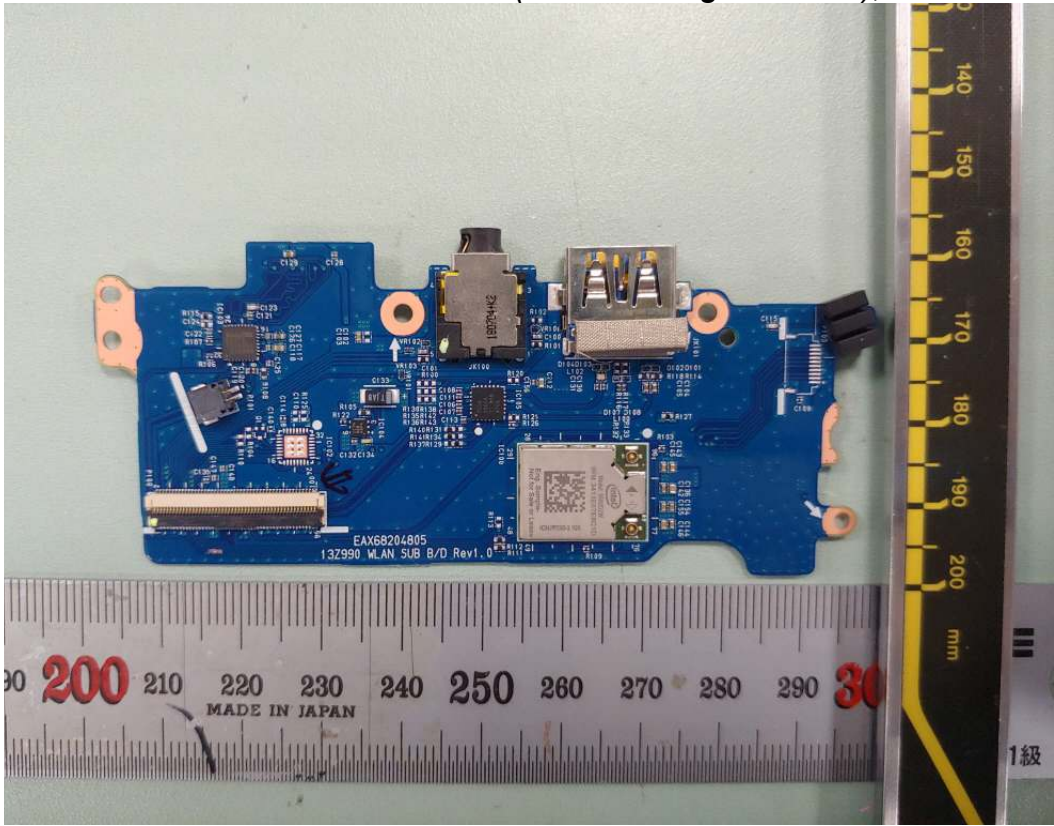
Figure 32 SUB Board (Without Finger Printer), Front View
