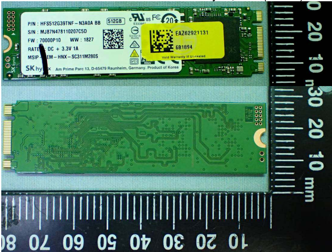
Figure 45 SK hynix, SSD (512GB) View
