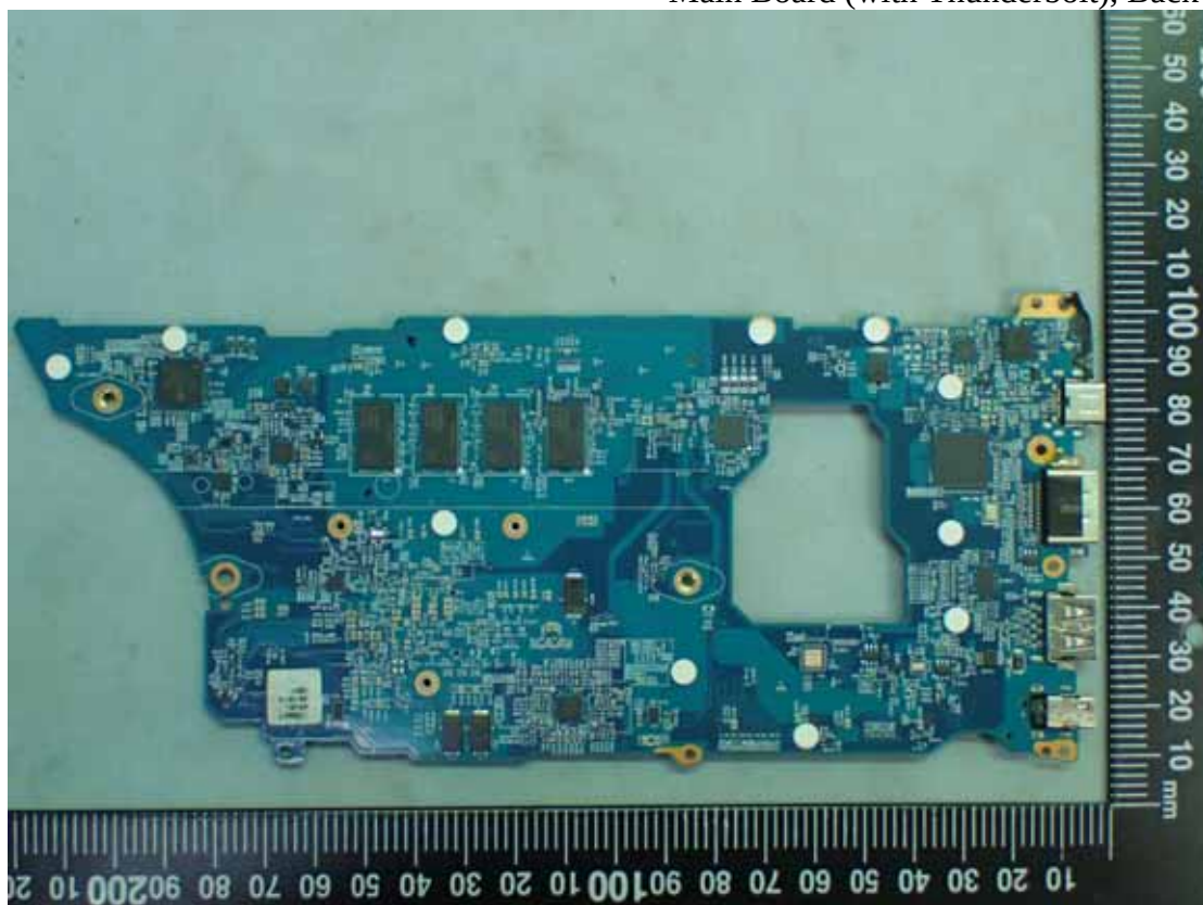
Figure 29 Main Board (with Thunderbolt), Back View
