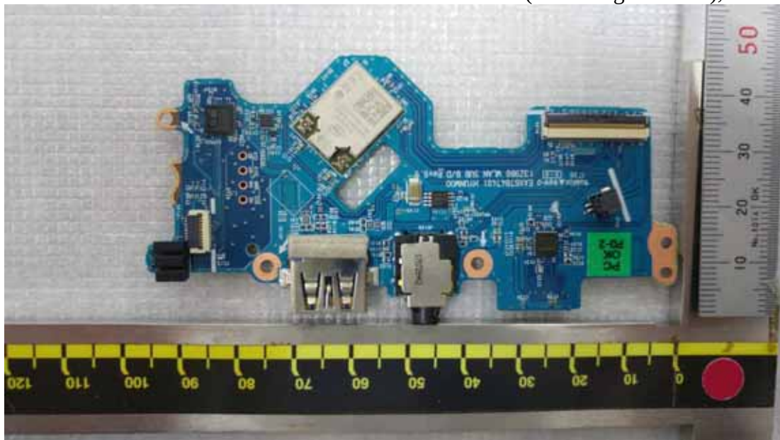
Figure 30 SUB Board (With Finger Printer), Front View
