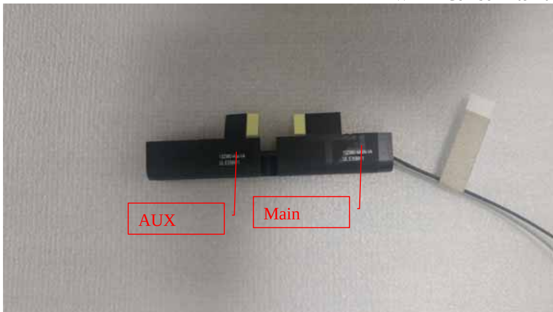
Figure 33 WLAN Combo Antenna View
