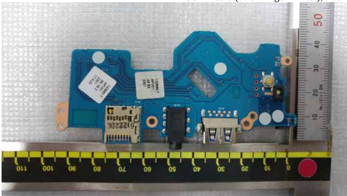
Figure 31 SUB Board (With Finger Printer), Back View
