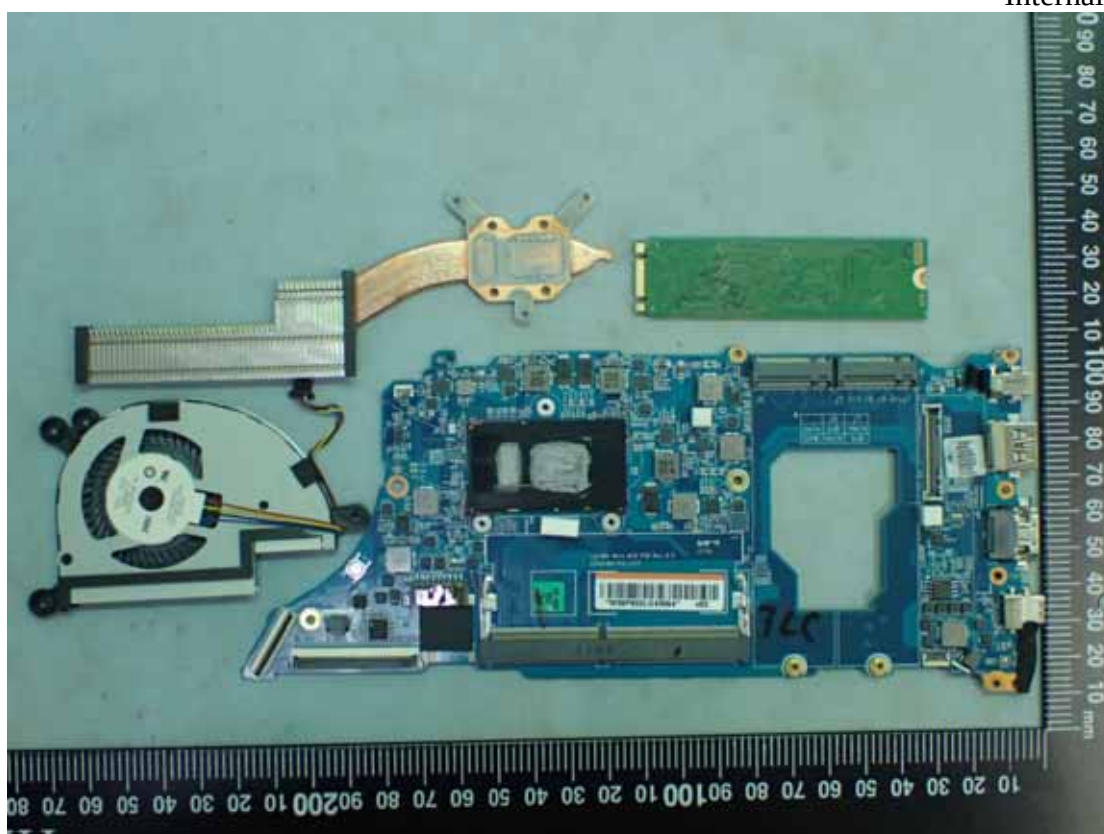
Figure 22 Internal View
