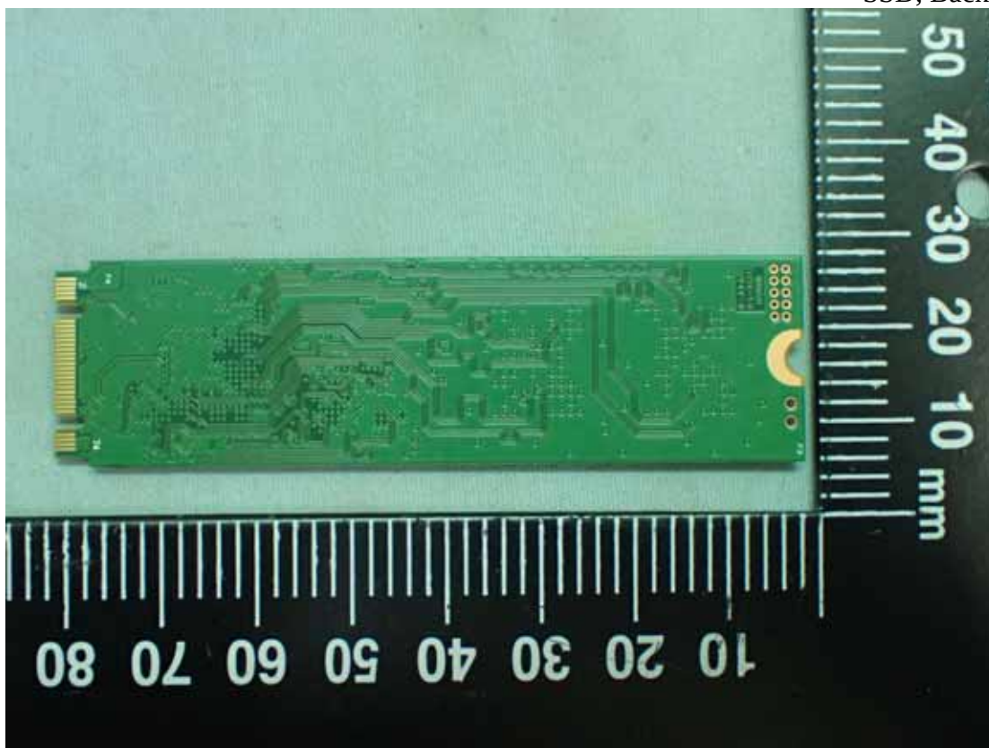
Figure 38 SSD, Back View
