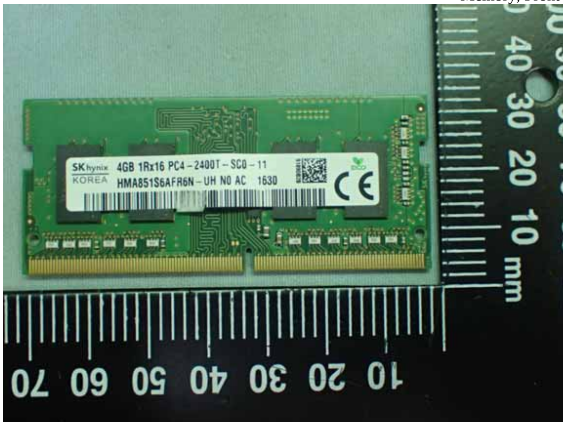
Figure 41 Memory, Front View
