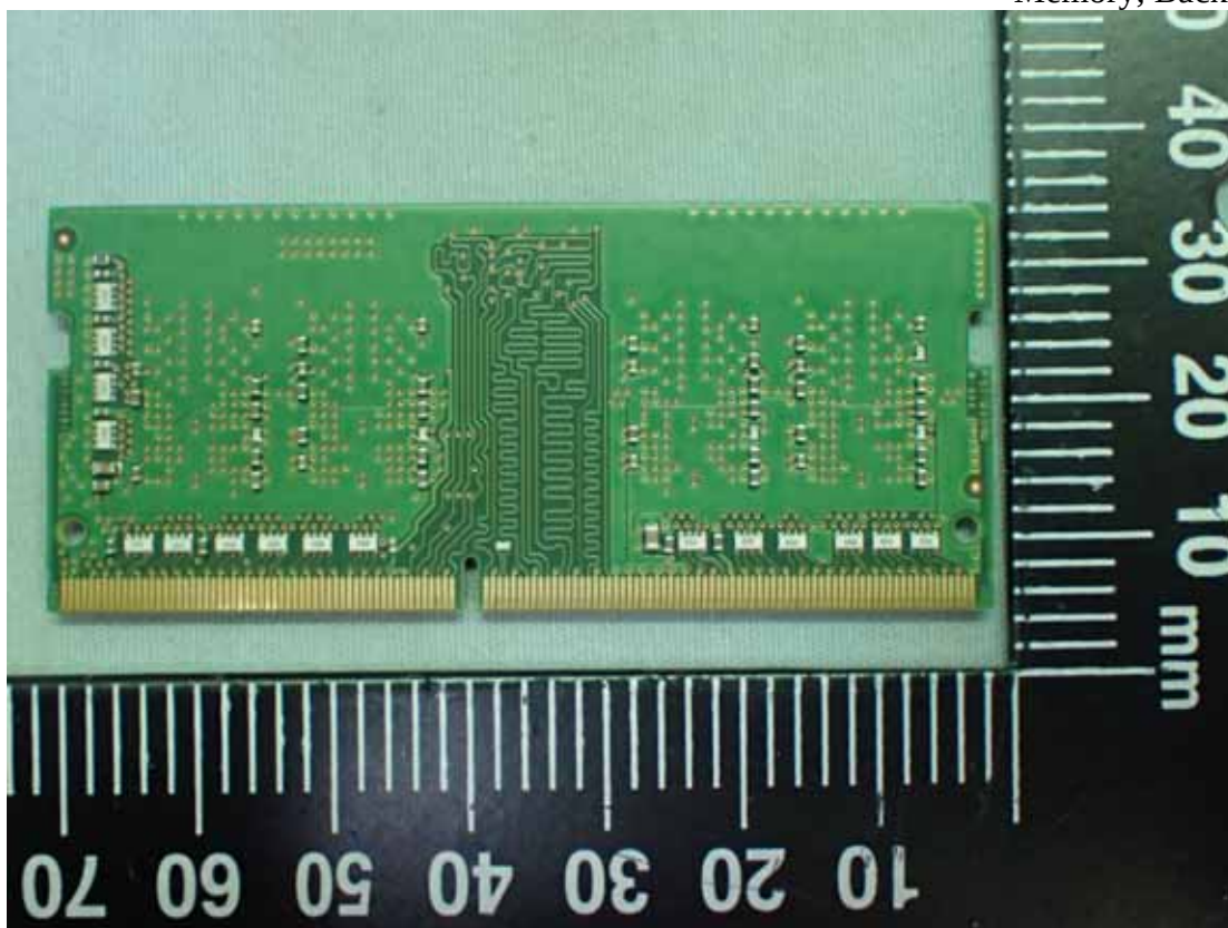
Figure 42 Memory, Back View
