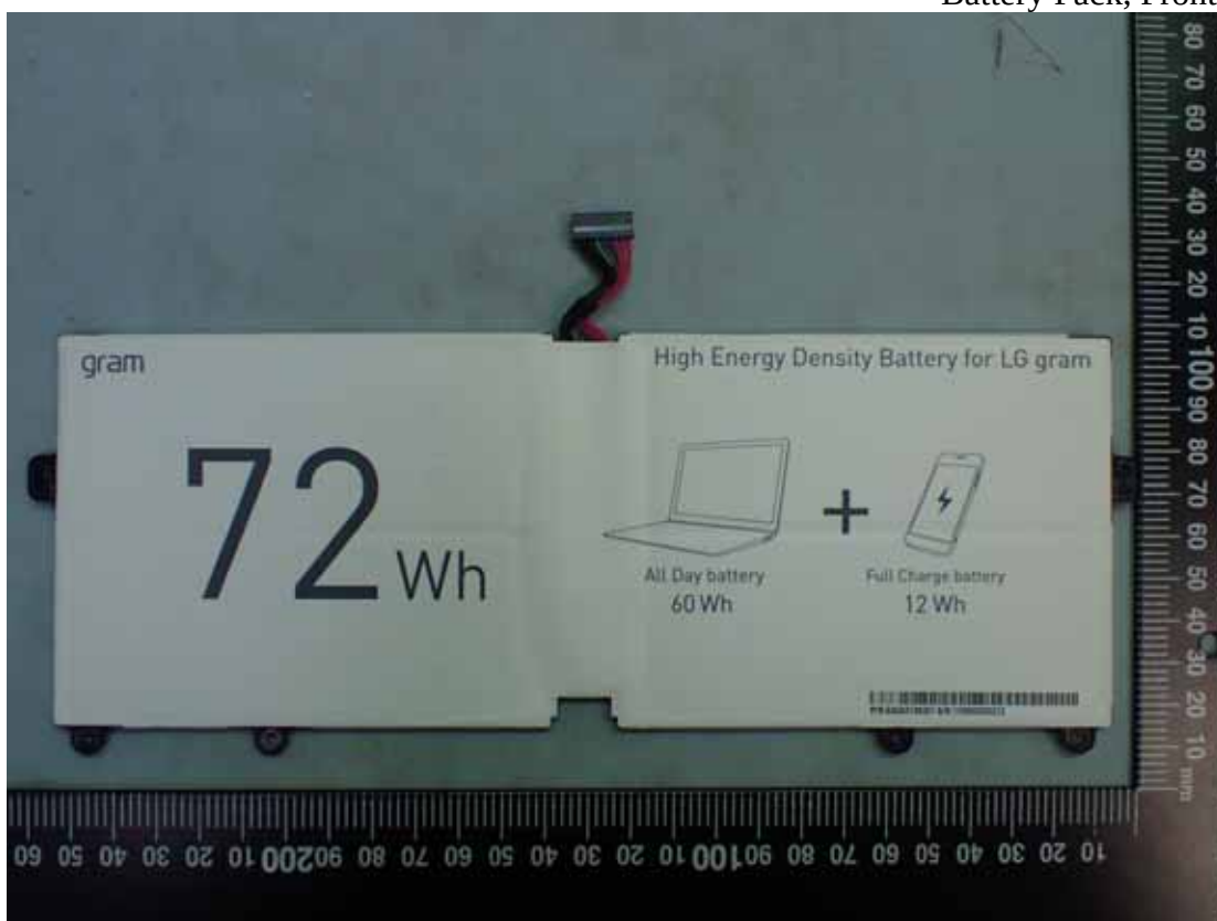
Figure 43 Battery Pack, Front View
