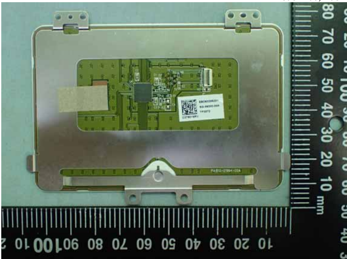
Figure 27 Touch Pad, Back View
