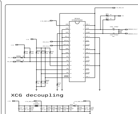
CLOCK Generator
