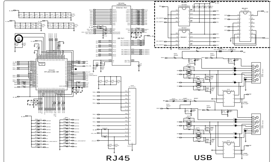
RJ45, USB
