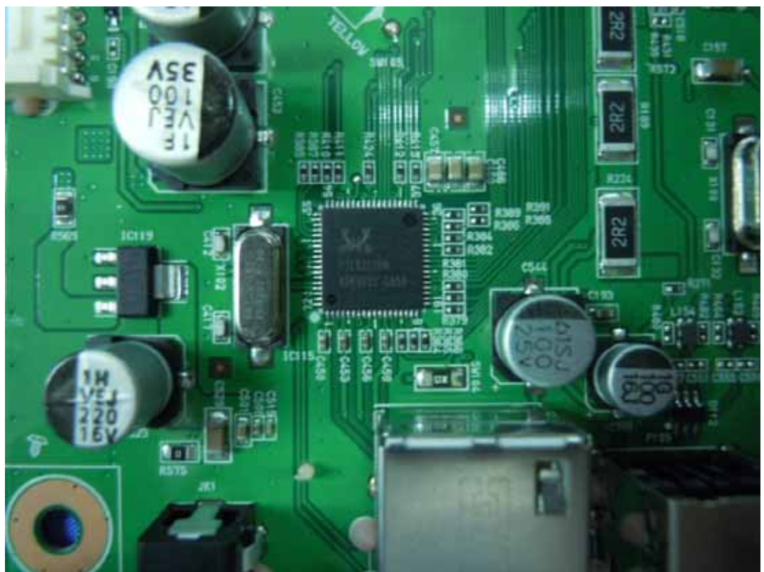
FIGURE 6 LCD MONITOR (M/N: N2210WZT) CHIP #2 & CRYSTAL #2 ON MAIN BOARD
