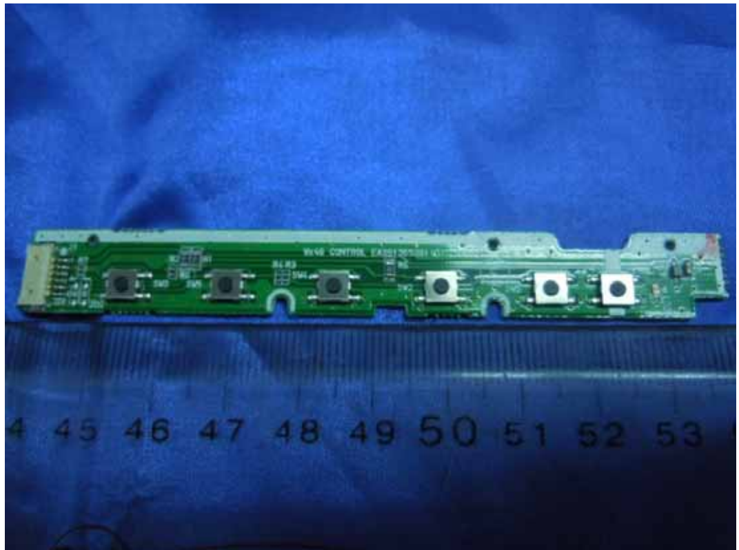
FIGURE 8 LCD MONITOR (M/N: N2210WZT) KEY BOARD (COMPONENT SIDE)
