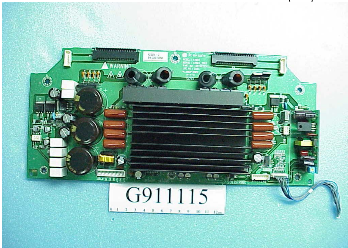
Figure 41 ZSUS-Drive Board (Component Side)
