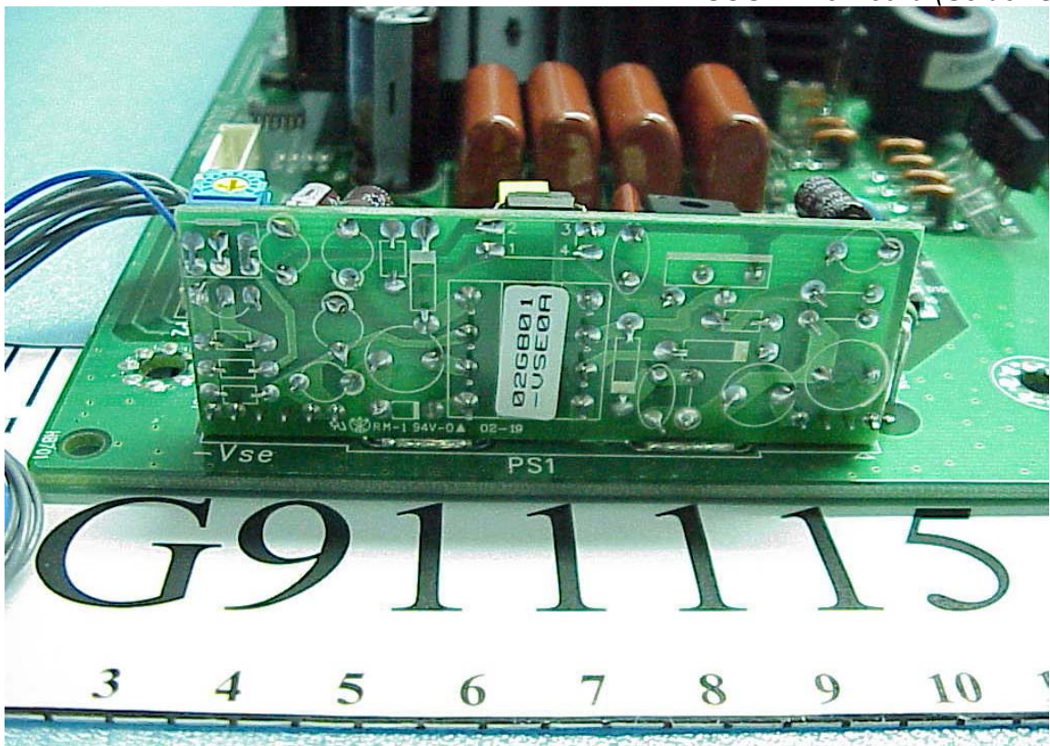
Figure 44 ZSUS-Drive Board (Solder Side)
