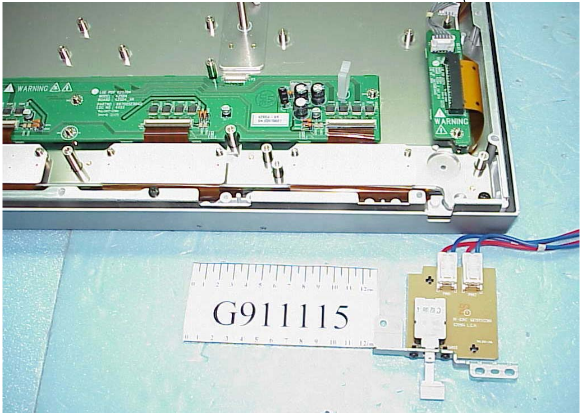
Figure 45 Frame of Internal (Remove SW Board)
