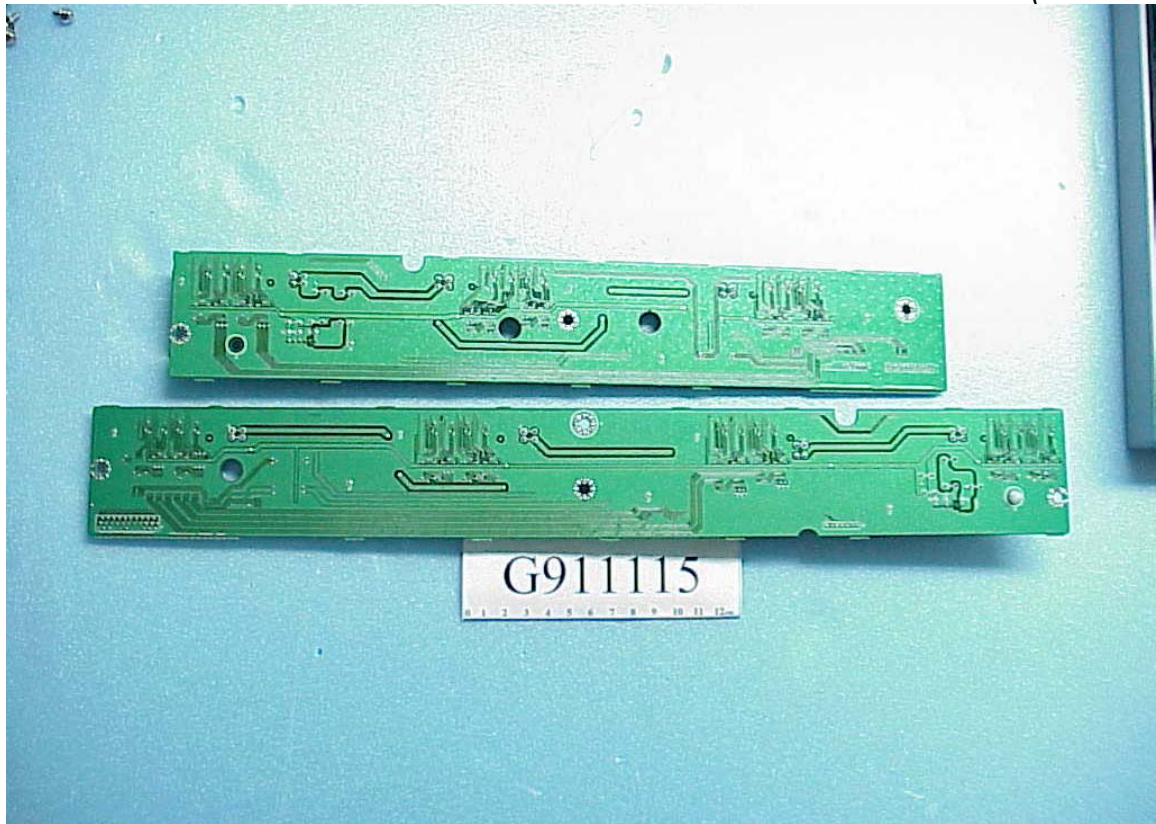
Figure 53 XL/XR-Drive Board (Solder Side)
