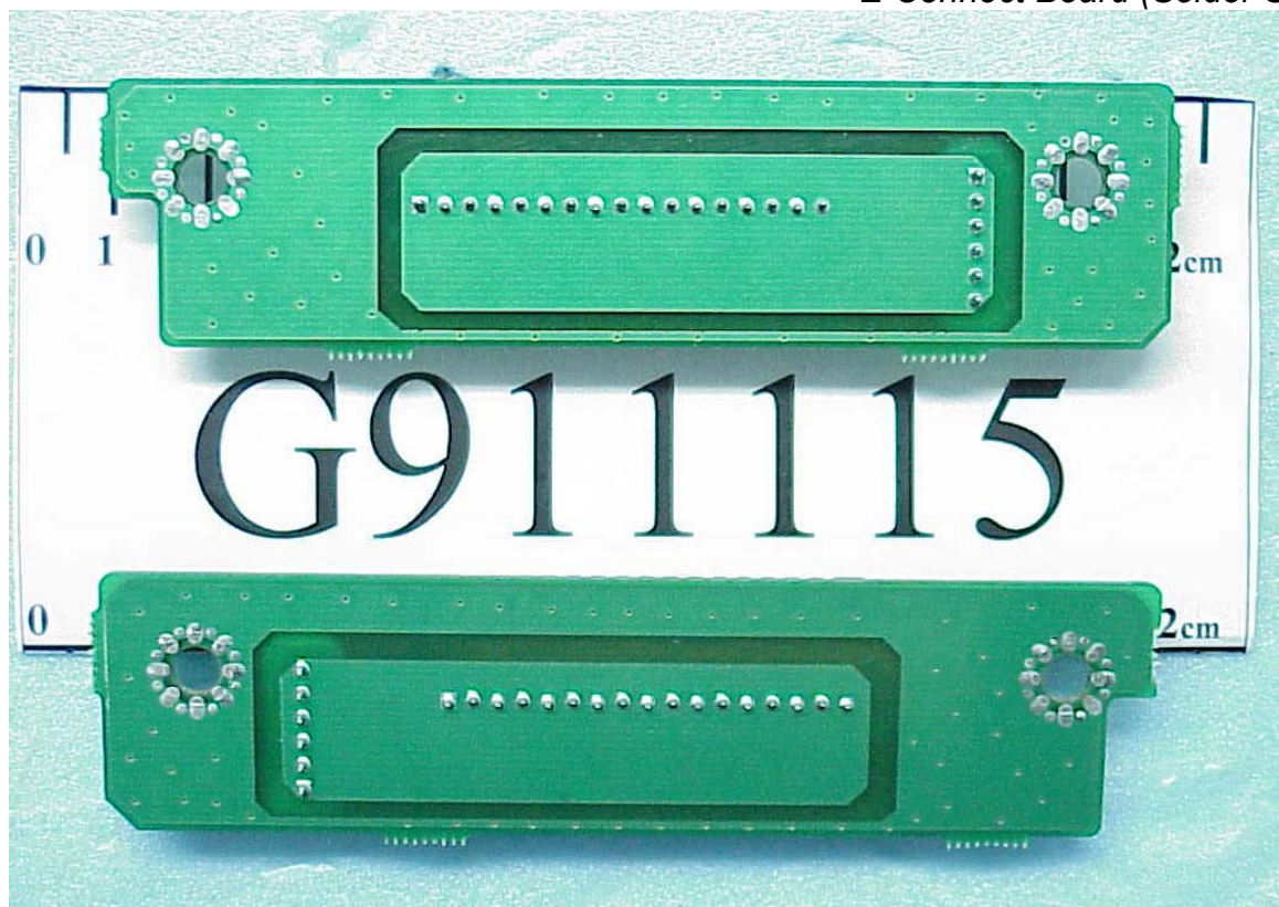
Figure 50 Z-Connect Board (Solder Side)
