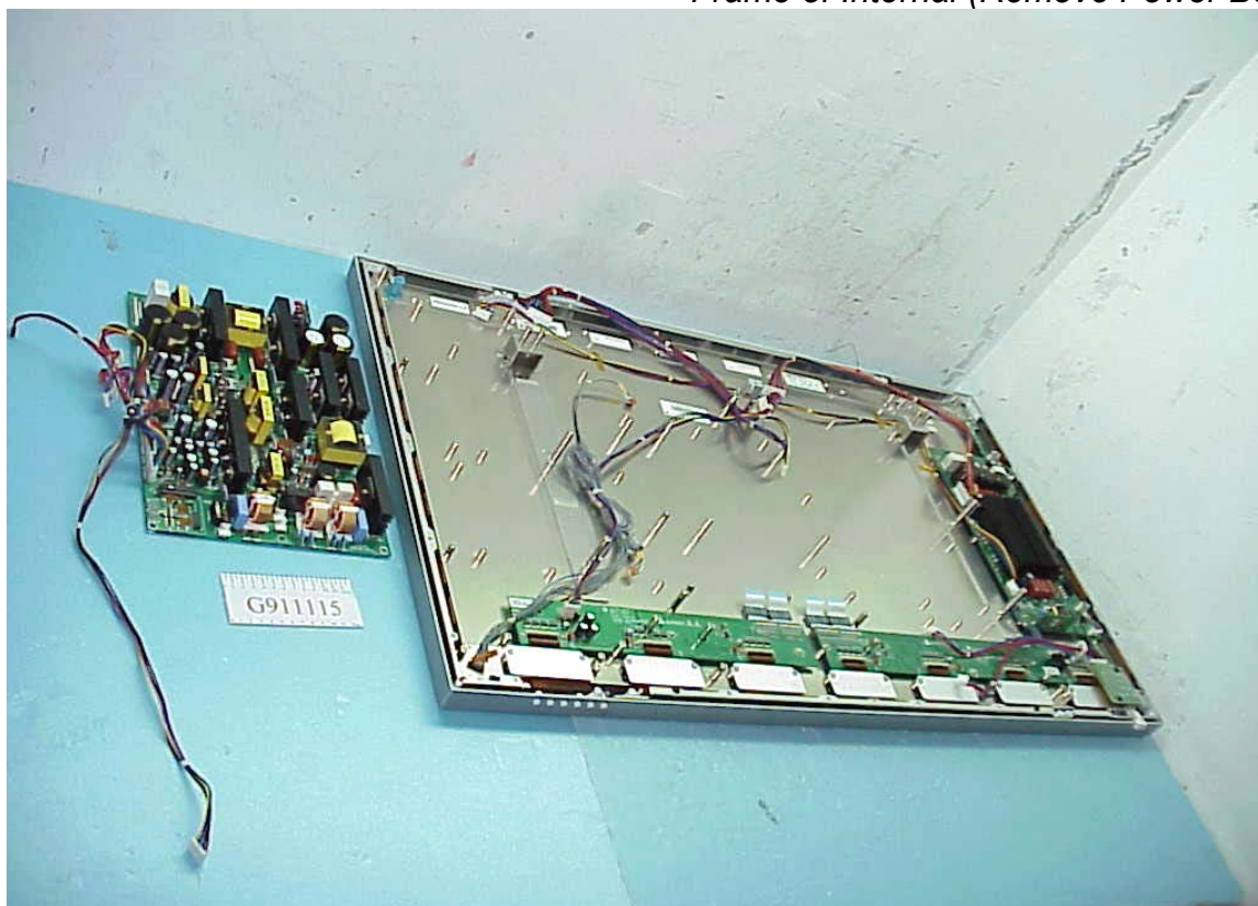
Figure 37 Frame of Internal (Remove Power Board)
