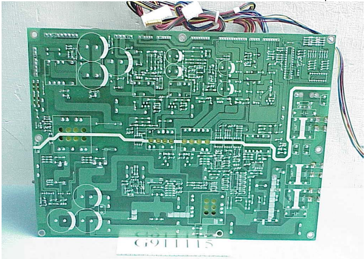
Figure 39 Power Board (Solder Side)
