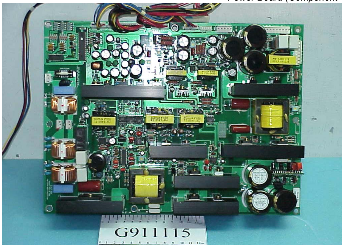
Figure 38 Power Board (Component Side)
