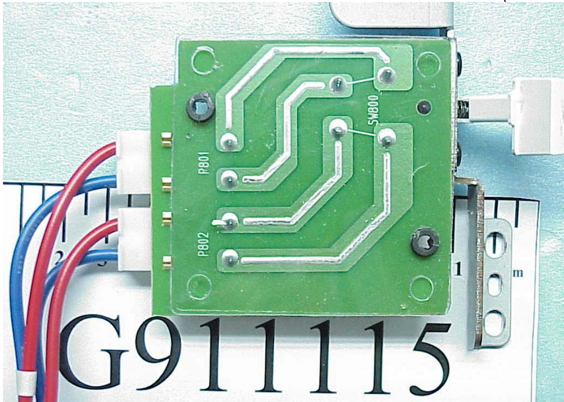
Figure 47 SW Board (Solder Side)
