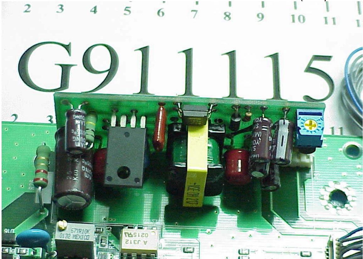
Figure 43 ZSUS-Drive Board (Component Side)
