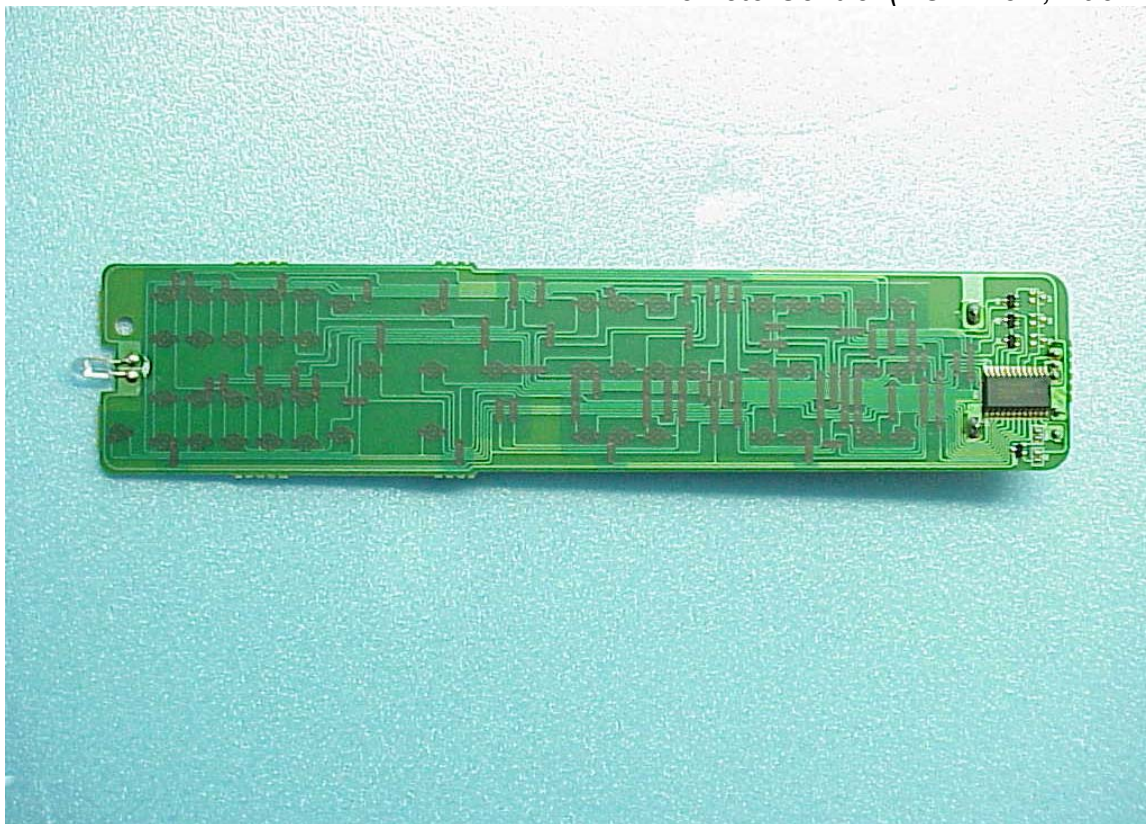
Figure 65 Remote Control (PCB View, Back Side)
