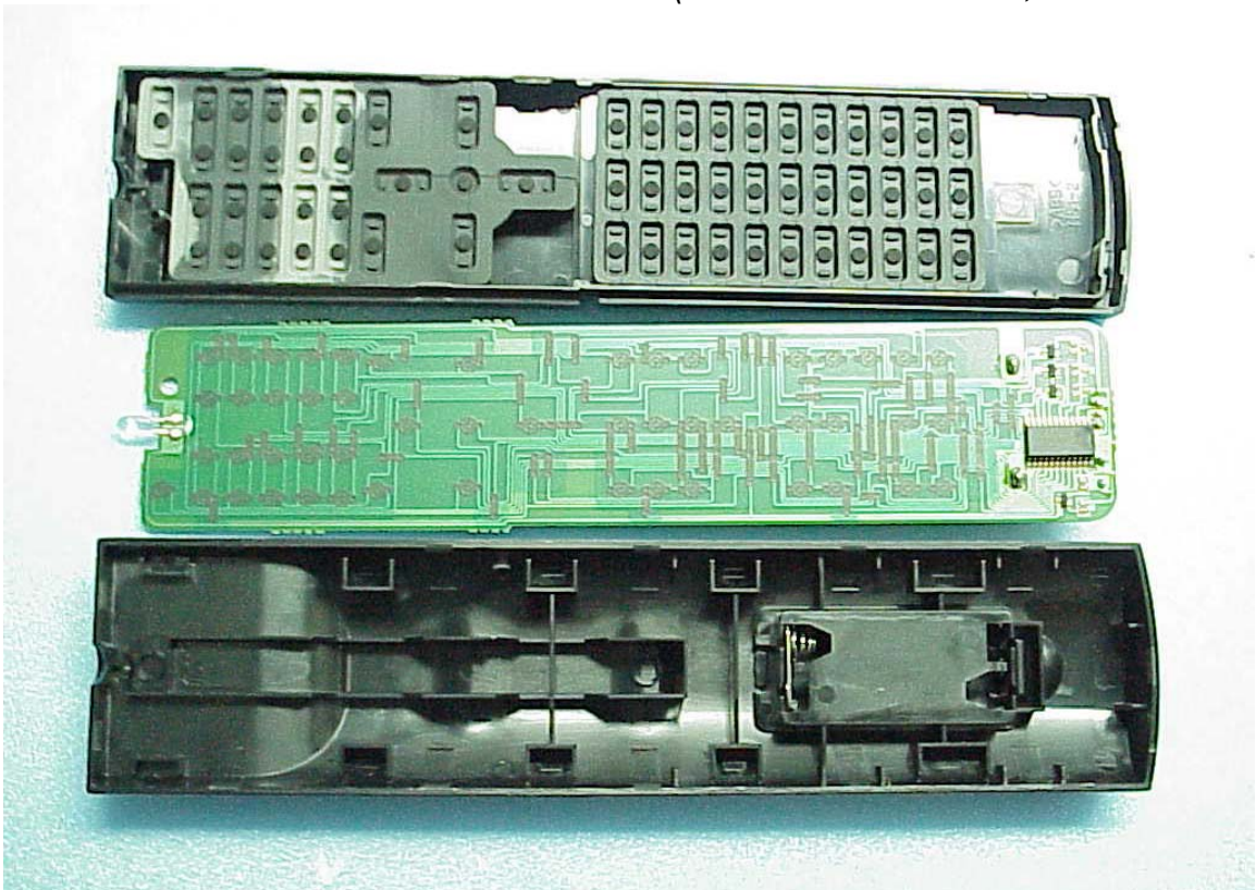
Figure 64 Remote Control (Remove Case Covers, Frame of Internal)
