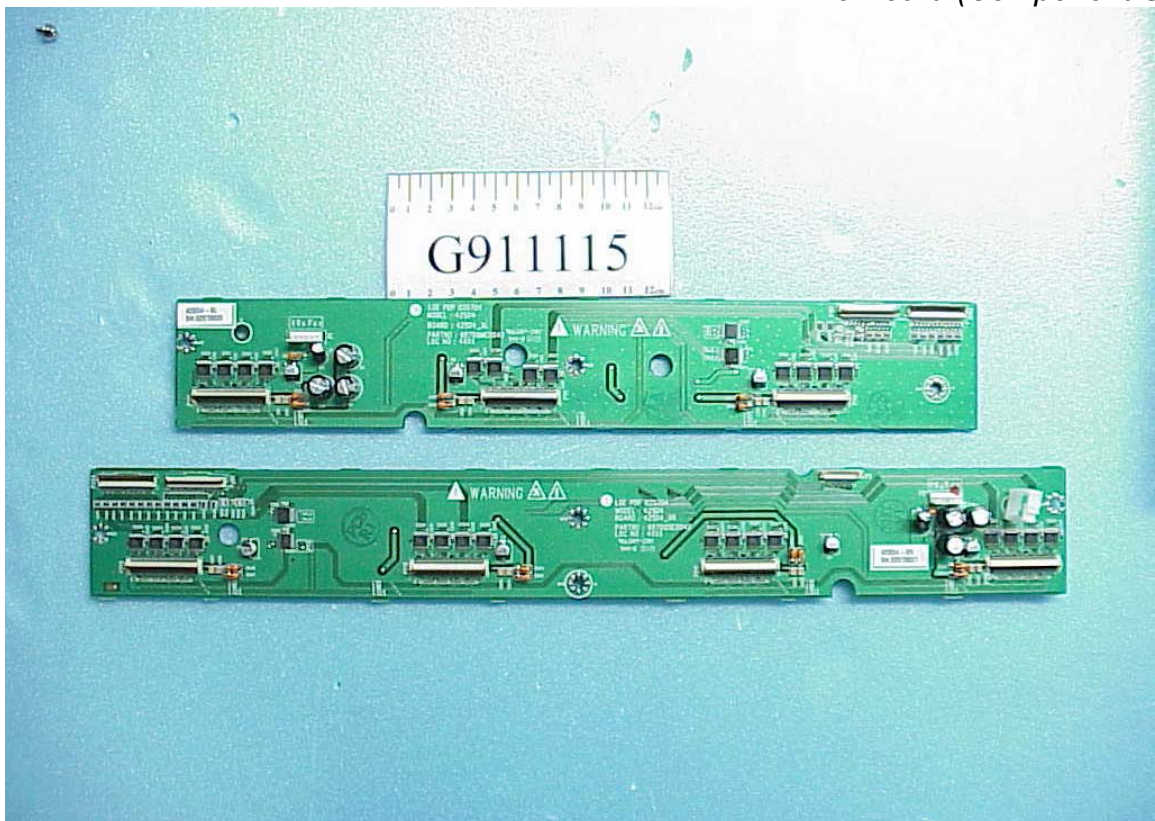
Figure 52 XL/XR-Drive Board (Component Side)
