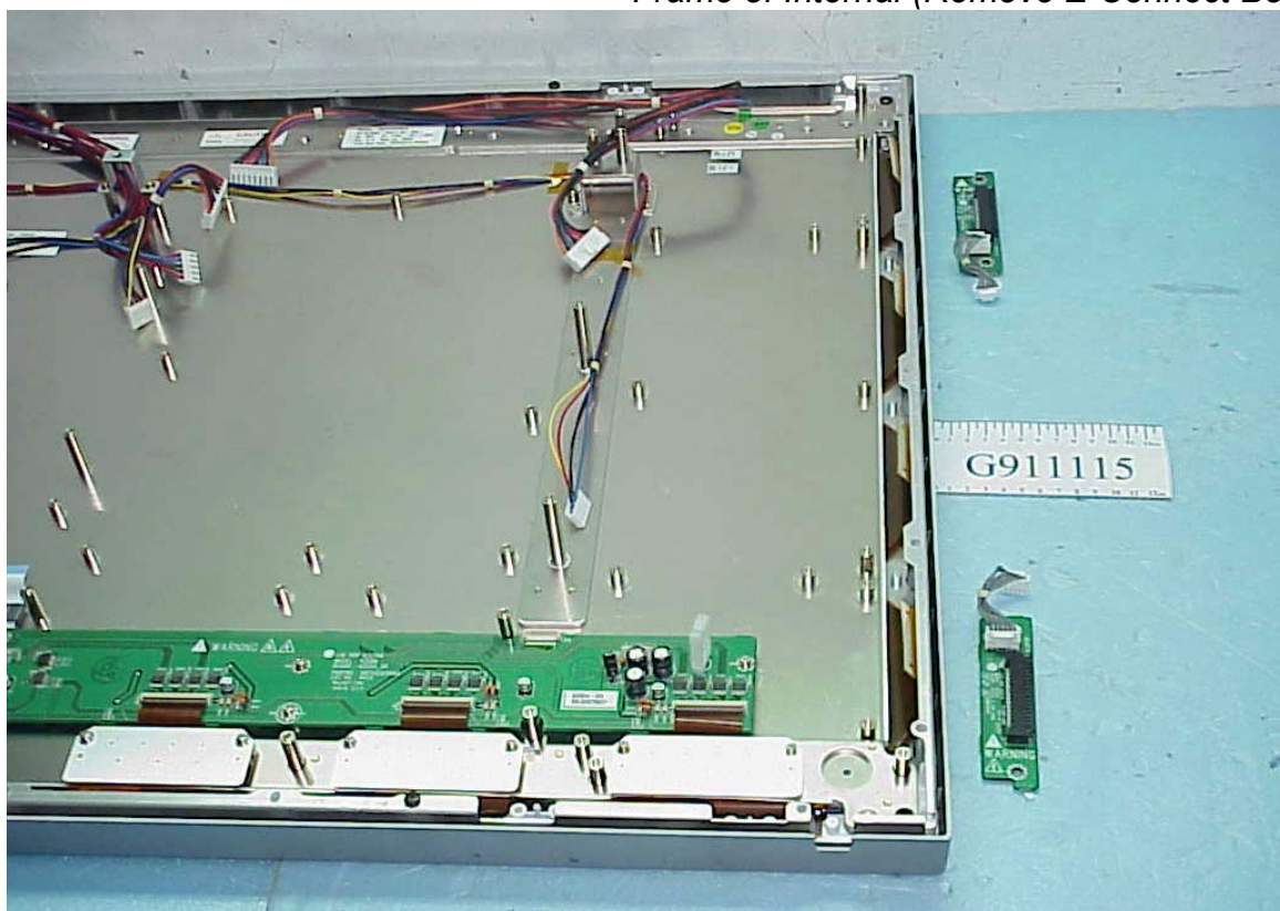
Figure 48 Frame of Internal (Remove Z-Connect Board)
