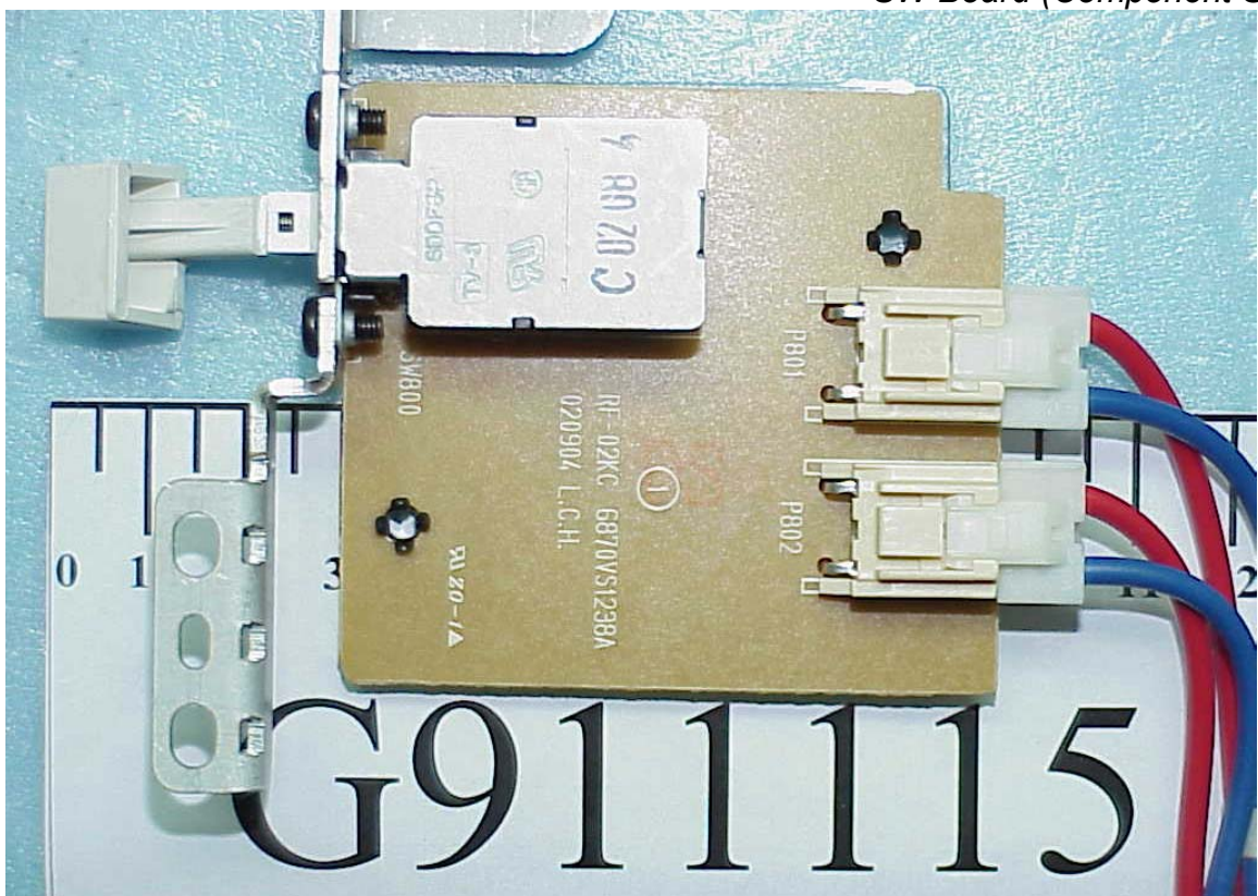
Figure 46 SW Board (Component Side)
