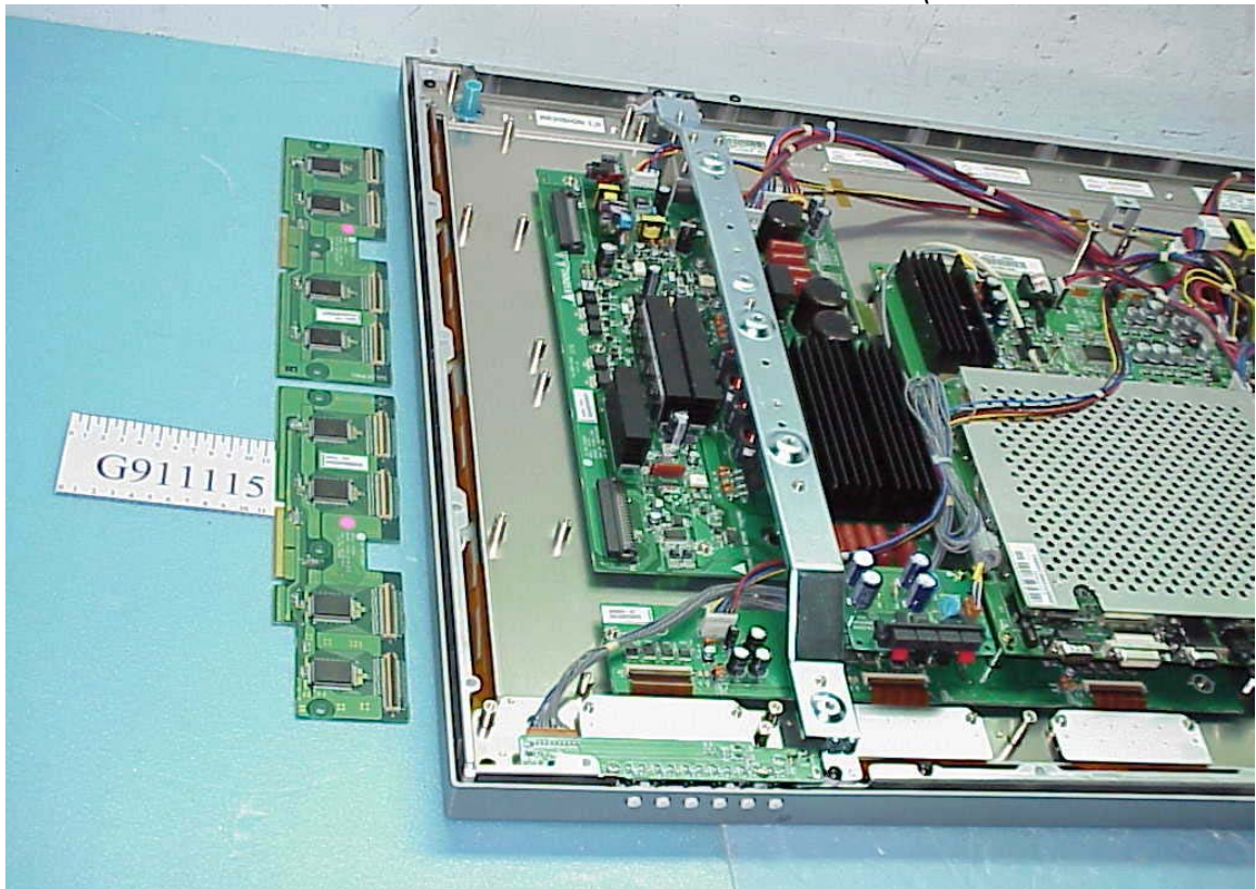
Figure 12 Frame of Internal (Removed Y-Drive Board)
