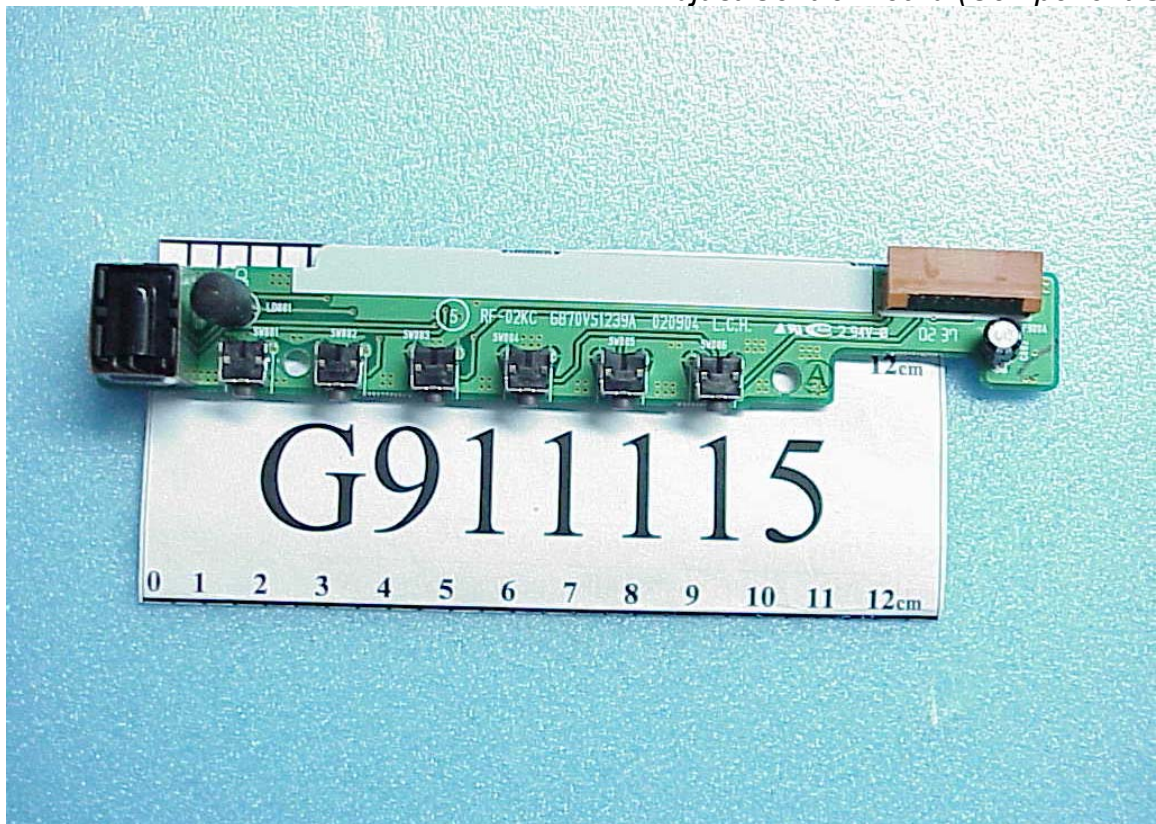
Figure 15 Adjust Control Board (Component Side)
