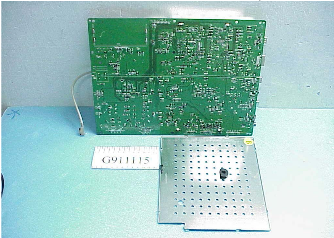
Figure 25 Main Board (Remove Metal Cover)
