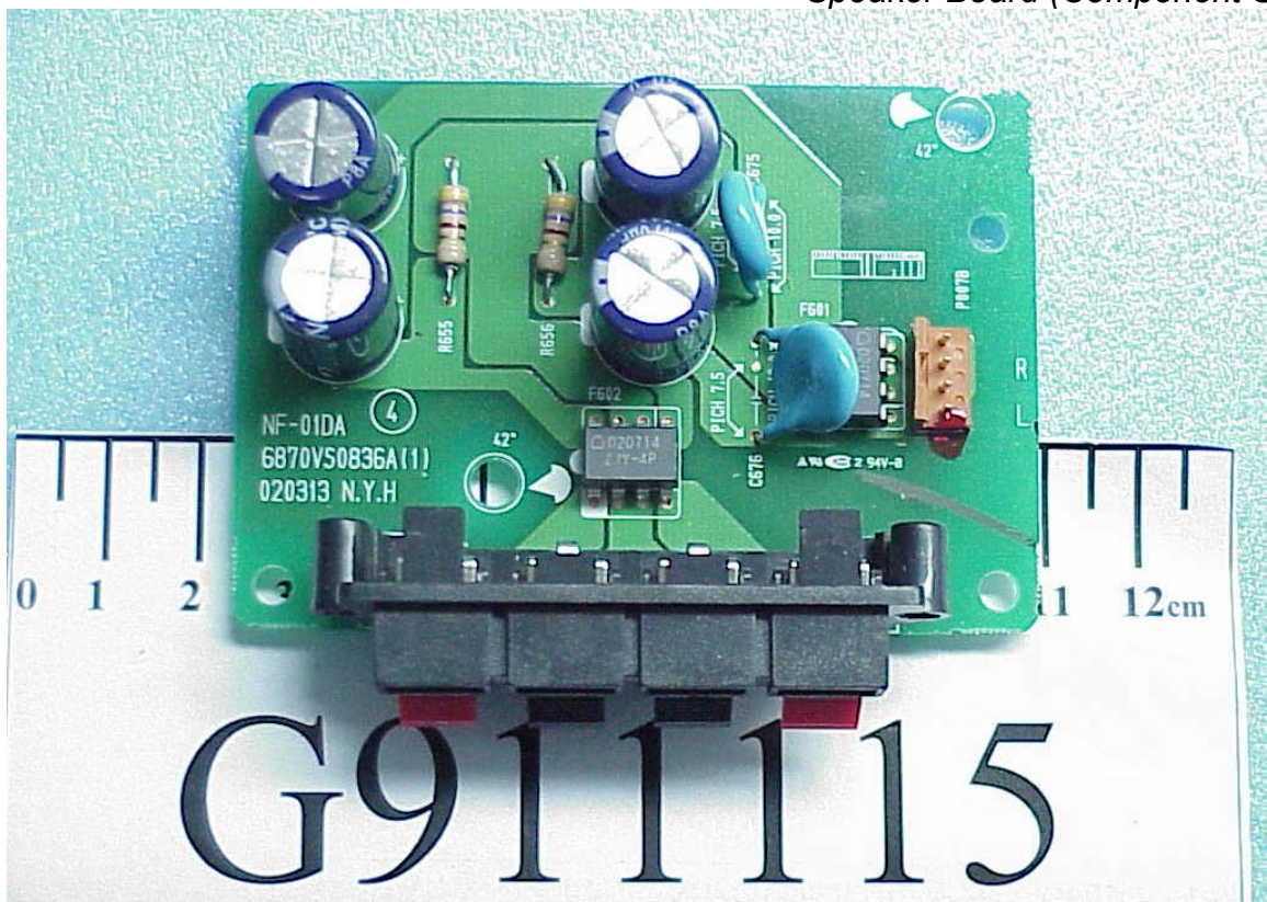
Figure 20 Speaker Board (Component Side)
