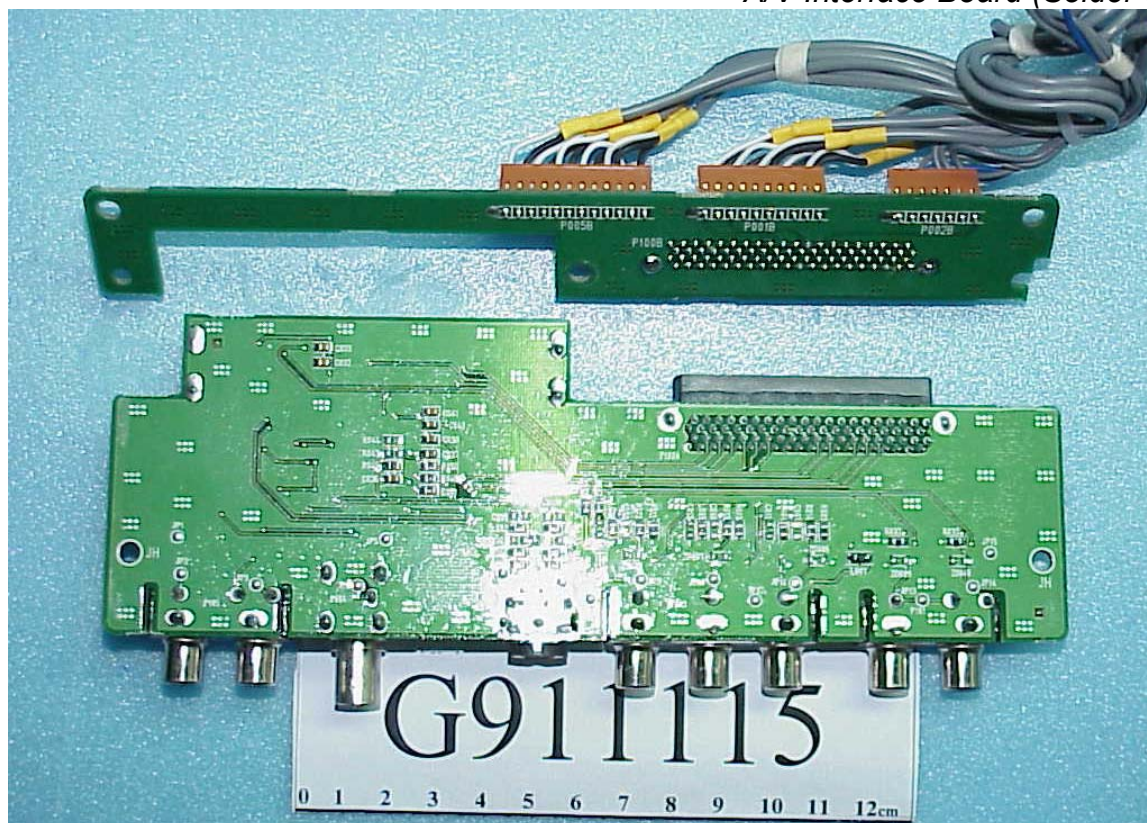
Figure 36 A/V Interface Board (Solder Side)
