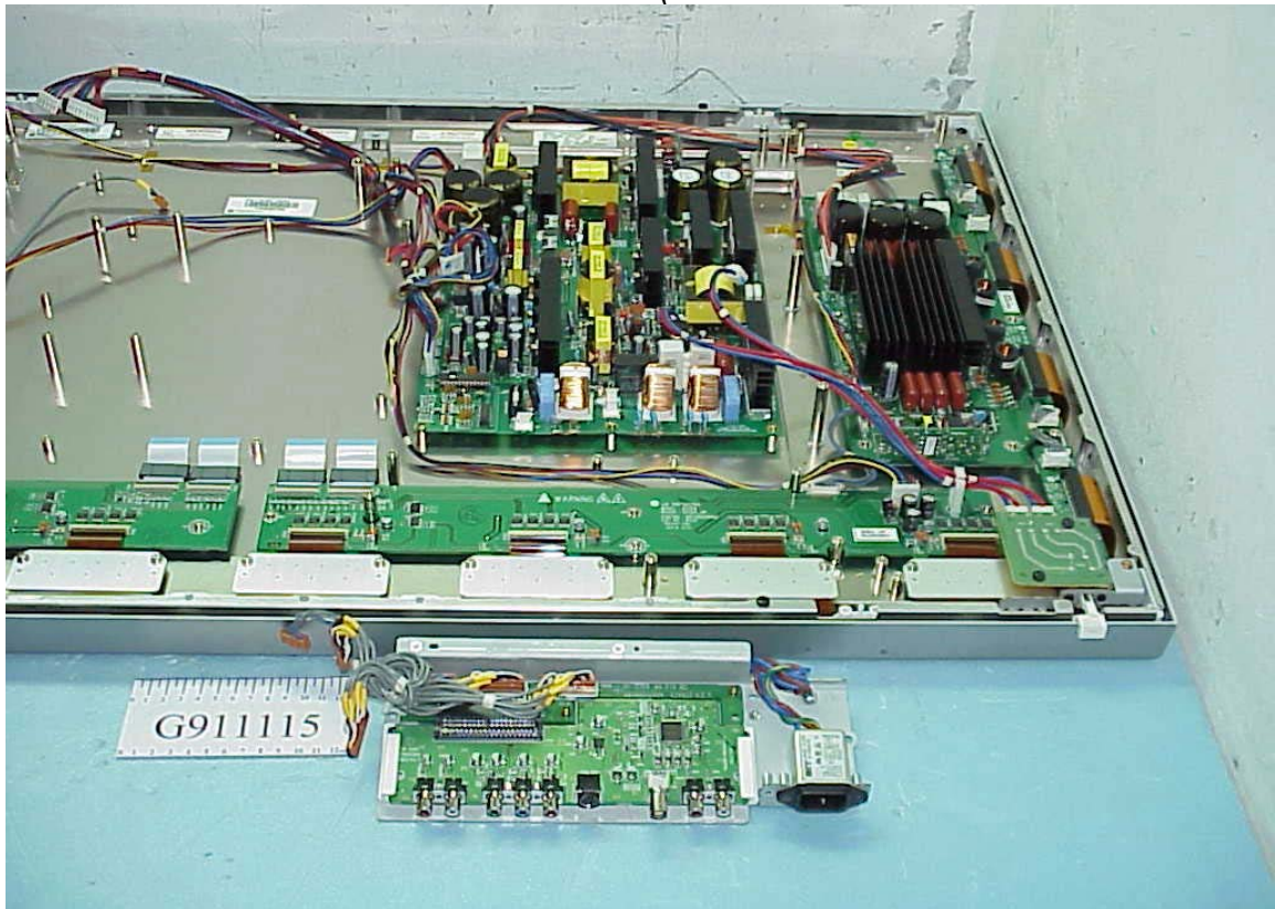
Figure 33 Frame of Internal (Remove A/V Interface Board & AC Socket)
