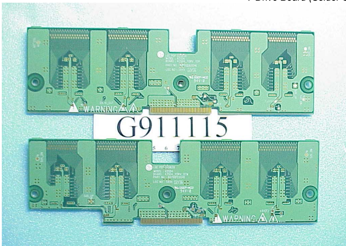
Figure 14 Y-Drive Board (Solder Side)
