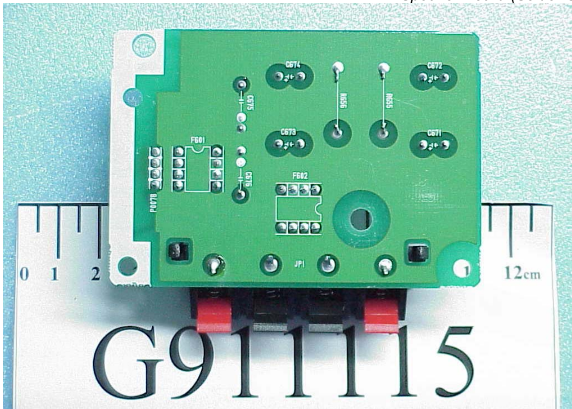
Figure 21 Speaker Board (Solder Side)
