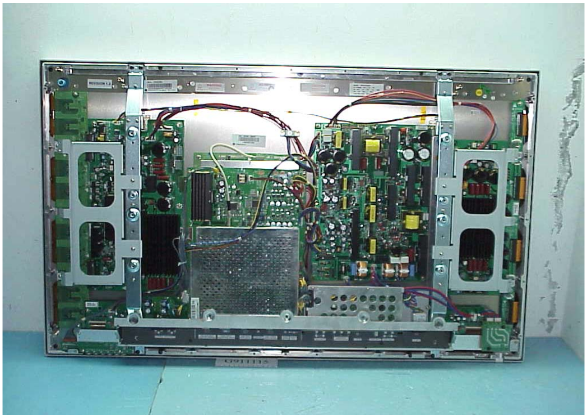
Figure 8 Frame of Internal
