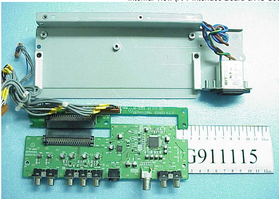
Figure 34 Internal View (A/V Interface Board & AC Socket)
