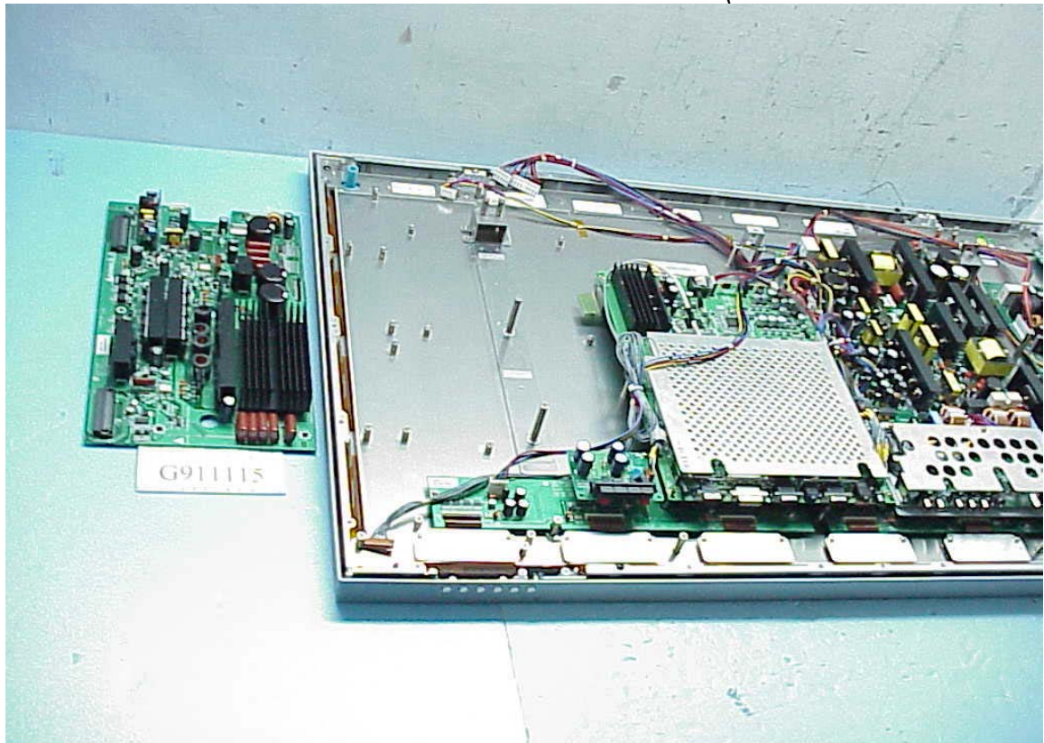
Figure 17 Frame of Internal (Remove ZSUS-Drive Board)
