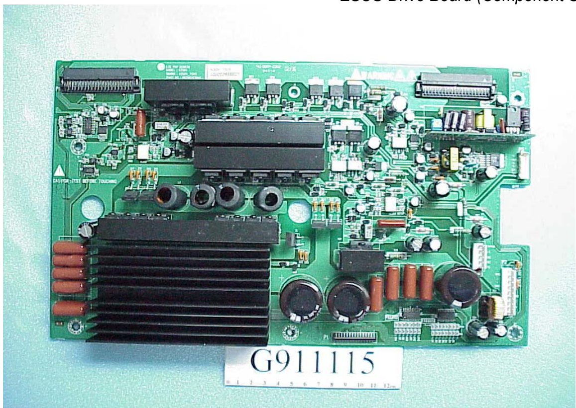
Figure 18 ZSUS-Drive Board (Component Side)
