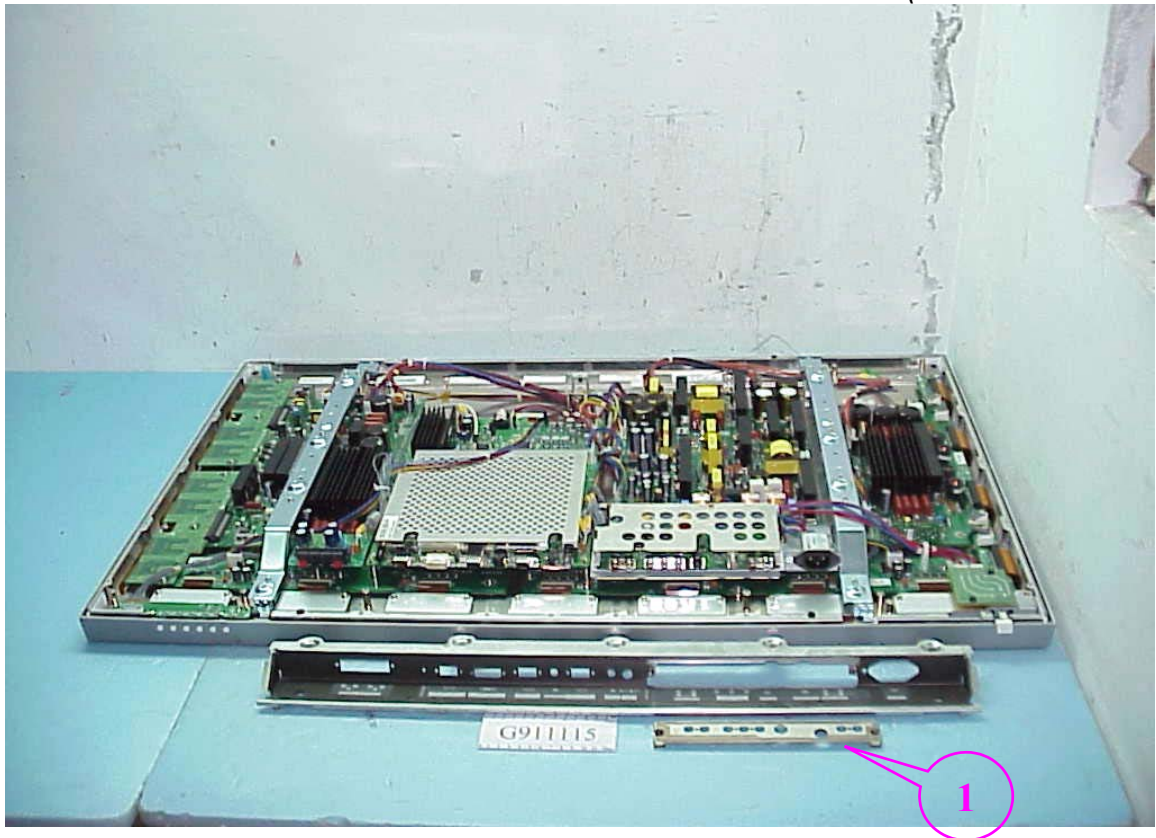
Figure 12 Frame of Internal (Removed Y-Drive Board)
