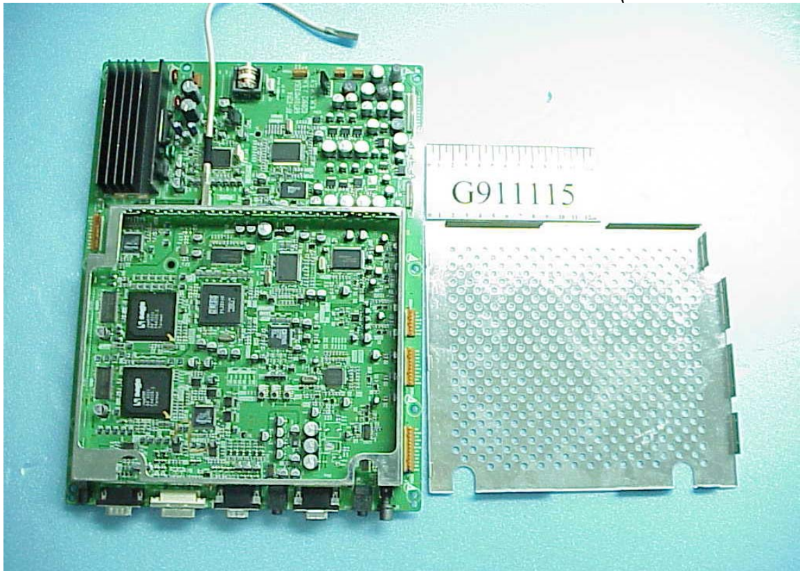
Figure 23 Main Board Board (Remove Metal Cover)
