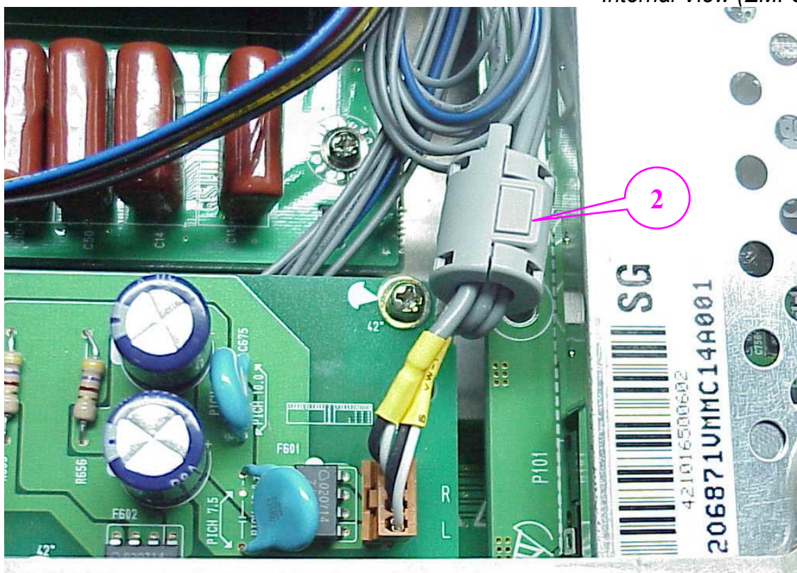
Figure 10 Internal View (EMI Core)
