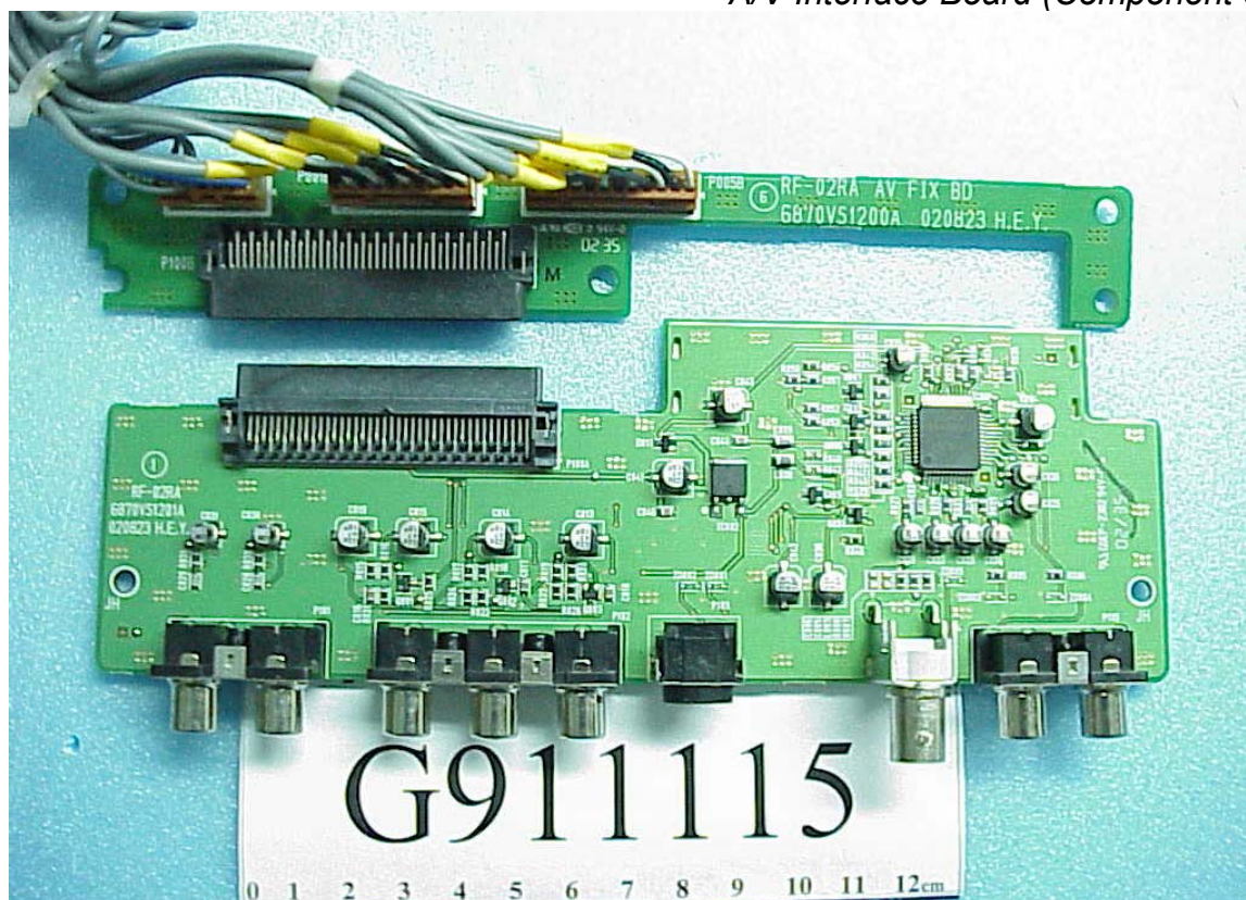
Figure 35 A/V Interface Board (Component Side)
