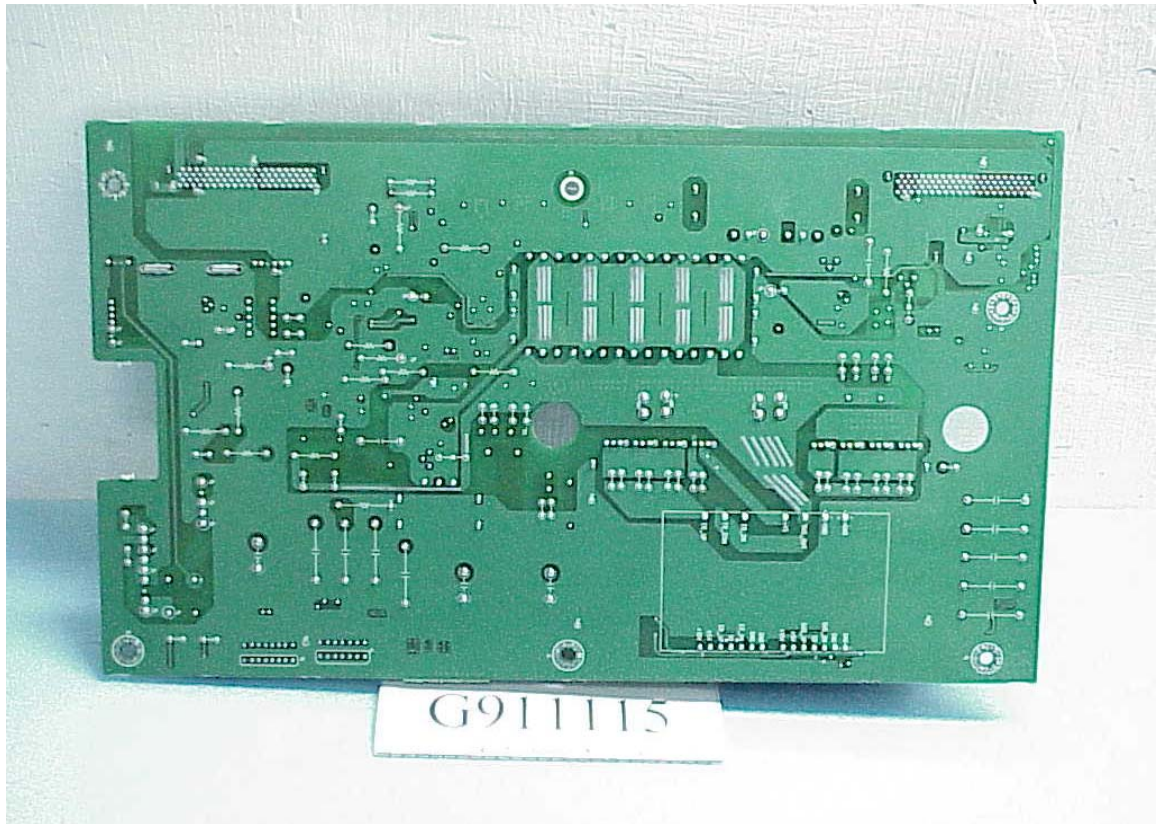
Figure 19 ZSUS-Drive Board (Solder Side)
