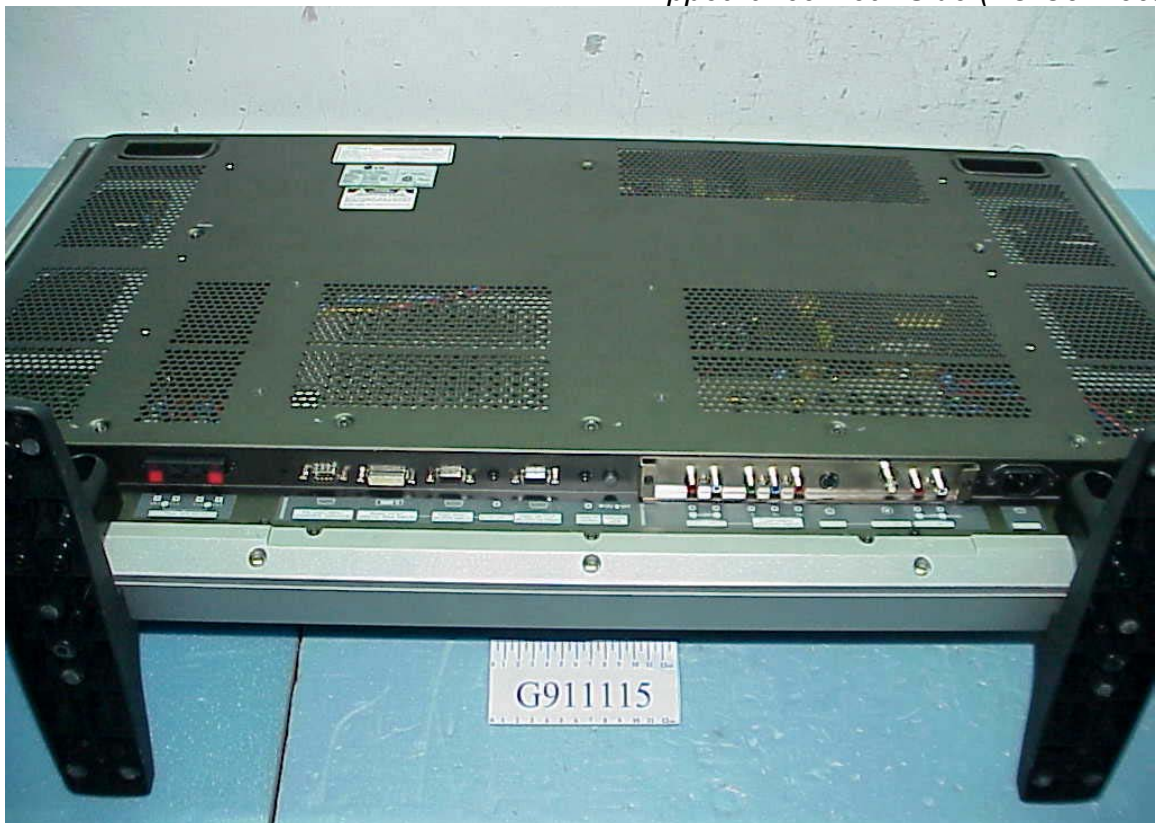
Figure 6 Appearance/Rear Side (I/O Connectors)
