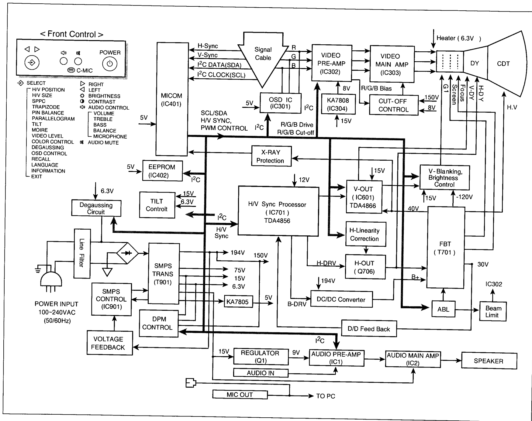
BLOCK DIAGRAM
