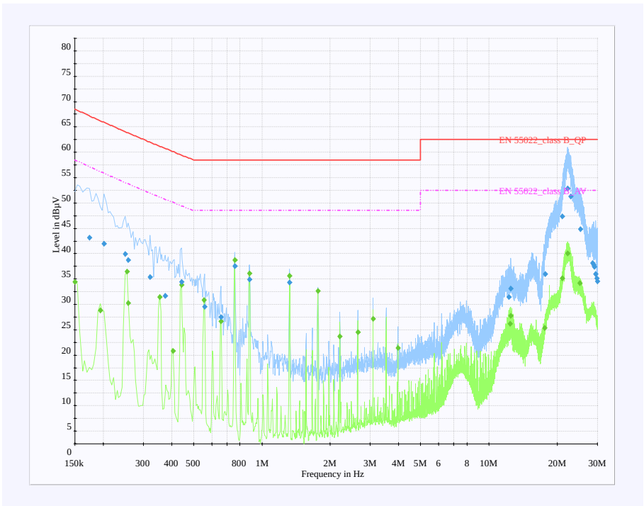
< Neutral line >
