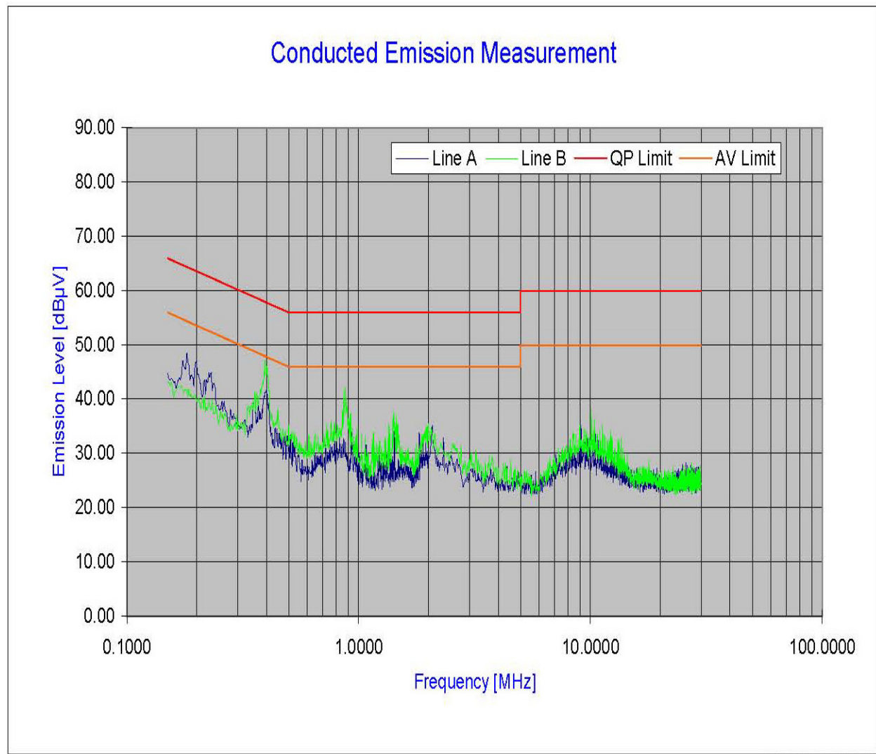
Plot 6-16. Line Conducted Plot with Bluetooth
