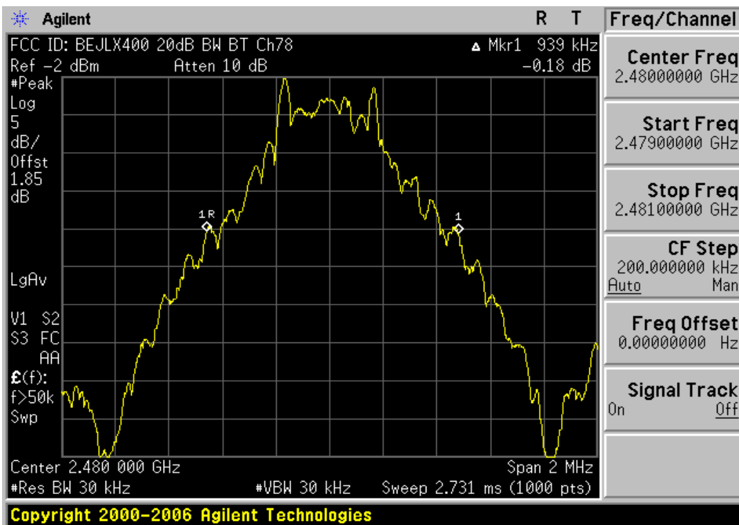
Plot 6-3. 20dB Bandwidth Plot (Bluetooth – Ch. 78)
