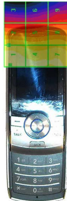
Figure 17-5 H-Field WD Scan overlay
