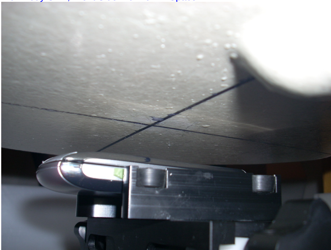
10. Body SAR, Front Side with 20mm Space
