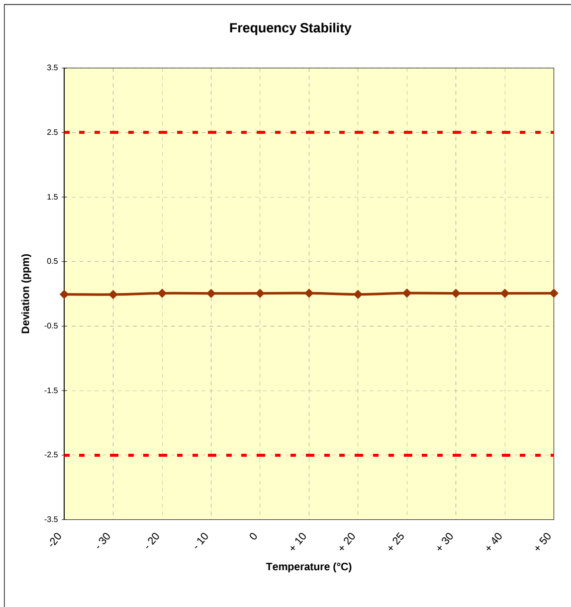
Figure 6-2. Frequency Stability Graph (PCS CDMA Mode – Ch. 600)
