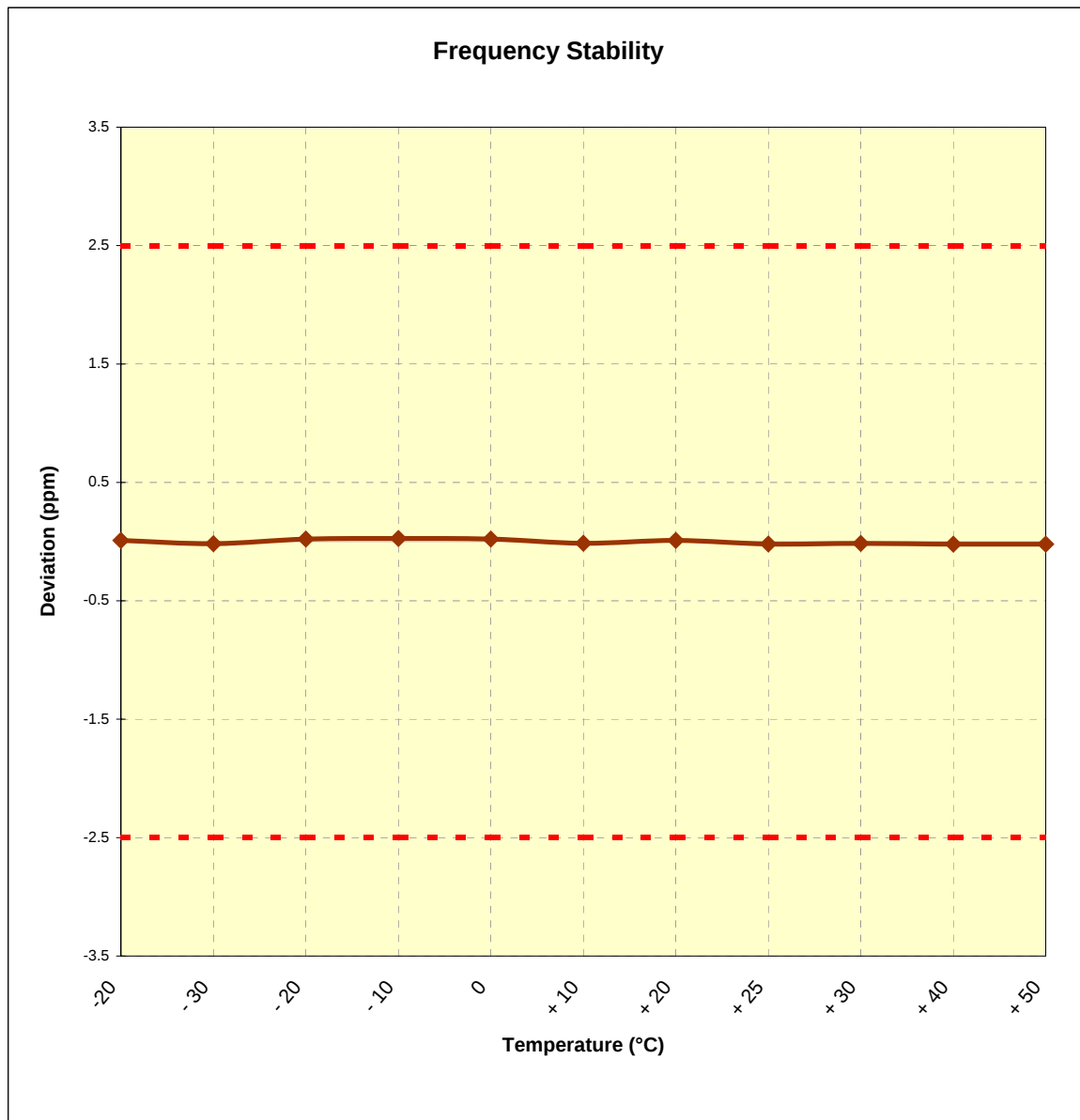
Figure 6-1. Frequency Stability Graph (Cellular CDMA Mode – Ch. 384)
