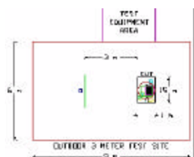
Figure 3-2. Dimensions of Outdoor Test Site
