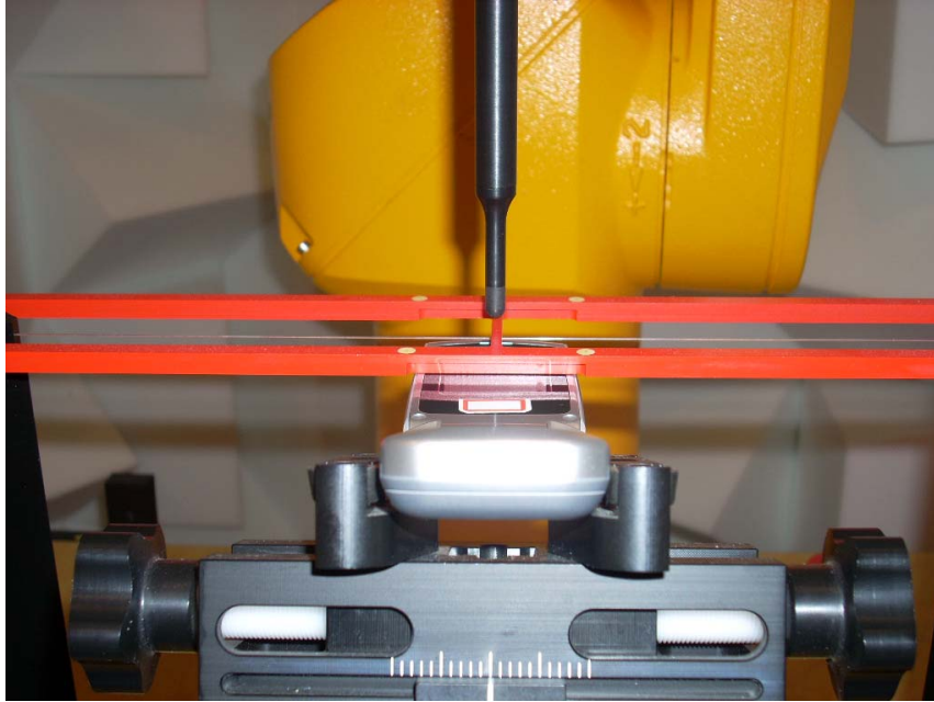
Figure 16-1 Ear Reference Point HAC Phantom Alignment
