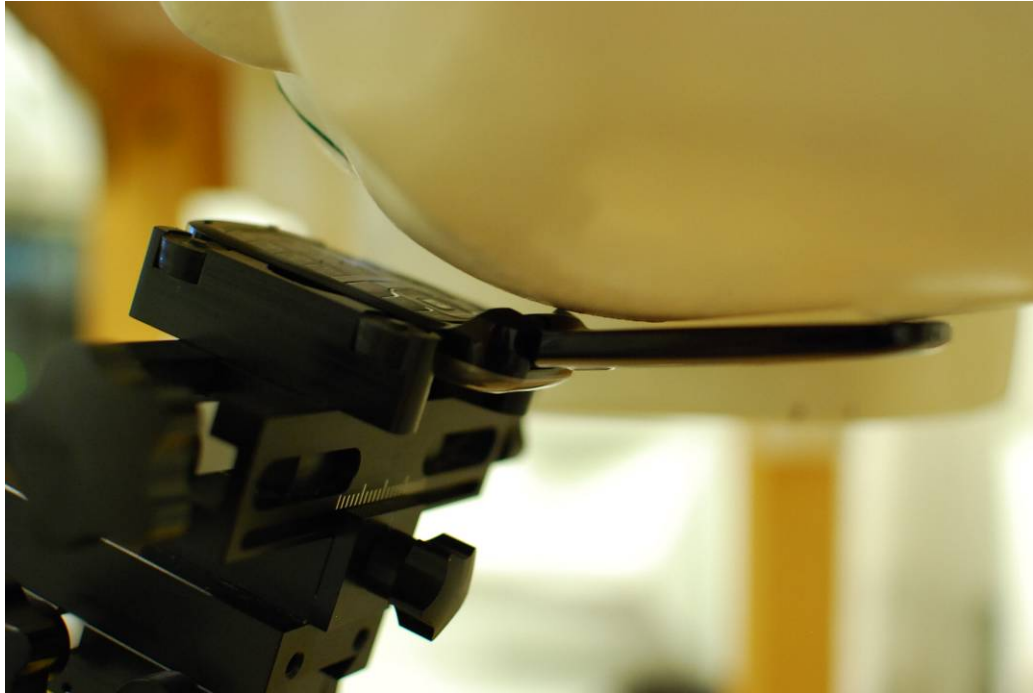
Figure 19-3 SAR Test Setup Photo 3
