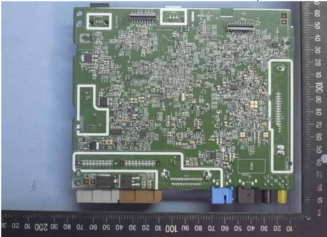
Figure 6 Internal View (Main Board, Back View)
