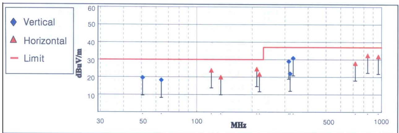
< Fig 4. Radiated Emission _ Analog(30MHz ~ 1000MHz) >
