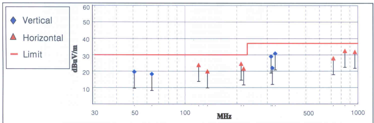
< Fig 6. Radiated Emission _ Digital(30MHz ~ 1000MHz) >
