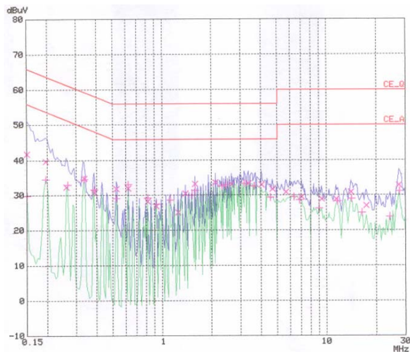
< Neutral line >
