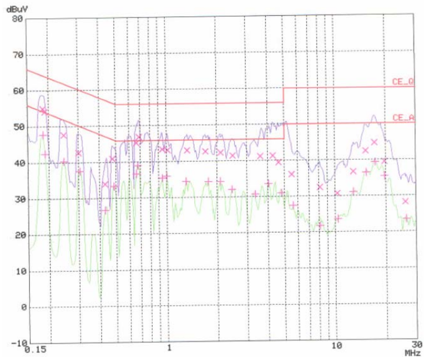
< Neutral line >
