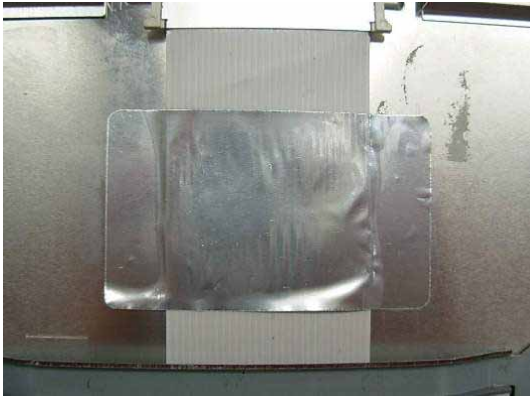
FIGURE 17 LCD MONITOR (M/N: L1942PQT) DEBUG 1
