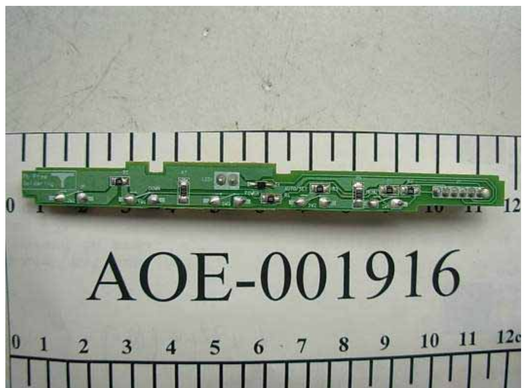
FIGURE 4 LCD MONITOR (M/N: L1942PQT) KEY BOARD (SOLDERED SIDE)
