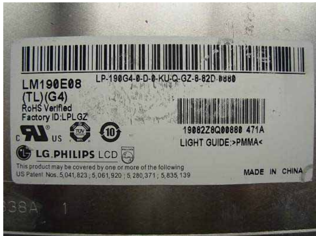
FIGURE 11 LCD MONITOR (M/N: L1942PQT) LABEL 1 ON LCD PANEL
