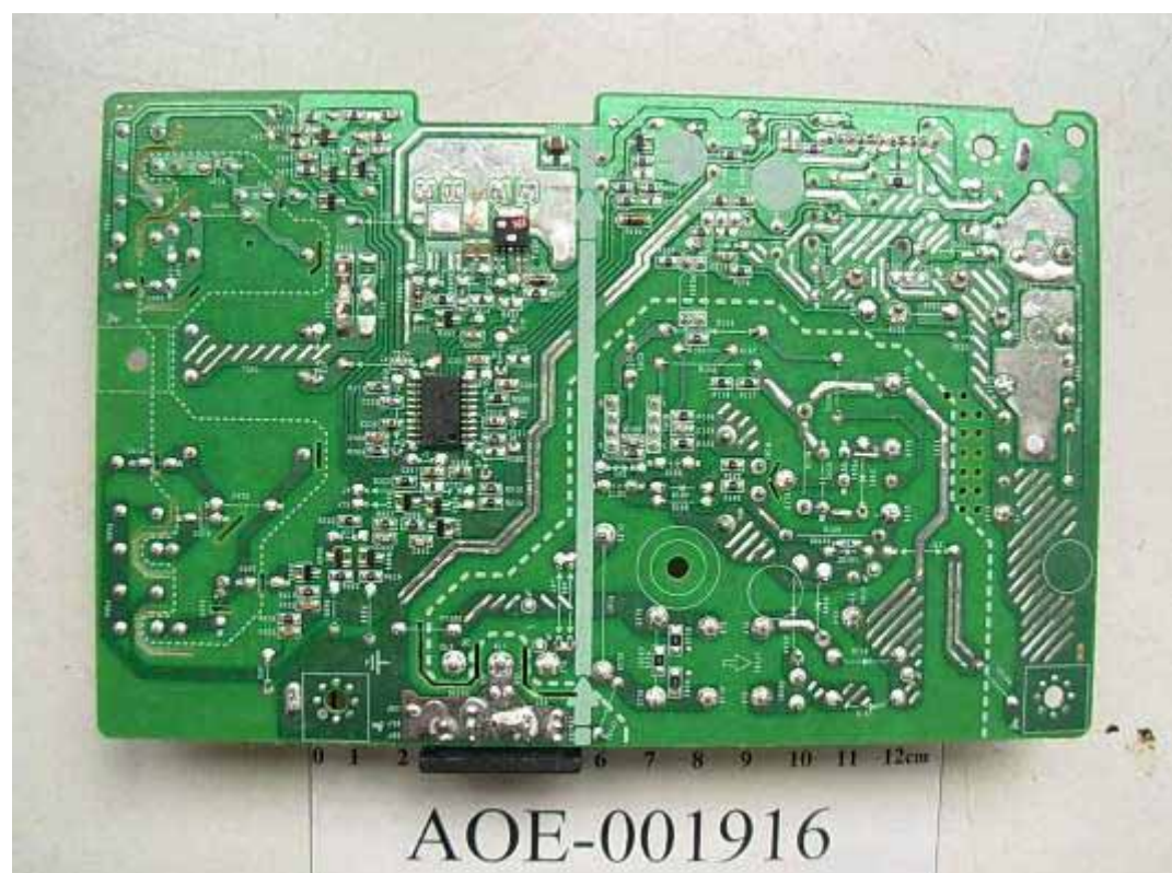
FIGURE 10 LCD MONITOR (M/N: L1942PQT) POWER BOARD (SOLDERED SIDE)
