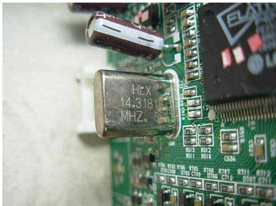
FIGURE 8 LCD MONITOR (M/N: L1942PQT) CRYSTAL ON MAIN BOARD
