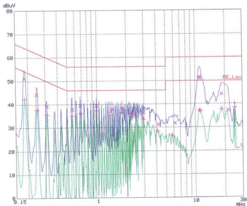
< Neutral line >
