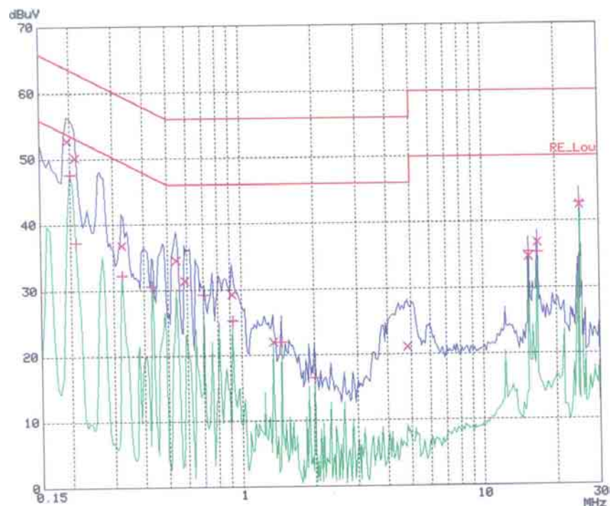
< Neutral line >
