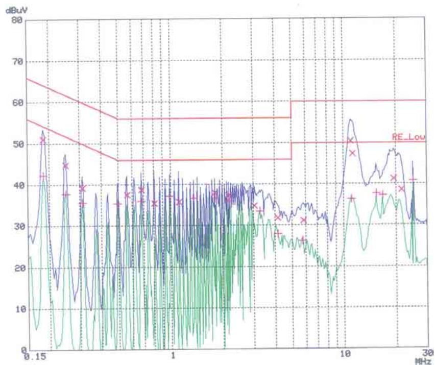
< Neutral line >
