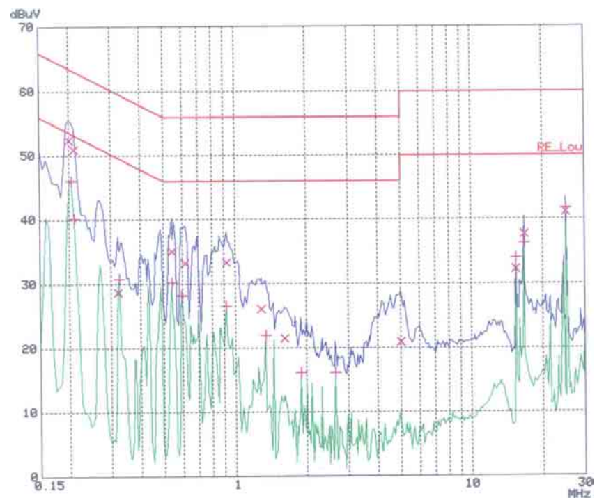
< Neutral line >
