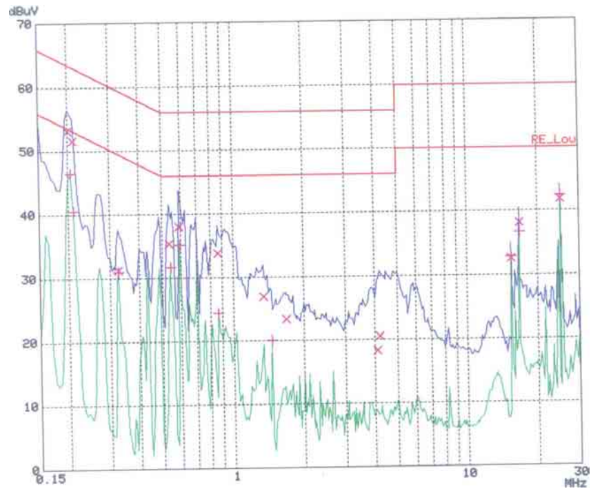
< Hot line >
