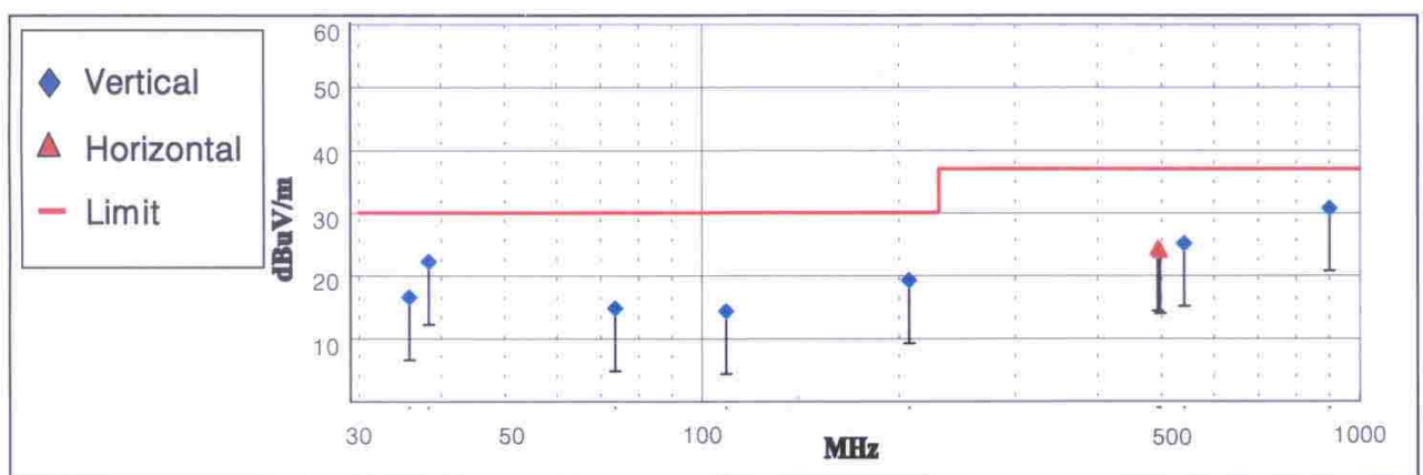
&lt; Fig 6-2. Radiated emission result &gt;
