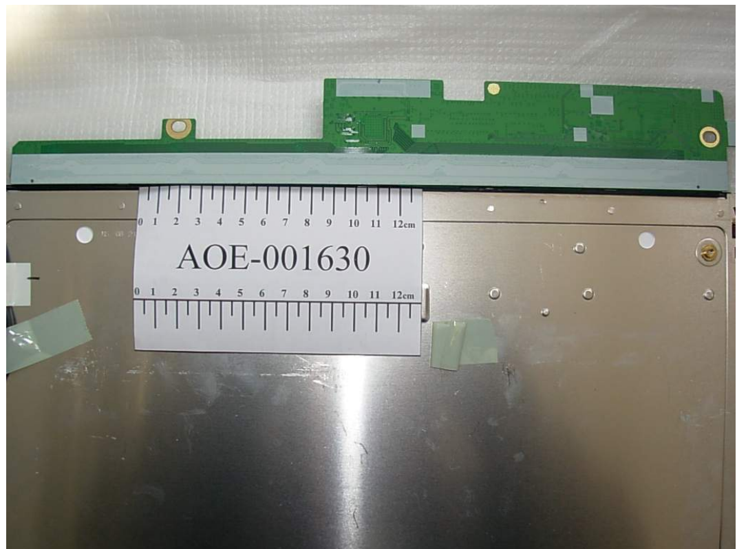
FIGURE 17 LCD MONITOR (M/N: L1755TT) LCD PANEL MAIN BOARD (BACK VIEW)
