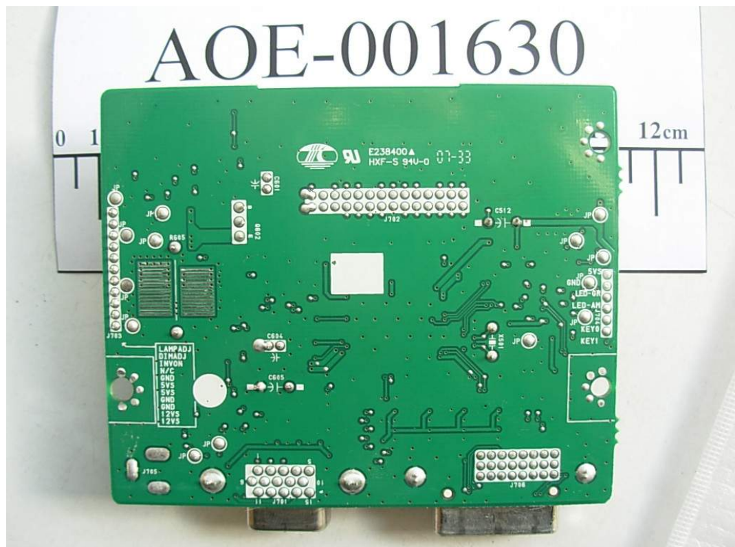
FIGURE 10 LCD MONITOR (M/N: L1755TT) MAIN BOARD (SOLDERED SIDE)
