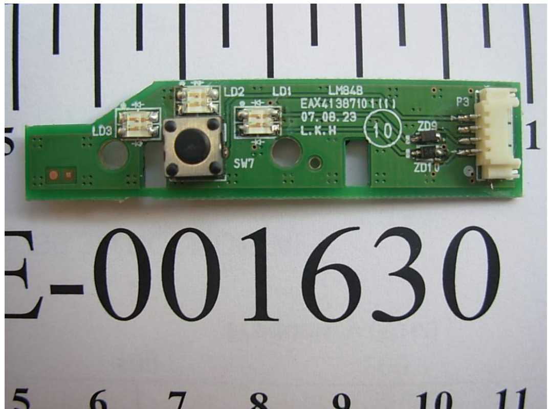
FIGURE 5 LCD MONITOR (M/N: L1755TT) LED BOARD (COMPONENT SIDE)
