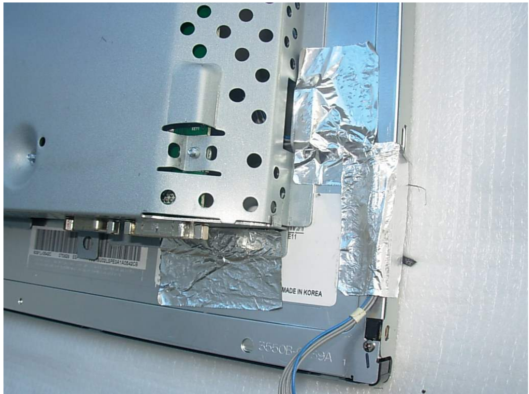
FIGURE 19 LCD MONITOR (M/N: L1755TT) DEBUG 1
