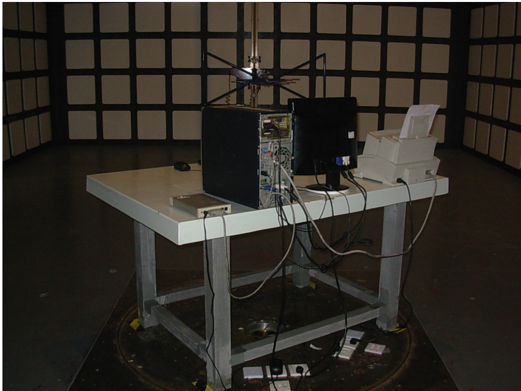
SETUP WITH MAXIMUM DETECTED EMISSION AT HORIZONTAL POLARIZATION (DVI 1280*1024@60Hz, BELOW 1GHz)
