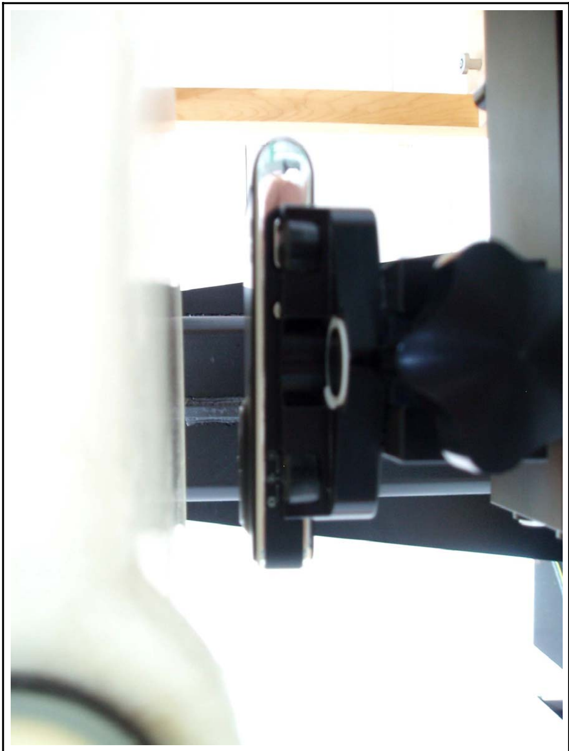
Figure 14 Body SAR Test Setup – w/o Holster
