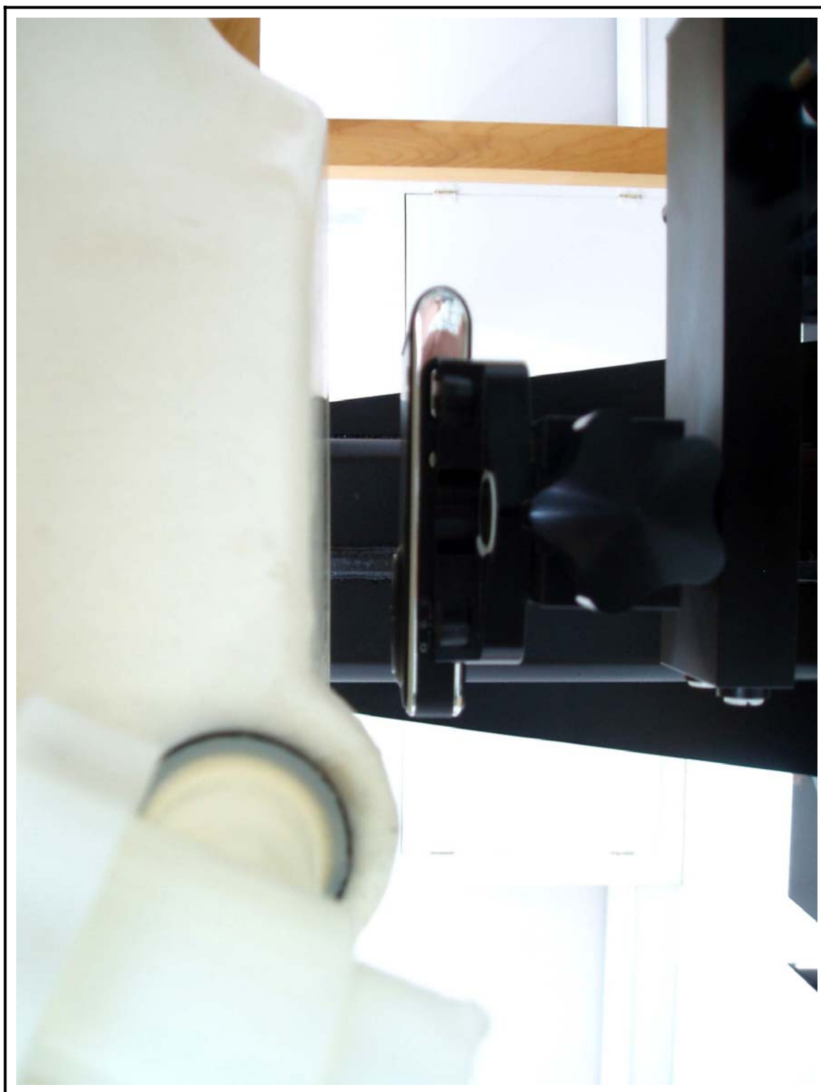
Figure 15 Body SAR Test Setup – w/o Holster
