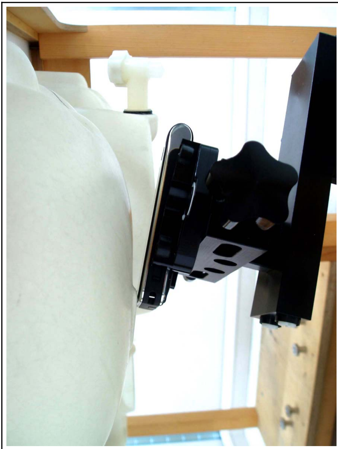
Figure 6 Right Head SAR Test Setup - Ear Tilt Position
