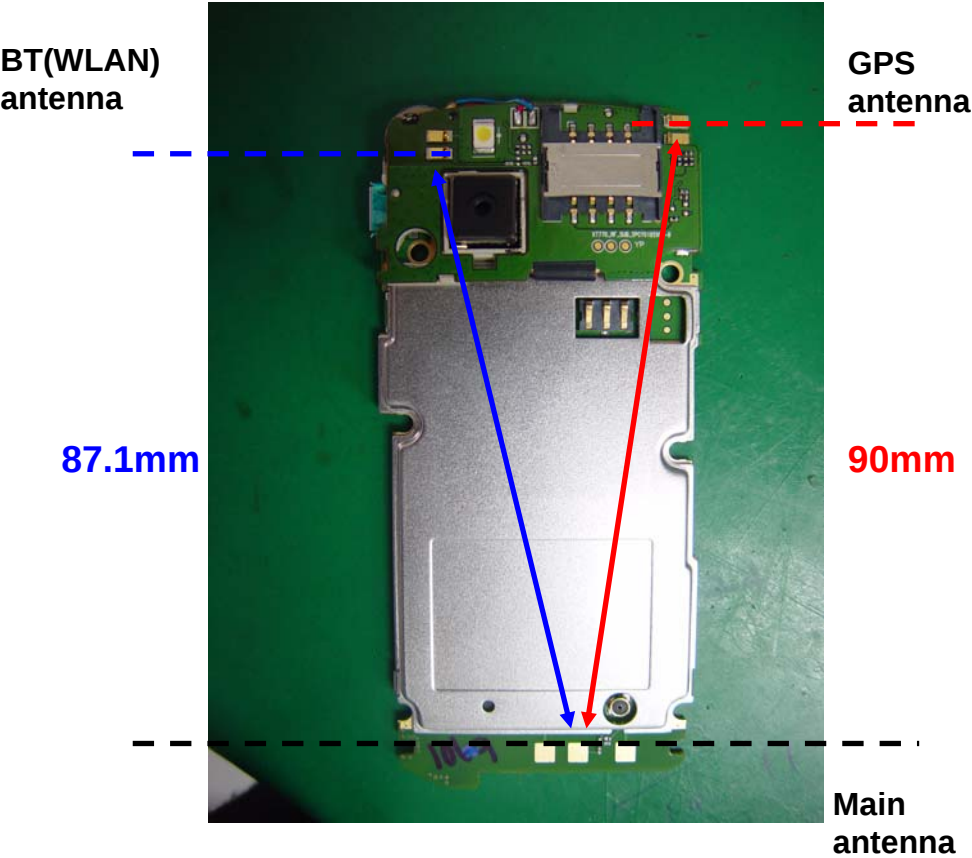
- Feeding distance between antennas -
