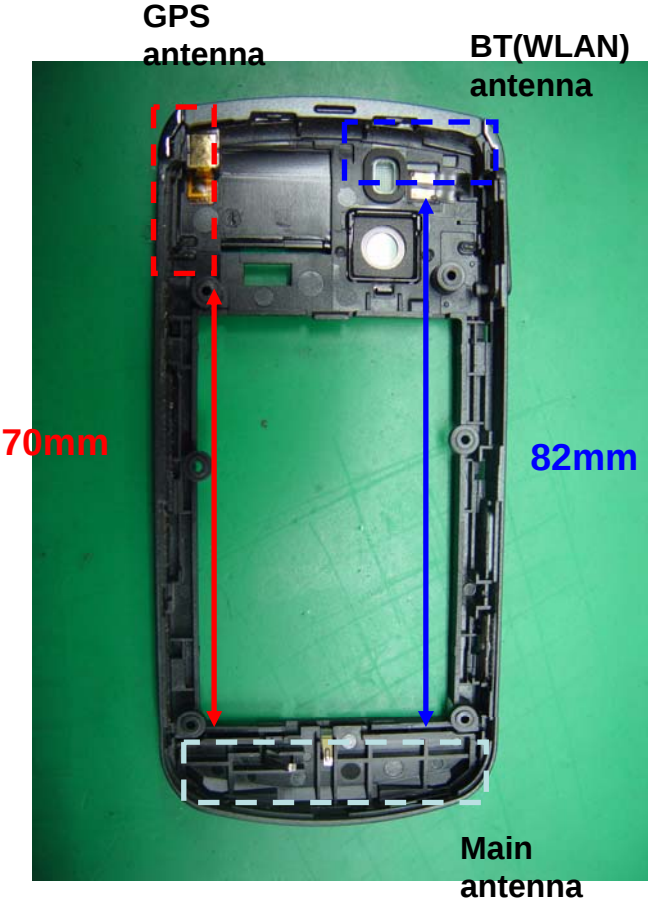
- Pattern distance between antennas -
