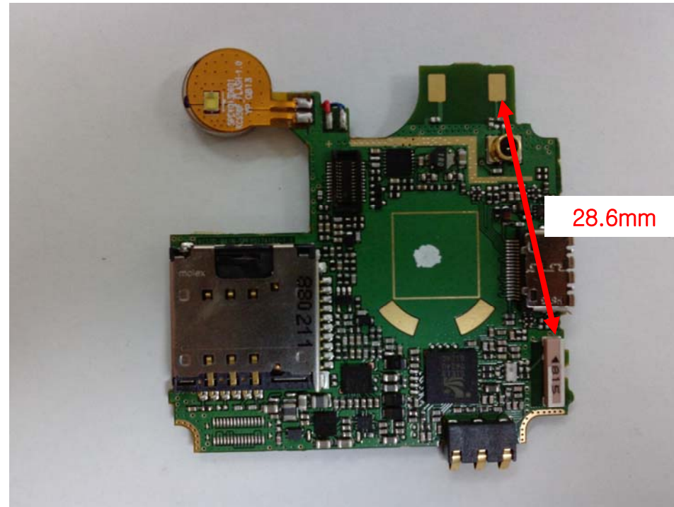
The distance between Main antenna and BT antenna : 28.6mm
